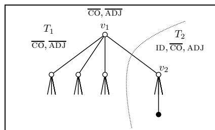
Figure X – Computation of f_{\overline{CO}, \overline{ADJ}}(v_1, T) : 1 case
