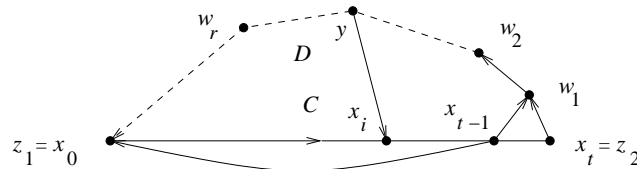
Figure IX – The paths C and D and the path F (in bold).
