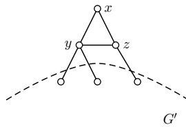
Figure D.XII – Illustration of Lemma D.8.
