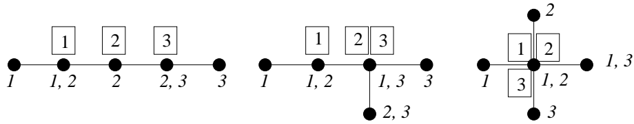
Figure III – the case n=5 in Theorem G.4
