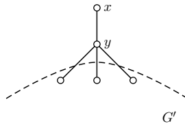
Figure D.XI – Illustration of Lemma D.7.
