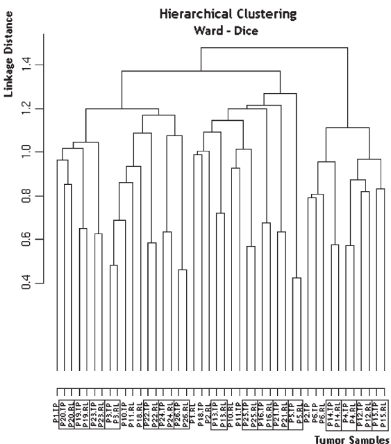
Fig. 3. Dendrogram of hierarchical clustering by breakpoints (Ward-Dice) of 22 available pairs of primary tumors (TP) and their ipsilateral breast cancer (RL). Boxes represent natural pairs with a true recurrence, that is, a pair of tumors from one patient clustered together.
