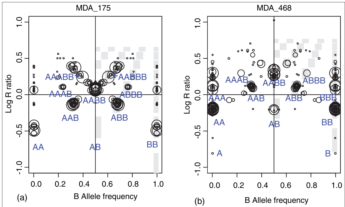
Figure 3 Genome alteration prints (GAPs) for breast cancer cell lines. GAPs for breast cancer cell lines: (a) MDA_175; and (b) MDA_468. Both GAPs show a near-tetraploid pattern, and genotypes were assigned accordingly.
