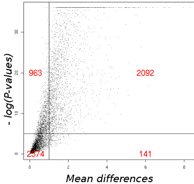
Figure 11.2: Volcano plot: -\log(\text{p-values}) as a function of the mean differences. Only genes with a positive mean difference are considered. It can be seen that 963 genes with a p-value smaller than 10^{-5} are discarded because the mean difference is smaller than 1.
