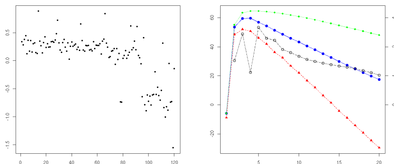
Figure 3: Left panel: Chromosome 10 profile of cell line BT474. The DNA copy number logratio is represented as a function of its position along the chromosome. Right panel: (Left axis) \text{BIC}(m) : \blacktriangle , \text{BIC}(K) : \bullet and \text{ICL}(K) : \blacksquare as a function of the dimension. (Right axis) \mathcal{H}(K) - \mathcal{H}(K-1) : \circ as a function of the dimension.
