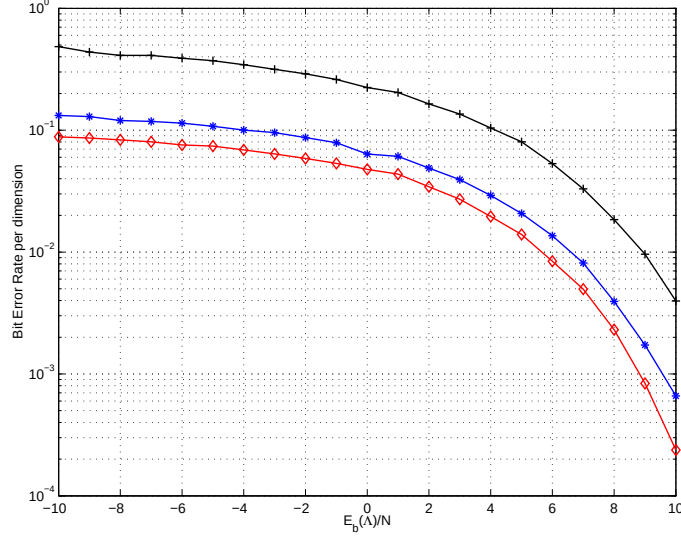
Figure 4.12: Bit Error Probability v.s. the (per-dimension per-bit) Signal-to-Noise Ratio \text{SNR1} = E_b(\Lambda)/N for QIM-embedding the message W_1 . From bottom to top: lattices Checkerboard D_4 , Hexagonal A_2 and Cubic \mathbb{Z} . Bit Error Probabilities (plotted v.s. \text{SNR2} ) corresponding to transmitting W_2 are obtained by shifting these curves to the right according to (4.28).
