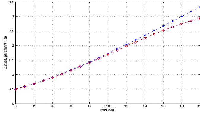
Figure 5.4: Channel capacity loss, in the Gaussian case, due to a weak contaminating perturbation of the two-sided state information. The curves represent the nominal capacity C^{nc}(0) with a perfect knowledge of the two sided state information (Asterisk) and the capacity with imperfect knowledge of two sided state information (Diamond). Perturbation parameters are set to \mathbb{E}[Z^2] = Q_1/100 and \theta = (0.1, 0.1)^T . Capacity loss is independent of the two-sided state information.
