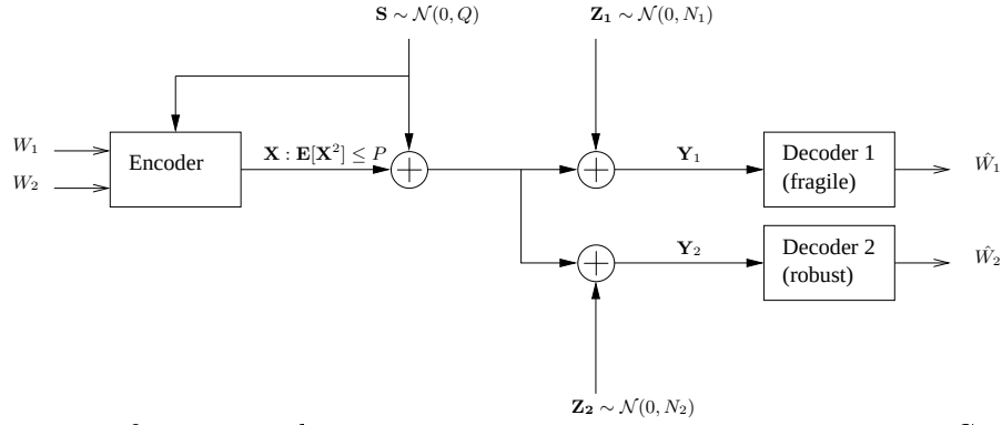
Figure 4.1: Two users information embedding viewed as communication over a two users Gaussian Degraded Broadcast Channel (GDBC).
