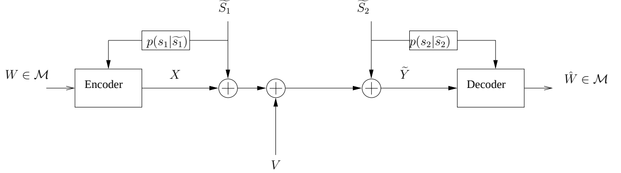
Figure 5.2: Channel with a two-sided state information pair (\tilde{S}_1, \tilde{S}_2) . \tilde{S}_1 is known only partially at the transmitter and \tilde{S}_2 is known only partially at the receiver.
