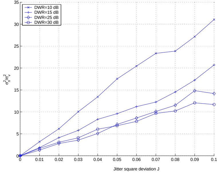
Figure 6.6: Diagram of dependency of the desynchronization noise \sigma_{n_r}^2 on the jitter square deviation J . Dependency on the composite signal \mathbf{c} = \mathbf{s} + \mathbf{x} is illustrated through that on the Document-to-Watermark Ratio DWR: the jitter becomes stronger with strong watermarks (lower DWRs).
