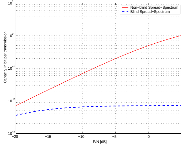
Figure 2.7: Channel capacity, in bit per transmission, for both non-blind and blind Spread Spectrum v.s \text{SNR} = P/N [dB]. The depicted curves are for \text{DWR} = 20 dB. Blind SS suffers great performance loss due the host interference.
