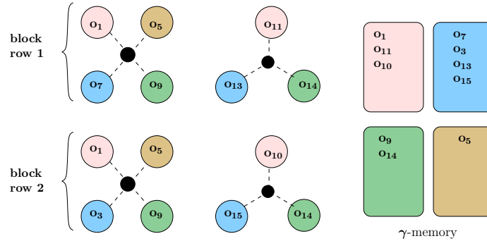
Figure 5.2: Macro-organization by conflict graphs.
