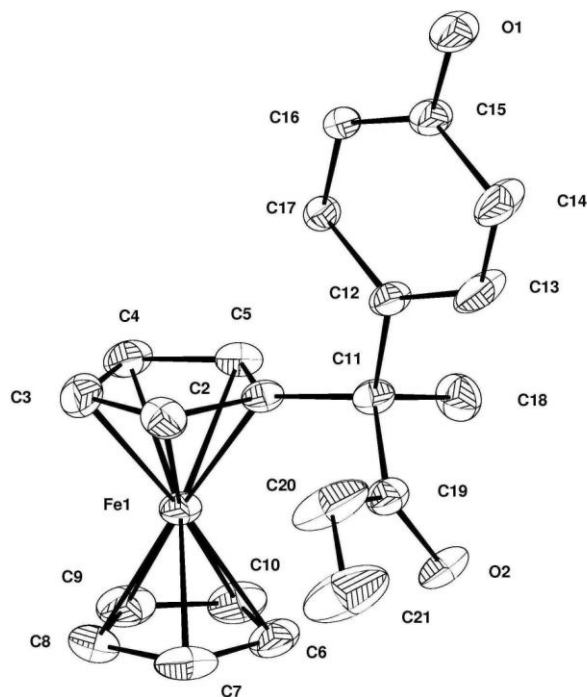
Figure 4.2.2.1. X-ray structure of 20 . Thermal ellipsoids shown at 50% probability level and hydrogen atoms have been omitted for clarity.
