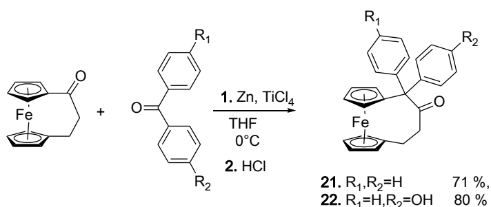
Scheme 5.2.3 McMurry pinacolic rearrangement reaction
