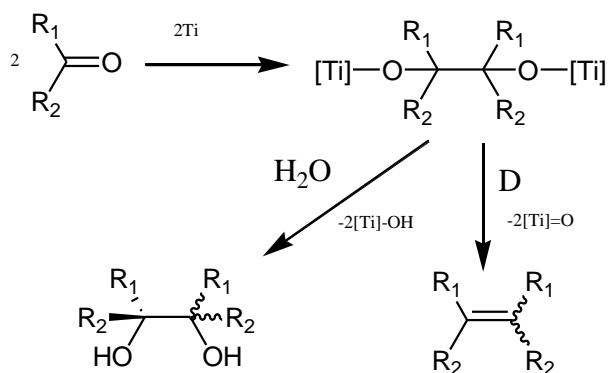
Scheme 4.2 Reductive coupling of ketones via a metalpinacol intermediate
