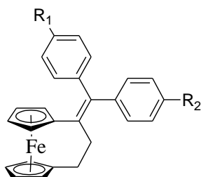
1-[(4-R-phenyl)(4'-R'-phenyl)]methylidene[3]ferrocenophane
