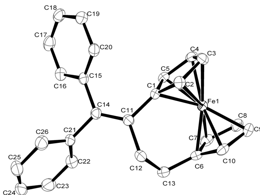
Figure 2.2.2.1 ORTEP diagram of 2a
