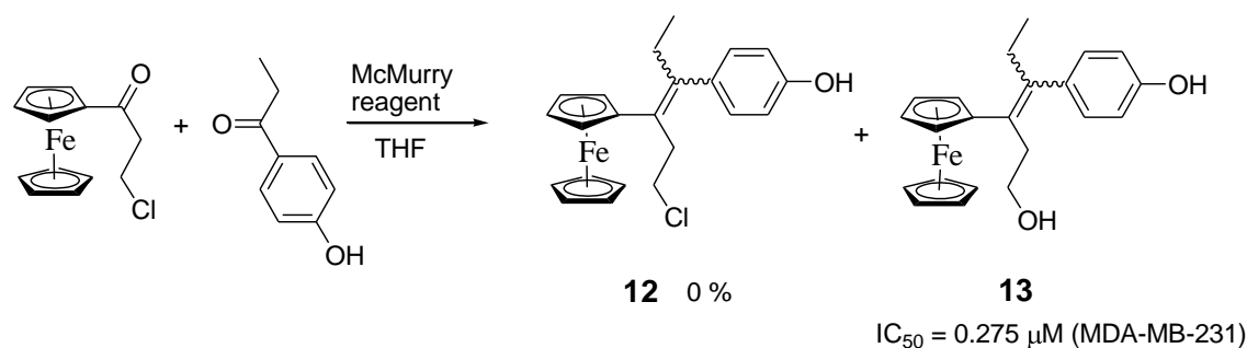
Scheme 4.1.1 Synthesis of 13
