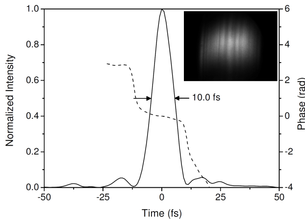
Figure 5.19: Temporal profile after compression at 1.5 atm of Ar and 37 fs input duration. The inset shows the output mode profile.
