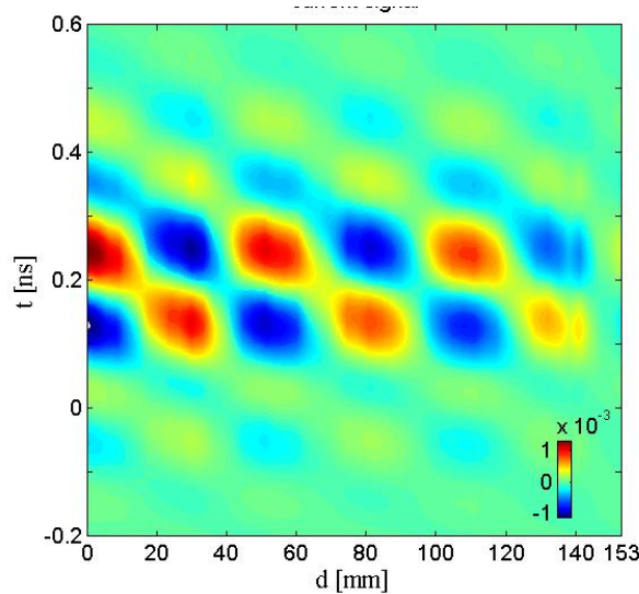
Figure 4.32: The measured current signals in the middle of the plasma column. The laser pulse before the BBO is 40 fs, 1.5 mJ , and linearly polarized. d is the displacement distance.
