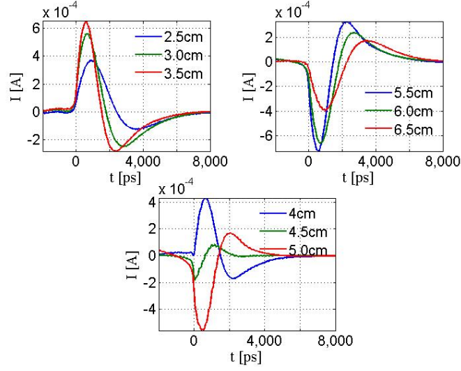
Figure 4.25: The current oscillation at different positions along the plasma channel 0.4 \mu\text{bar} air. The positive and negative value denote that electrons go forward and backward respectively. The laser pulse is 3 mJ, 40 fs, linearly polarized. The focal length is 1 m.
