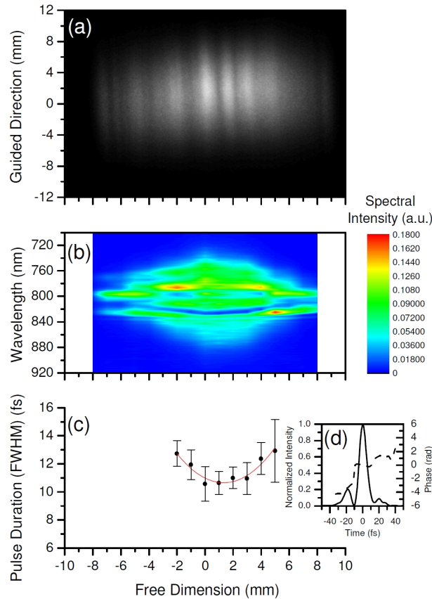
Figure 5.16: Transverse output profile (a), Spectrum (b), and measured pulse duration (c) along the non-guided direction. Typical measured temporal pulse profile in the beam center (d).
