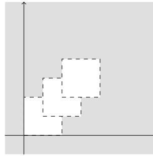
(b) A_1 = [0, 1]^2, A_2 = [0.5, 0.5]^2, A_3 = [1, 2]^2
