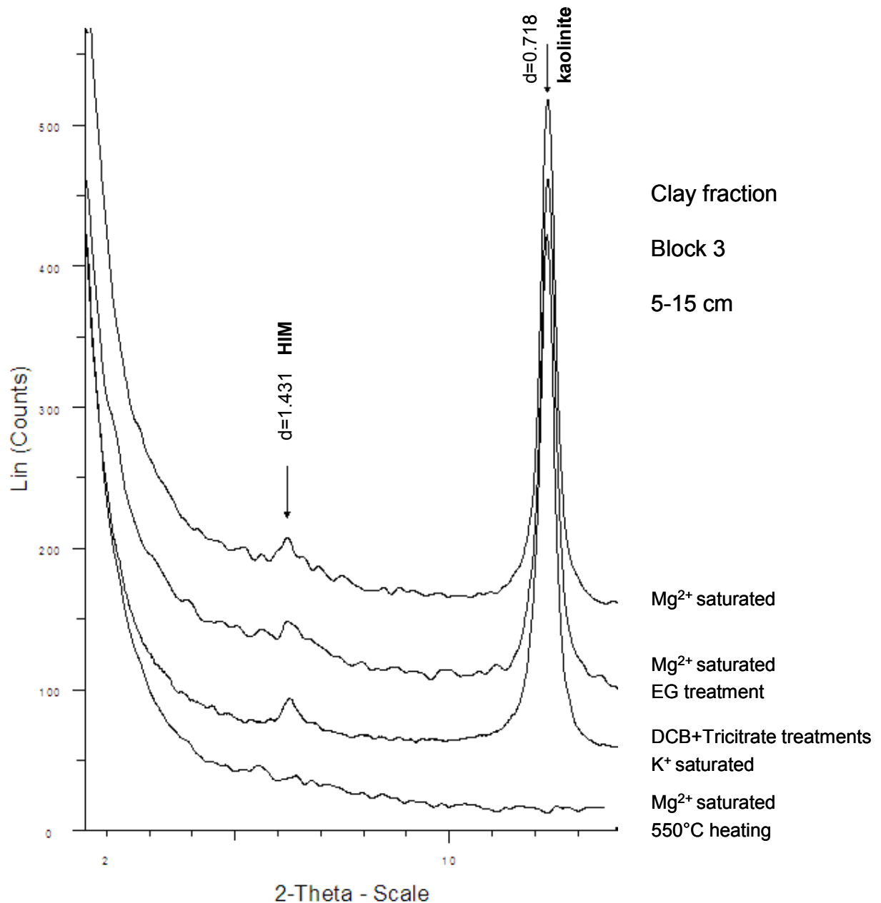
Figure 25 Identification of the peak at 1.431 nm: influence of treatments ( Mg^{2+} saturation, ethylene glycol (EG) treatment, DCB followed by tricitrate extractions and saturation by K^+ , heating at 550°C) on RX diffractograms performed on oriented deposits of the clay fraction for layer 5-15 cm block 3 of data set SOIL AP11 .
