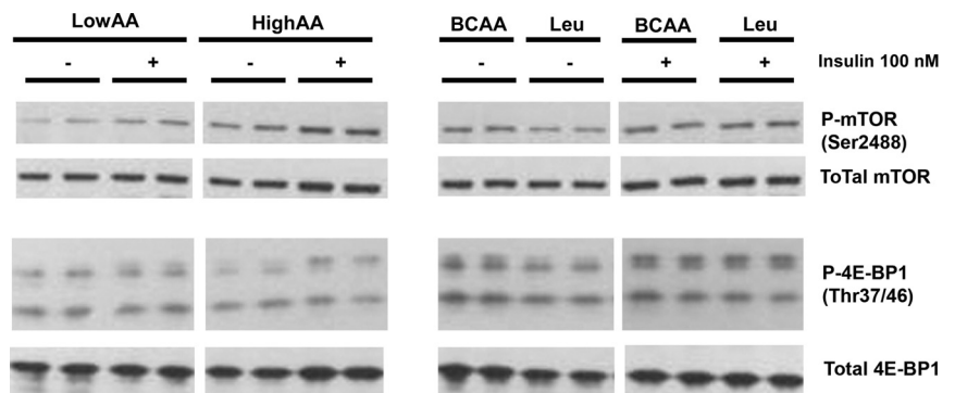
Fig. 5. Effect of branched chain amino acids (BCAA), leucine (Leu), and insulin on mTOR and 4E-BP1 phosphorylation in a primary hepatocyte culture. Hepatocytes were incubated for 60 min in M199 salt medium containing 5 mM glucose supplemented with AA at low or high AA concentrations with or without insulin. To study the effect of BCAA and Leu, the medium containing low AA was supplemented with BCAA or Leu at the same level as high AA. Protein extracts were processed for Western blot analyses, as described in the MATERIALS AND METHODS. Results are representative of at least 2 separate experiments.
