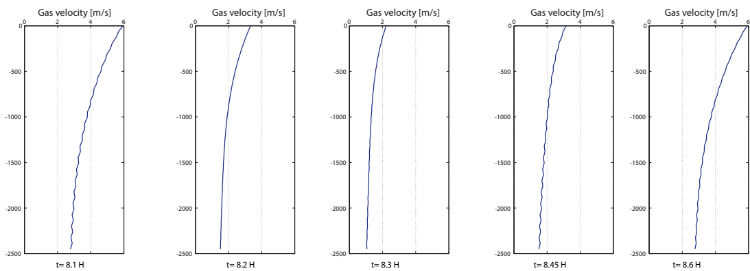
(b) Gas velocity profiles
