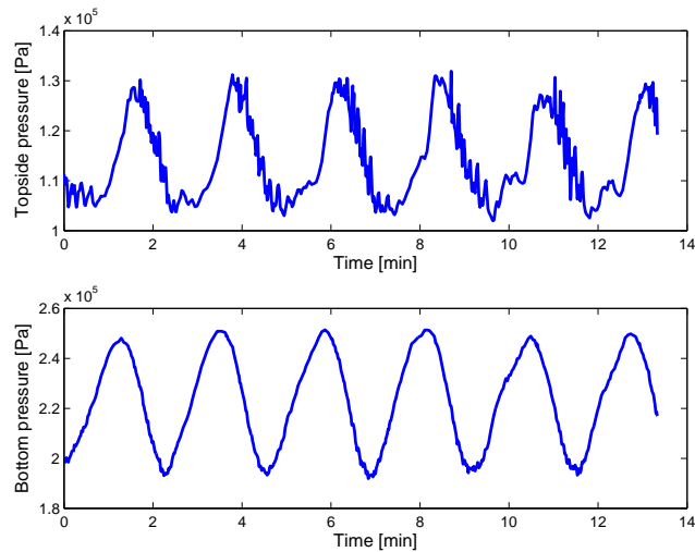
(b) Open-loop oscillations of the topside and bottom pressures
