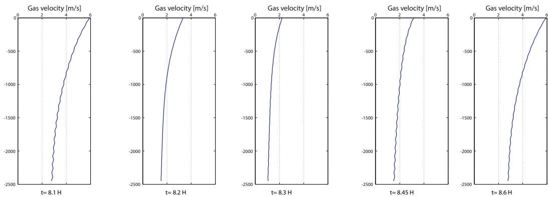
(b) Gas velocity profiles
