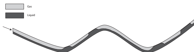
Figure 1.5: Schematic view of a flowline subject to terrain slugging. The accumulation of liquid at the low points blocks the flow of gas at these locations, which causes a build up of pressure. When the pressure is high enough, the liquid is pushed downstream, before another slug is formed.
