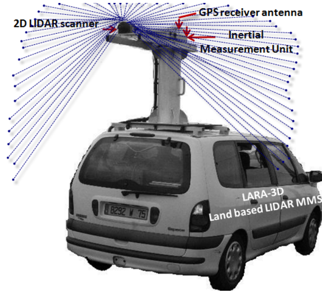
Figure 3.1: LARA-3D prototype mobile mapping platform - present configuration
