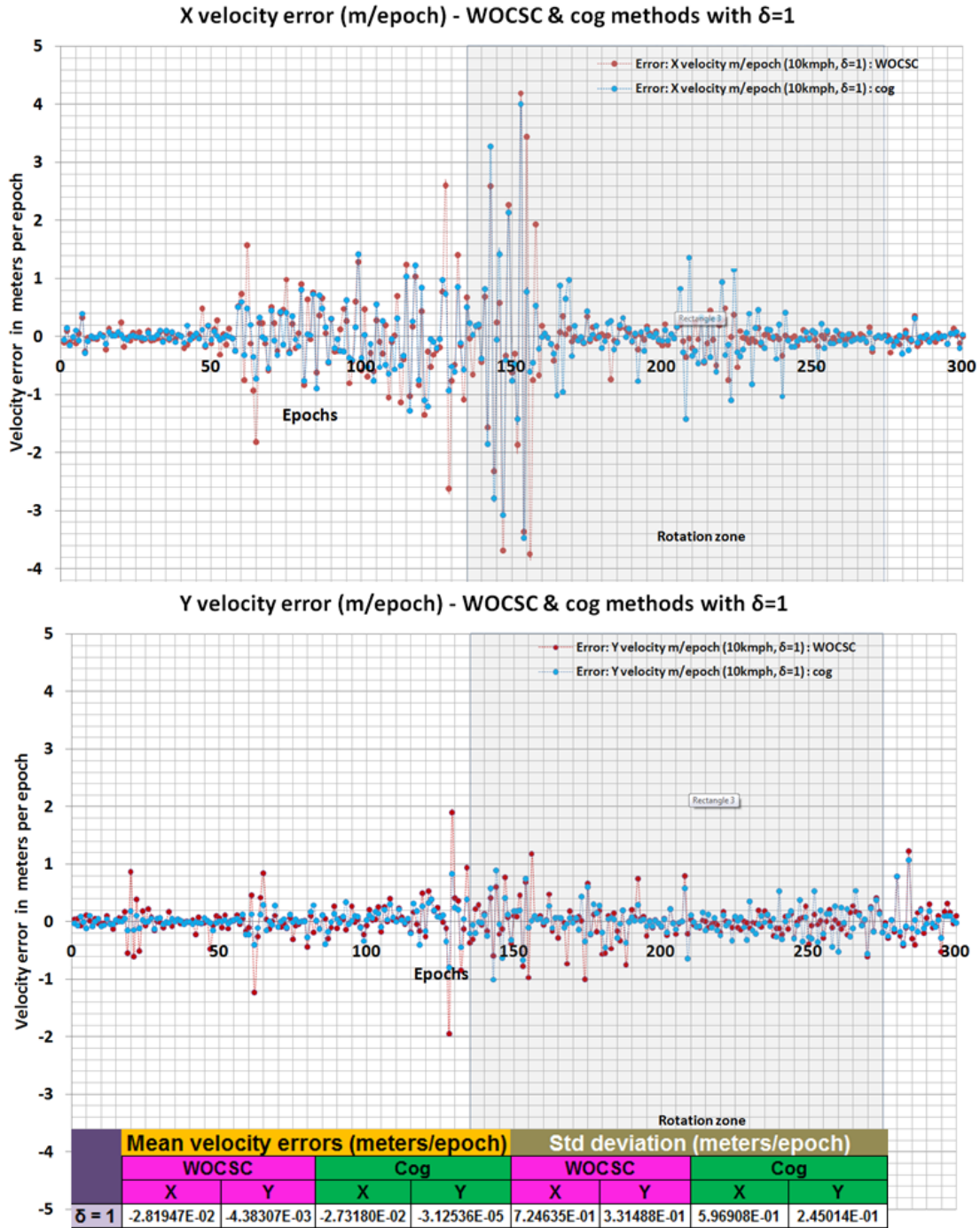
Figure 7.14: 2DOF (X and Y) translation errors for the estimated trajectory (refer to figure 7.12), for a vehicle driven at \sim 10 kmph. The error statistics (refer to the table in this figure) for two alternative methods to compute translation: WOCSC without SDA and cog with SDA, are comparable. This demonstrates that in the absence of association outliers both the methods function equivalently. In each plot, the epochs corresponding to the rotation in the trajectory is highlighted.
