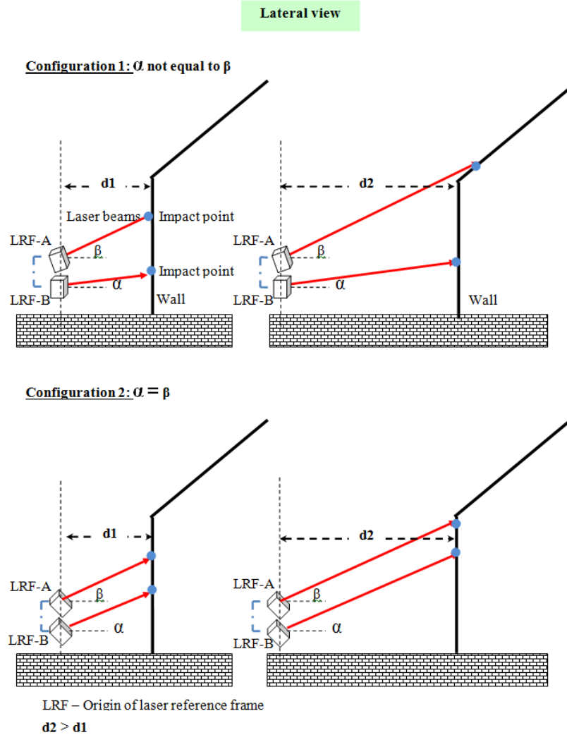
Figure 5.2: Two configurations of a laser scanner pair used to extract planar features. (Top) Non isoclinical beams result in a divergence effect and a dependence of the distance to the analyzed object. (Bottom) Isoclinical lasers lead to a higher probability of detecting the planar features independent of the distance. The impact locations of the laser scans on the wall are represented by blue points.
