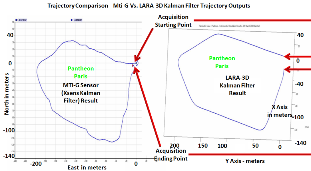
(c) Obtained results - MTi-G and LARA-3D trajectory outputs
