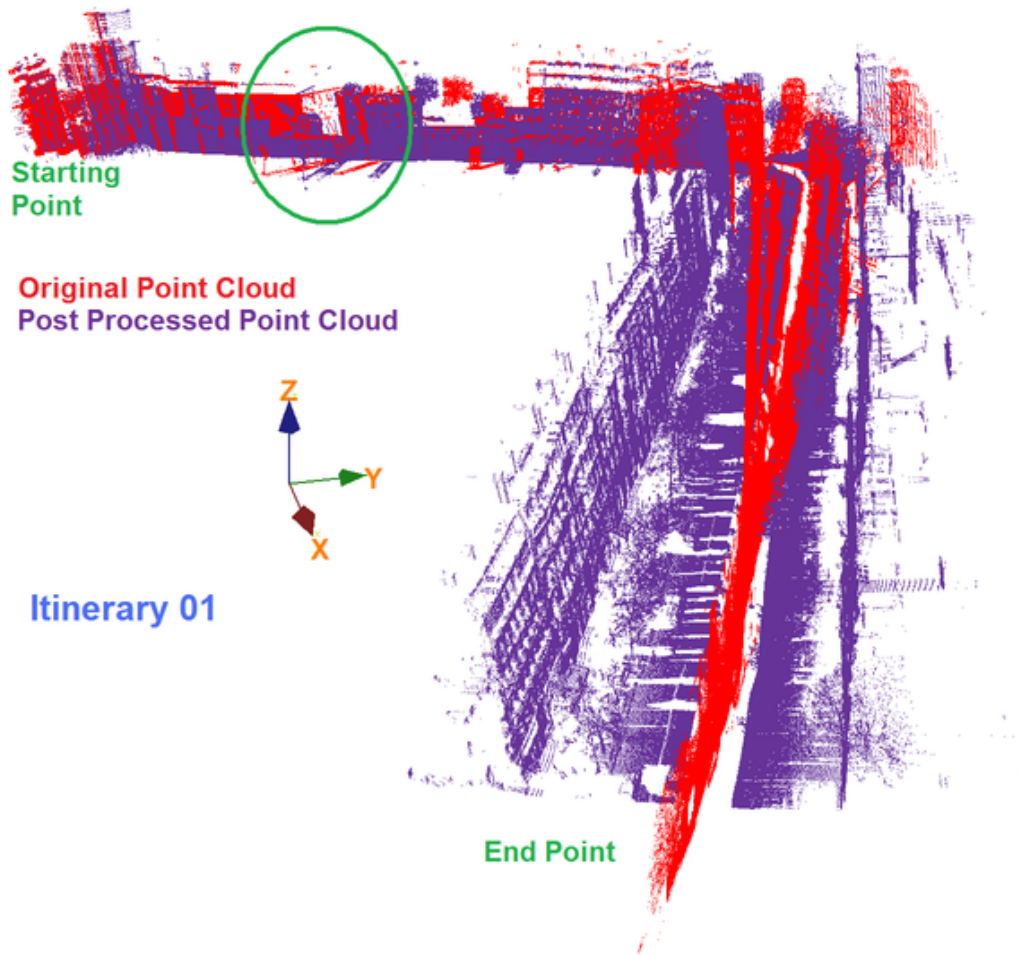
Figure 3.22: Heading drift and discontinuities corrected 3D point cloud after applying post-mission processing for Itinerary 01.
