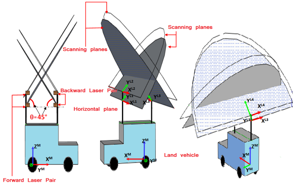
Figure 5.1: The laser scanner configuration used in our approach. Two isoclinal pairs of laser scanners are mounted on a vehicle with an angle \theta , with respect to the horizontal plane.
