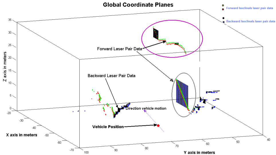
(a) Extracted planar patches - simulated data from SIVIC
