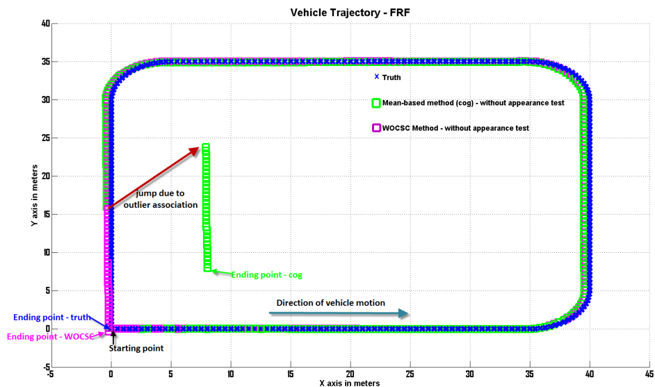
(b) Trajectories computed using cog and WOCSC translation methods
