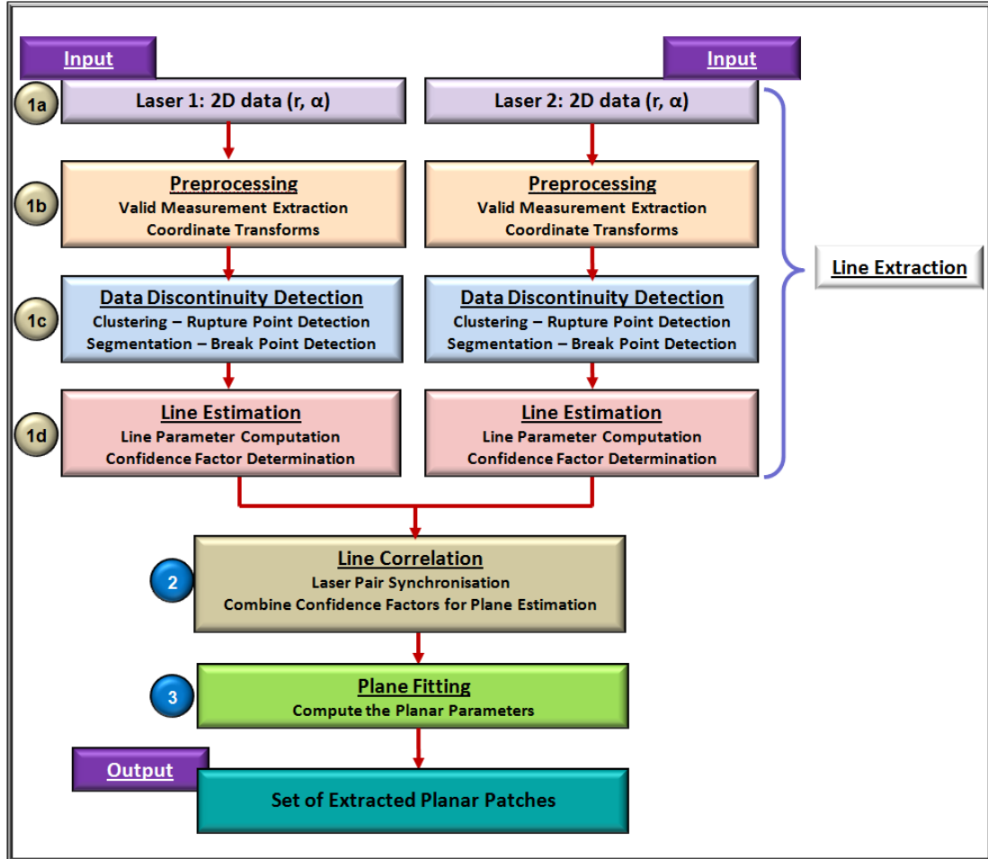
Figure 5.4: Planar landmark extraction process using the measurements of an isoclinical pair of 2D laser scanners.
