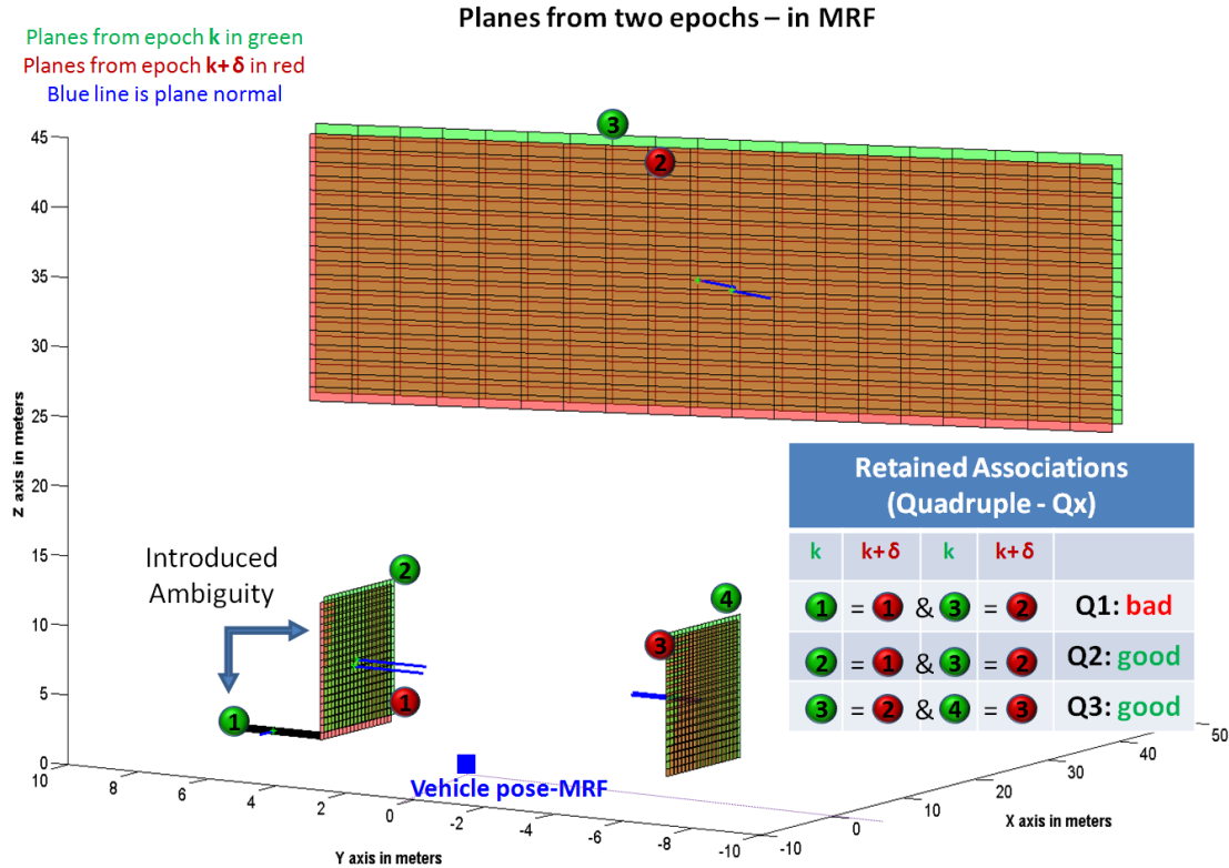
(a) Planes observed at epochs 262 and 263, and their retained associations
