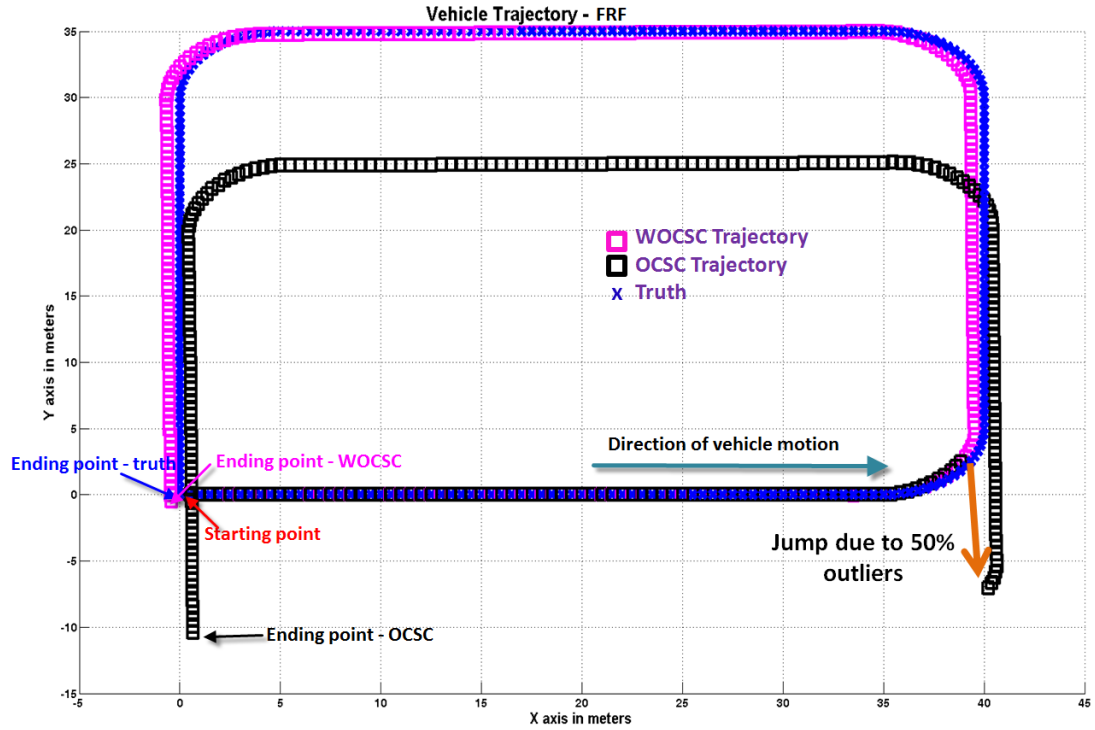
Figure 7.9: Generated trajectory comparison between OCSC and WOCSC methods, showing that WOCSC can handle 50% or more outliers. The scenario where OCSC fails is shown in figure 7.8. At epoch k + \delta = 83 , OCSC converges to an inaccurate optimal translation, resulting in a jump, and WOCSC overcomes this situation by using the confidence indicators CPEF .
