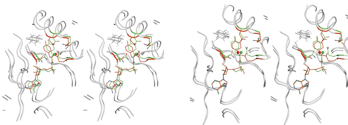
(a) TyrRS:L-TyrAMP
