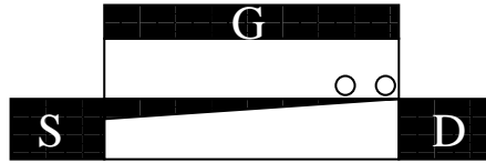
Figure 2.1: Interface traps in MOS structure under HCI degradation: illustration.
