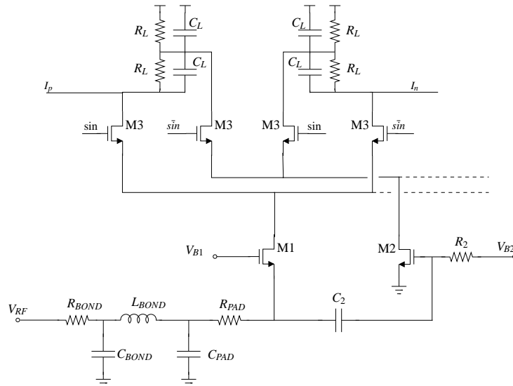
Figure 4.1: The BLIXER topology composed of a balun, a wide-band low noise amplifier (WBLNA), and a mixer connected: illustration of the I-path (the Q-path is not present as it is similar to the I-path) [2].
