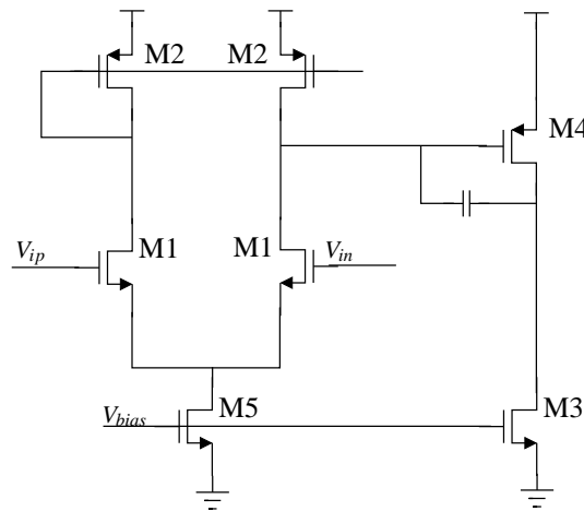
Figure 4.15: Basic operational amplifier: illustration.
