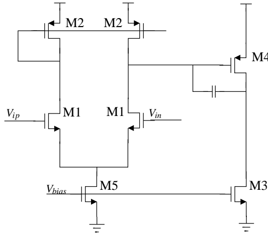
Figure 4.15: Basic operational amplifier: illustration.
