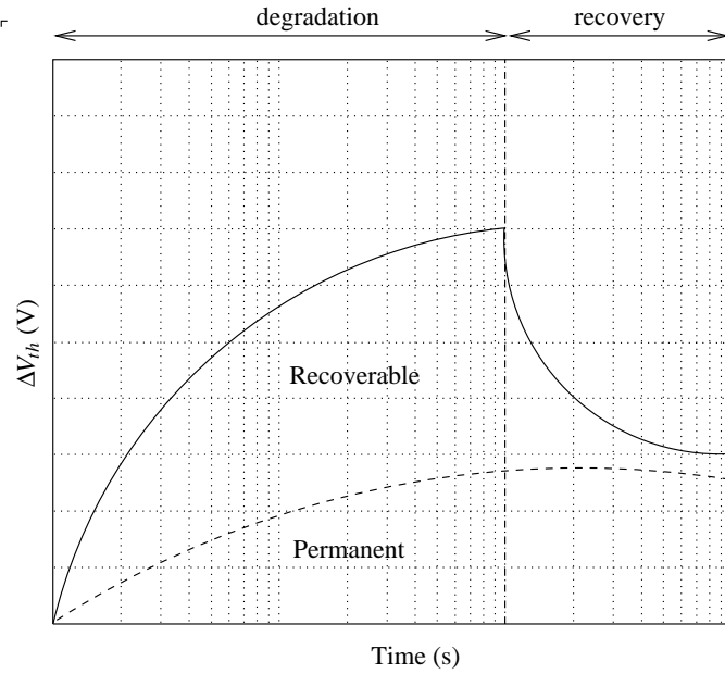
Figure 3.4: Behavior monitor of the NBTI permanent and recoverable damage: illustration [81].
