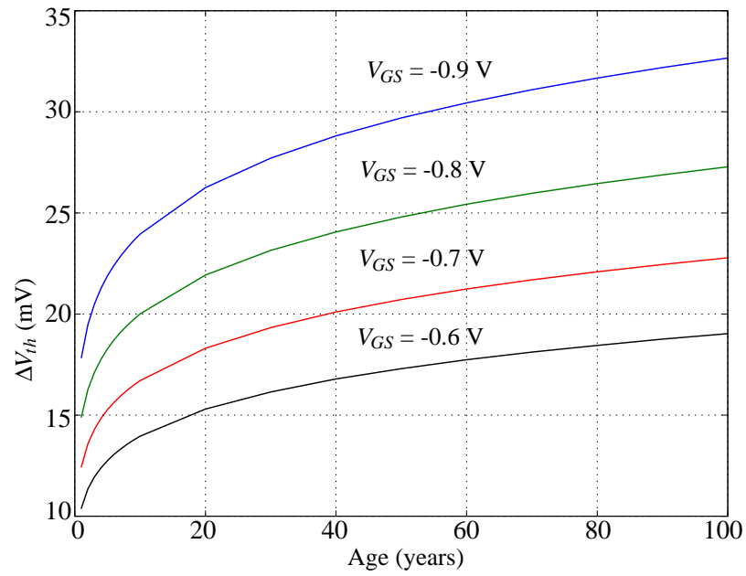
Figure 6.6: \Delta V_{th} degradation for the PMOS DCO transistors stressed by NBTI at 150 °C.
