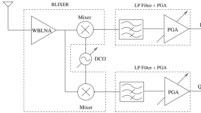
Figure 1.2: RF front-end architecture for multi-standard wireless applications: illustration [5].
