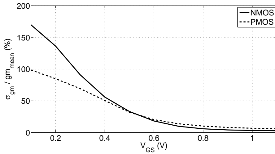
Figure 6.8: The percentage of \sigma_{gm}/gm for the NMOS (in solid line) and the PMOS (in dashed line).
