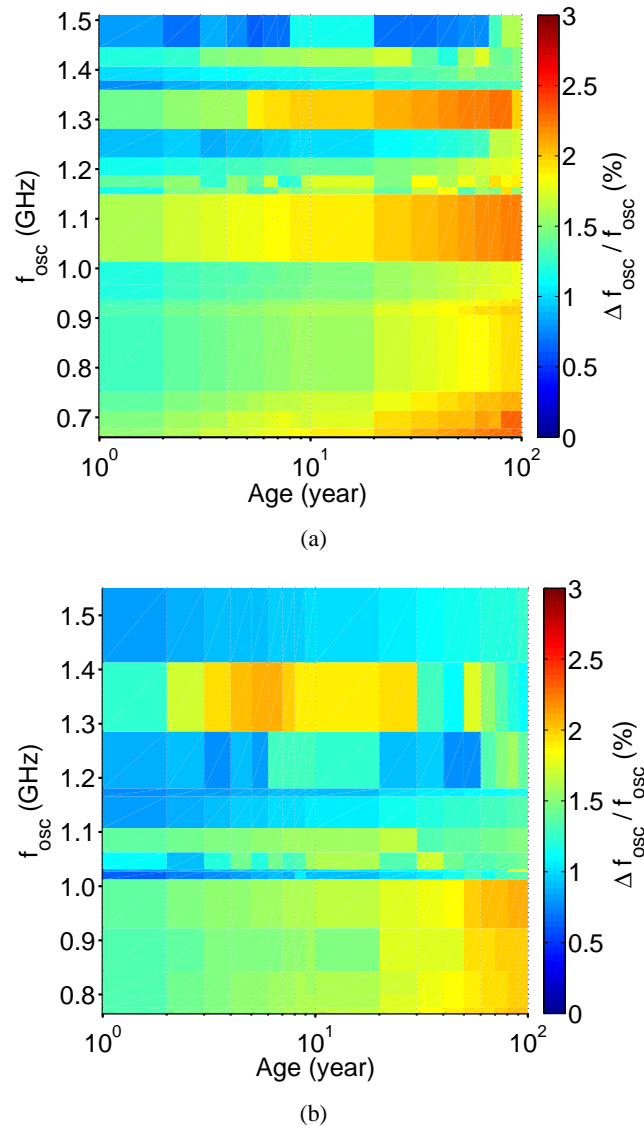
Figure 4.9: The \Delta f_{osc}/f_{osc} degradation at 27 °C for (a) the classical and (b) the reliable designed DCO.
