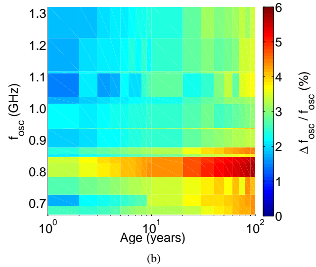
Figure 4.10: The \Delta f_{osc}/f_{osc} degradation at 150^{\circ}\text{C} for (a) the classical and (b) the reliable designed DCO.
