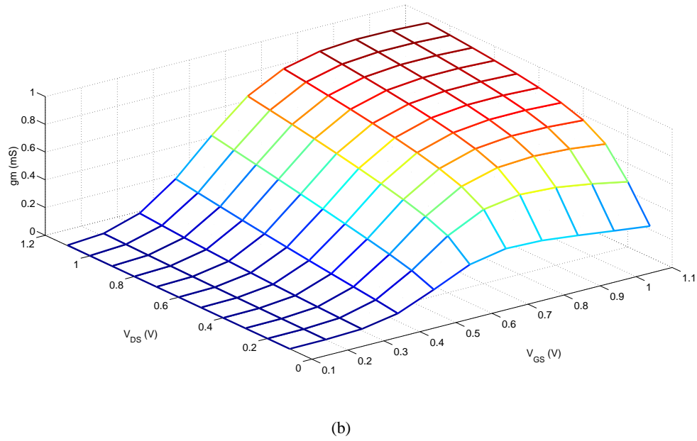
Figure 6.2: The technology simulated-characterization for normalized NMOS ( W = 1 \mu\text{m} and L = 60 \text{ nm} ) biased from 0.1 V to 1.1 V for the I_{DS} (a) and the gm (b).
