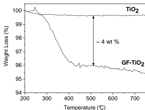
Figure 89 – TGA of pristine and PHEMA grafted (GF-TiO 2 ) TiO 2 nanoparticles (85/15 anatase/rutile).
