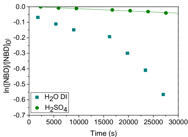
Figure 9 – Plots of \ln([\text{NBDT}]/[\text{NBDT}]_0) versus time in \text{H}_2\text{O DI} and \text{H}_2\text{SO}_4 with [\text{NBDT}]_0 = 10^{-4} \text{ M}
