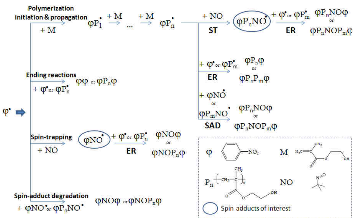
Scheme 65 – Representation of all the reactions identified as likely to occur during the Grafftast™ reaction (with NBDT, a reducing agent and HEMA) in presence of a MNP spin-trap. ER is an abbreviation for ending reactions, ST for spin-trapping and SAD for spin-adduct degradation.
