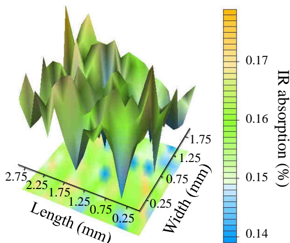
Figure 41 – IRRAS mapping ( 6\text{ mm}^2 ) of the \nu_{\text{NO}_2}^s band ( 1350\text{ cm}^{-1} ) from a typical PNP layer grafted by redox activation in \text{H}_2\text{O DI} .
