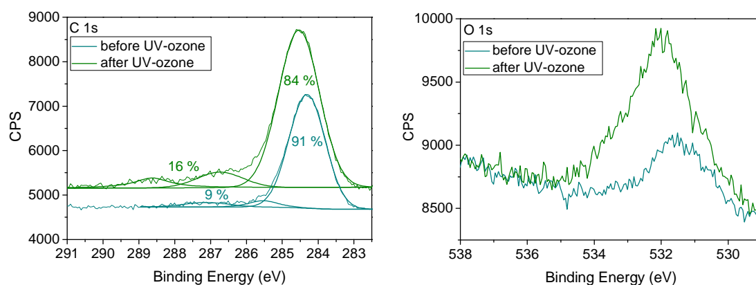
Figure 22 – C1s and O1s XPS spectra of a pristine gold substrate before and after a 10 min UV-ozone cleaning procedure.
