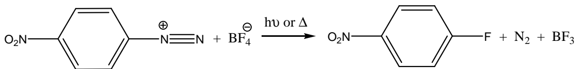
Scheme 37 – Formation of fluoroaryls by the Schiemann reaction.
