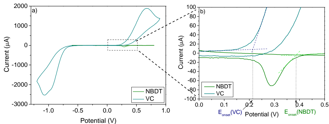
Figure 13 – Overlay cyclic voltammograms (0.1 V/s scan rate, SCE, working electrode = gold plate) of ascorbic acid ( C = 3 \cdot 10^{-2} M) and 4-nitrobenzene diazonium salt ( C = 5 \cdot 10^{-3} M) in HCl solutions (pH = 2) a) in full scale and b) zoomed in the area of interest.
