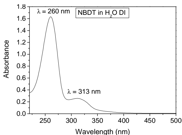
Figure 5 – Typical UV spectrum of NBDT in water.
