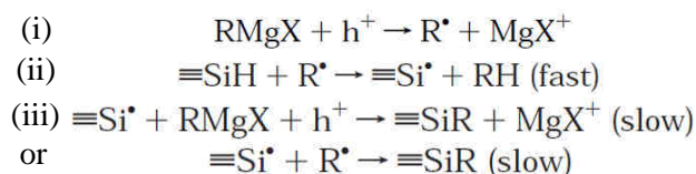
Scheme 6 – Oxidative electrografting of alkyl Grignard reagents on Si extracted from Etcheberry and coworkers' work 20 , (h + = hole).
