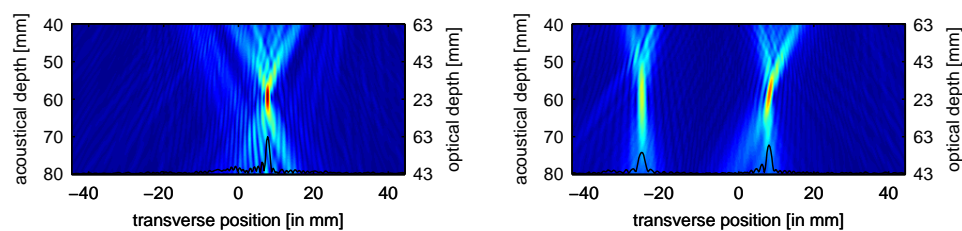
(e) Simulation of the intensity of the HIFU field when guided by the isolated photoacoustic signals of the target. (f) Simulation of the intensity of the HIFU field when guided by all photoacoustic signals originating from the depth of the target. Note: all scales are identical to those of Figure 6.17e.
