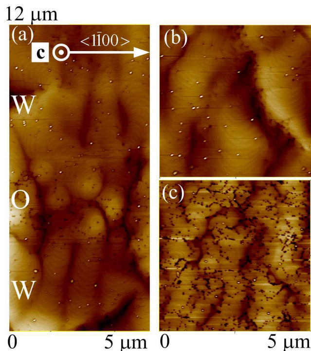
Figure 23. AFM images of blue MQWs on (a) LEO GaN (5 μm x 12 μm), (b) wing area of LEO GaN (5 μm x 5 μm), (c) conventional GaN (5 μm x 5 μm). ‘W’, and ‘O’ corresponds to the wing and opening regions, respectively.
