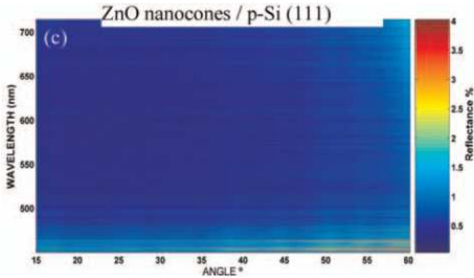
Figure 4 RT reflection of the ZnO nanostructures normalized to the reflection of the silicon reference. (b) ZnO nanocones/ n-Si (111) and (c) ZnO nanocones/p-Si (111).
