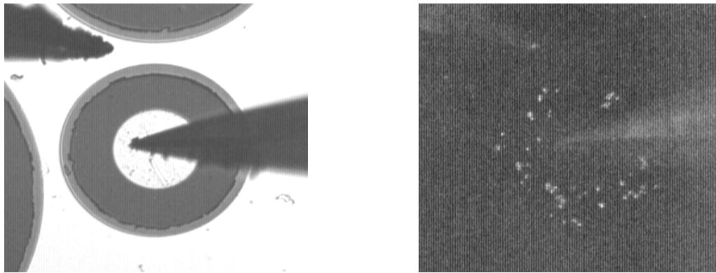
Figure 19: (a) Image of the mesa while being probed for electrical characterization. (b) Image of the mesa operated under DC bias with a current injection of approximately 100 mA demonstrating electroluminescence from discrete spots within the mesa area.
