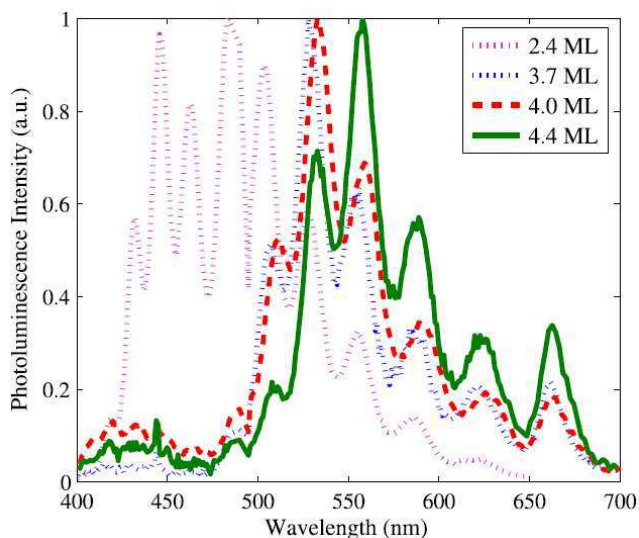
Figure 51. Normalized photoluminescence intensity versus wavelength at room temperature for 2.4-, 3.7-, 4.0-, and 4.4-ML-thick InGaN.
