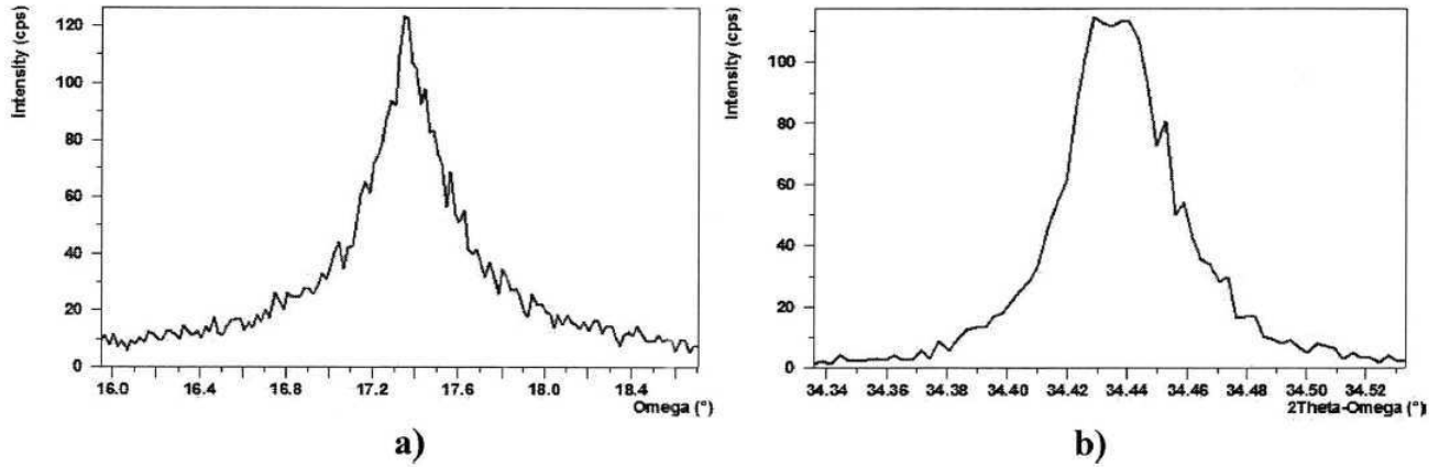
FIG. 9. a) Omega scans and b) two theta omega scans for ZnO nanostructures grown by PVT on c\text{-Al}_2\text{O}_3 .
