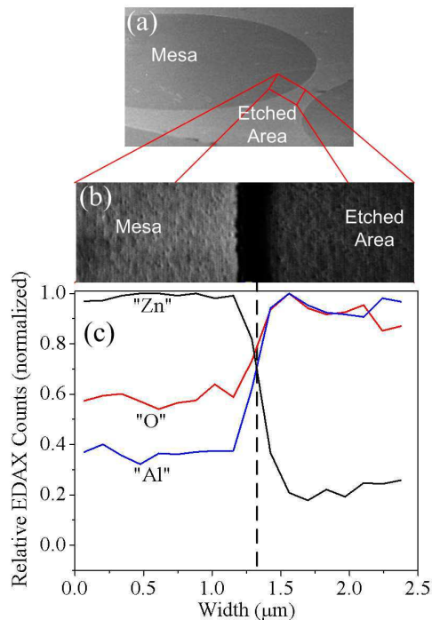
Figure 44. (a) Dry etching of n -ZnO on sapphire, (b,c) EDX system analysis shows the relative concentrations of O, Al and Zn atoms through 2.46 µm (from mesa through etched area). The EDX scale is normalized and relative.
