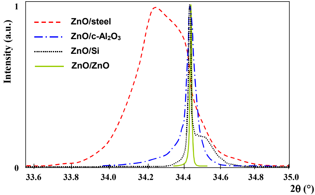
Figure 3. Normalised XRD 2\theta/\omega scans (linear intensity scale) for the (0002) peaks of the nanostructured ZnO grown on various substrates.
