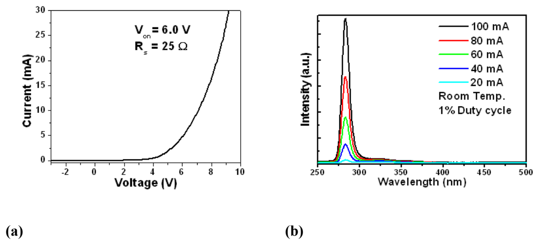
Figure 4: (a) IV curve and (b) EL spectra of high-power 280 nm LED.
