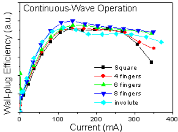
Figure 11: Wall-plug Efficiency under continuous-wave operation for the 300µm x 300 µm square mesa, the four-, six- and eight-finger mesas, and the involute geometry mesa.
