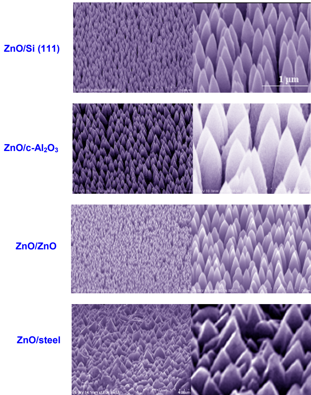
Figure 1: SEM images of ZnO nanostructures grown by PLD on (a) Si (111), (b) c-Al 2 O 3 , (c) ZnO and (d) high manganese austenitic steel. The images on the right are zooms of the images on the left. The scales for the images on the right are similar for all substrates.
