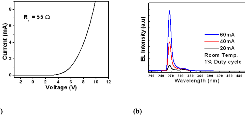
Figure 7: (a) IV curve of a single 265 nm LED and (b) EL spectra at various currents showing a dominant peak at 265 nm [Error! Bookmark not defined.].
