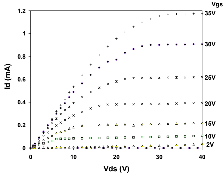
Figure 5: Output characteristic of an ZnO/Si 3 N 4 /SiO 2 /Si (111) TFT with L = 150μm & W = 700μm.
