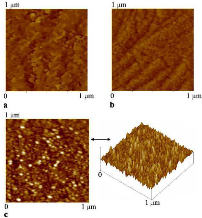
Figure 47. AFM ( 1\ \mu\text{m} \times 1\ \mu\text{m} ) images of 5.8 ML InGaN grown at (a) T = 734^\circ\text{C} , (b) T = 679^\circ\text{C} , and (c) T = 633^\circ\text{C} .
