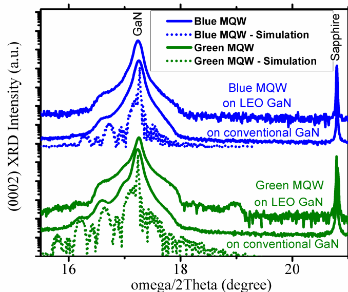
Figure 22. (0002) XRD omega/2Theta scan of blue and green MQWs on conventional and LEO GaN. The XRD simulation is realized to compare with experimental results.
