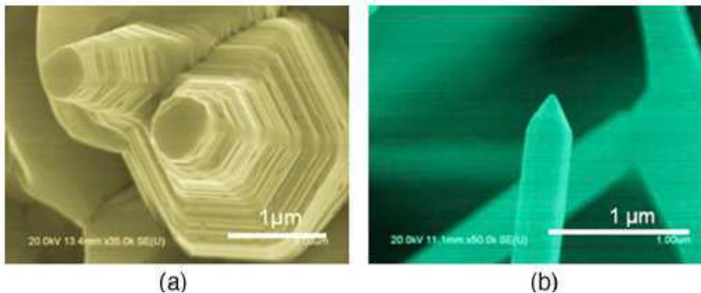
FIG. 4. SEM images of ZnO nanostructures on c\text{-Al}_2\text{O}_3 grown by PVT.
