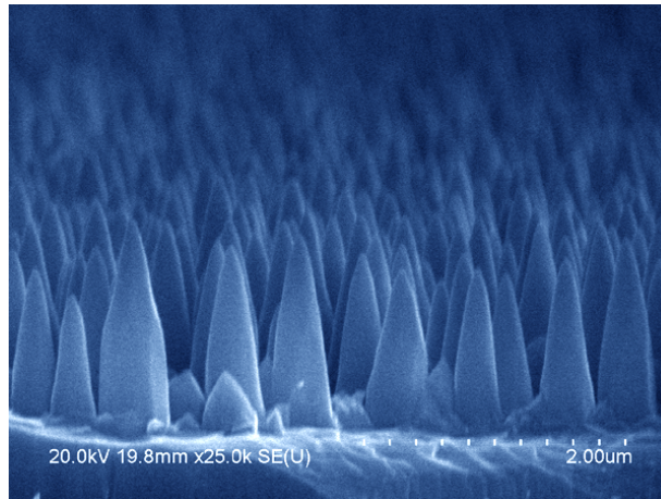
Figure 4: SEM side view of ZnO nanocones grown on Si (111).
