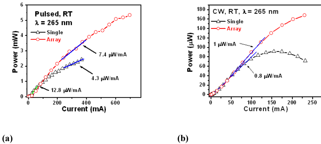
Figure 8: (a) Pulsed P-I measurements of a single 265 nm diode and an array of four 265 nm diodes connected in series and (b) continuous wave measurements of a single 265 nm diode and an array of four 265 nm diodes connected in series.
