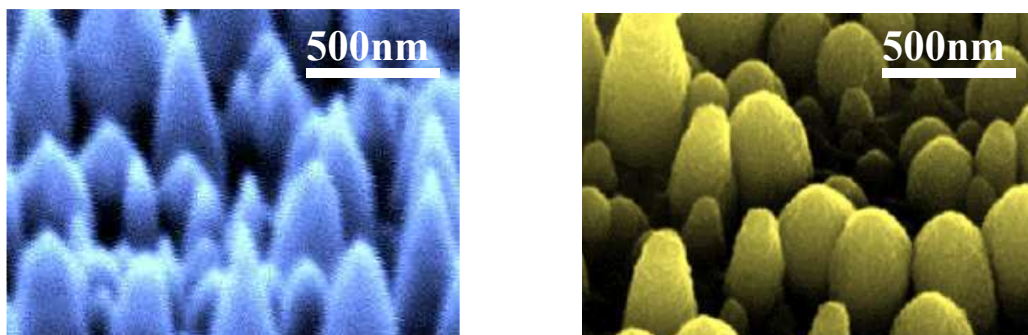
Figure 2. SEM images of a nano ZnO/Si sample before and after MOVPE overgrowth of GaN.
