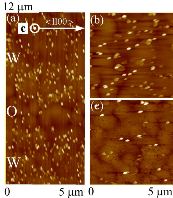
Figure 24. AFM images of green MQWs on (a) LEO GaN (5 μm x 12 μm), (b) wing area of LEO GaN (5 μm x 5 μm), (c) conventional GaN (5 μm x 5 μm). ‘W’, and ‘O’ corresponds to the wing and opening regions, respectively.
