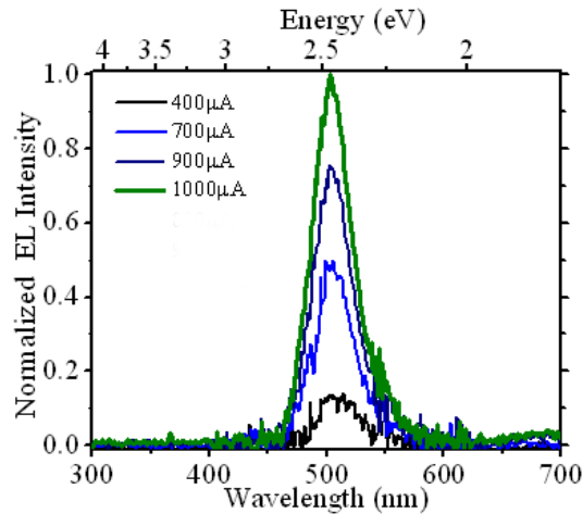
Figure 14. EL spectrum showing green emission from inverted hybrid heterojunction with PLD n-ZnO substituted for MOCVD n-GaN.
