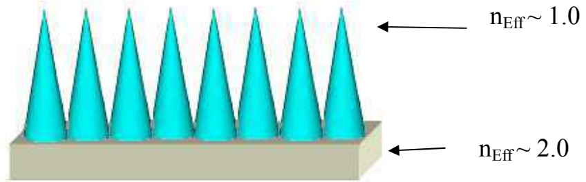
Figure 4: Schematic illustrating the graded effective refractive index of the nanocone type structures
