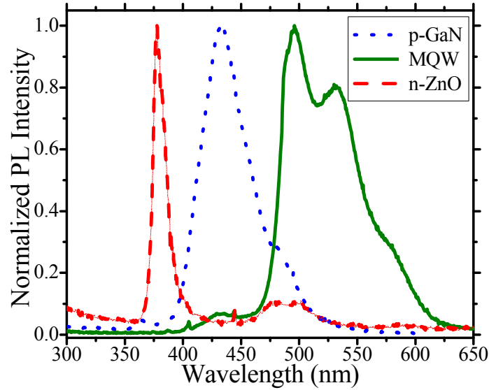
Figure 41. RT normalized PL spectra as consecutive p -GaN, InGaN/GaN MQW, and n -ZnO layers were grown on AlN/Sapphire.
