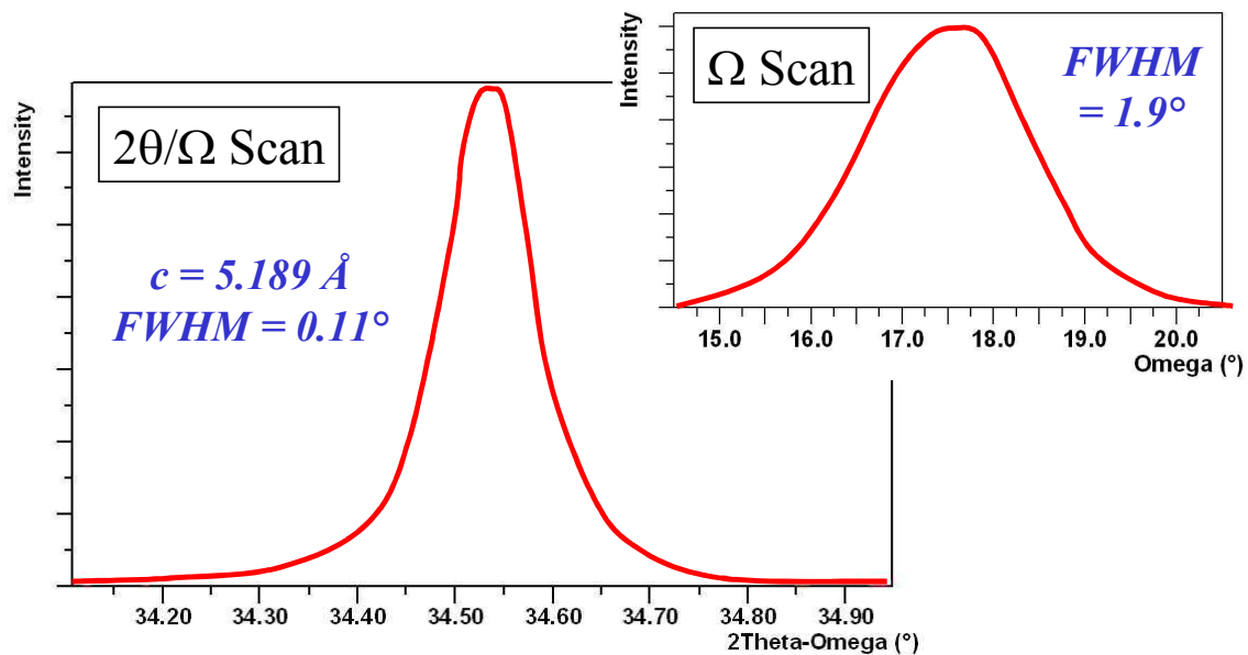
Figure 3. XRD 2\theta/\omega and \omega scans for the (0002) peak of the ZnO/Si 3 N 4 /SiO 2 /Si (111).
