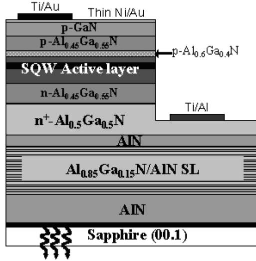
Figure 3: Device structure of high-power 280 nm LED.
