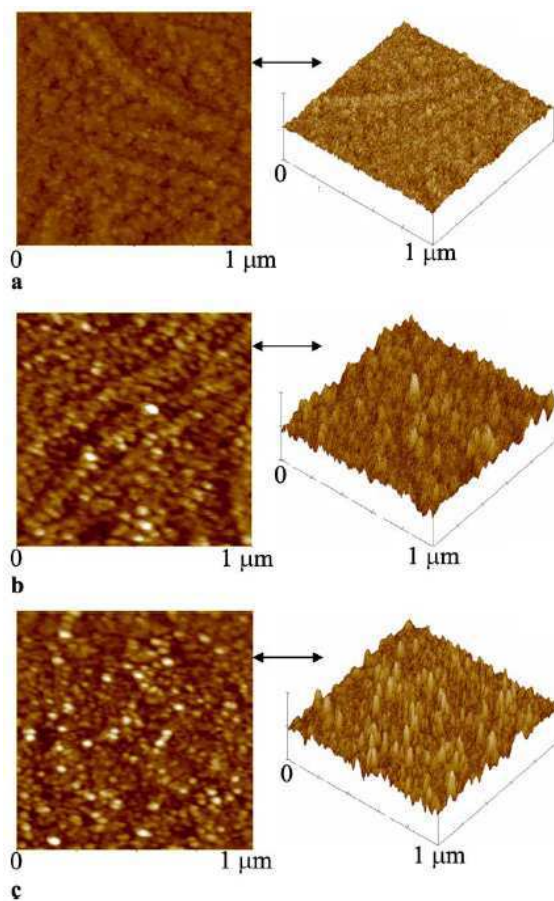
Figure 48. AFM ( 1\text{ }\mu\text{m} \times 1\text{ }\mu\text{m} ) images of (a) 2.9 ML, (b) 4.4 ML, and (c) 5.8 ML InGaN grown at T=633^\circ\text{C} .
