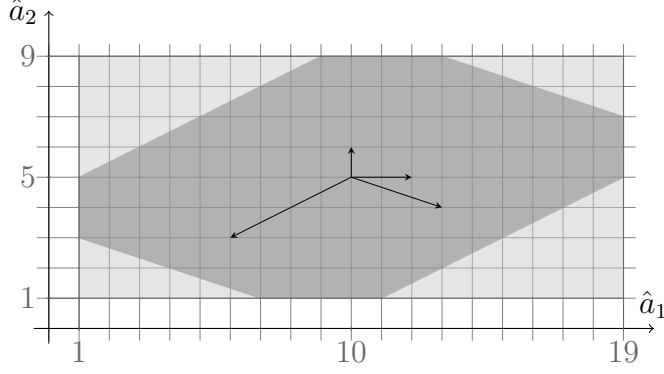
Figure 3.1: The joint range (the center symmetric polygon in dark gray) of two affine forms. This zonotope is spanned by the generators drawn in its center. The box \hat{\mathbf{a}}_1 \times \hat{\mathbf{a}}_2 (light gray) encloses the zonotope.
