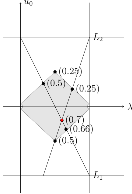
Figure 6.6: The evaluation of the objective function of (P_r) at each vertex.
