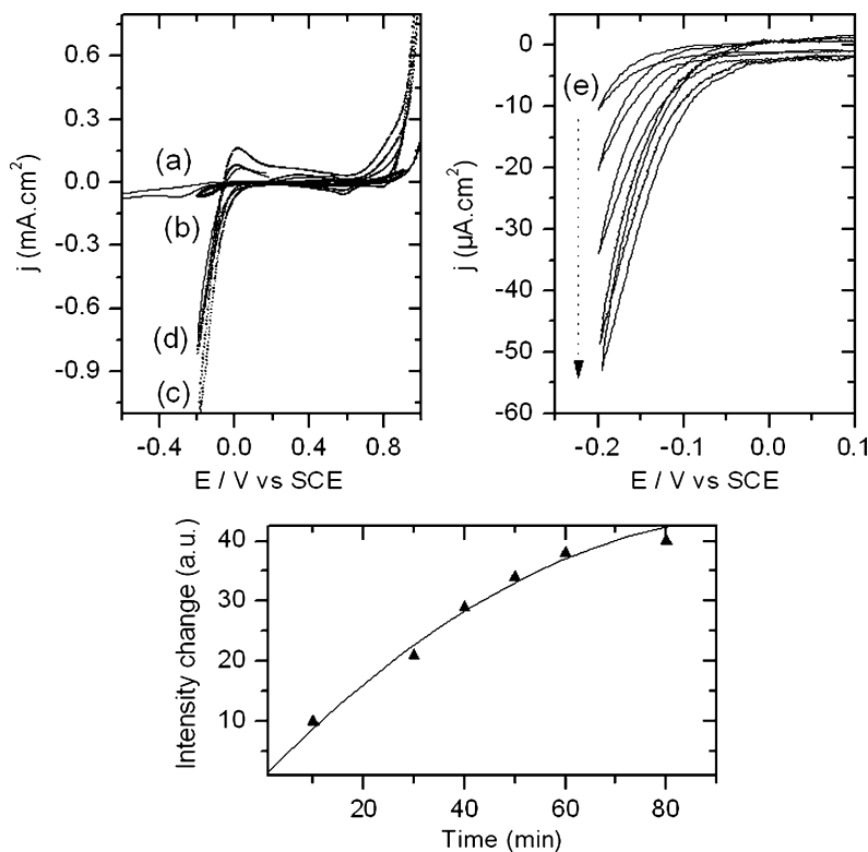
Fig. 9. (A) Cyclic voltammetry registered at 20\text{ mV s}^{-1} : (a) PBS 0.1 M solution on gold surface, (b) PBS 0.1 M and glucose 0.1 M solution on gold surface, (c) PBS 0.1 M and \text{H}_2\text{O}_2 3 \times 10^{-2}\text{ M} solution on gold surface, (d) PBS 0.1 M and \text{H}_2\text{O}_2 3 \times 10^{-2}\text{ M} solution on gold PAP modified surface. (e) Cyclic voltammetry registered at 20\text{ mV s}^{-1} during time, measured on glucose oxidase grafted PDP modified gold surface with addition of 7.69 \times 10^{-3}\text{ M} of glucose in 0.1 M PBS buffer. (B) Kinetic activity of a GOD modified gold electrode represented by the variation of intensity of the generated \text{H}_2\text{O}_2 electrochemically detected during time when glucose was added in cell. The initial rate of \text{H}_2\text{O}_2 production follows pseudo-first order appearance kinetics. First order rate constant k_{\text{obs}} is 0.016 \pm 0.003\text{ a.u./min} and intensity of current density change is 59.4 \pm 7.7\text{ a.u.}
