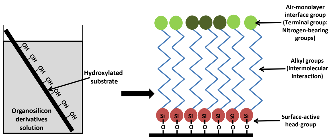
Figure 13 : Self-assembled monolayers are formed by simply immersing a substrate into a solution of the surface-active material. The driving force for the spontaneous formation of the 2D assembly includes chemical bond formation of molecules with the surface and intermolecular interactions [99].
