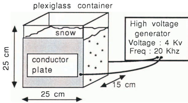
Fig. 1. Snow-warming device.
