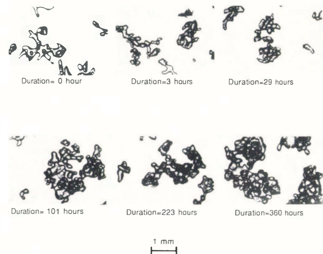
Fig. 2. Evolution of snow crystals submitted to a liquid-water content equal to 2% per mass. The duration since the end of the wetting is expressed in hours.
