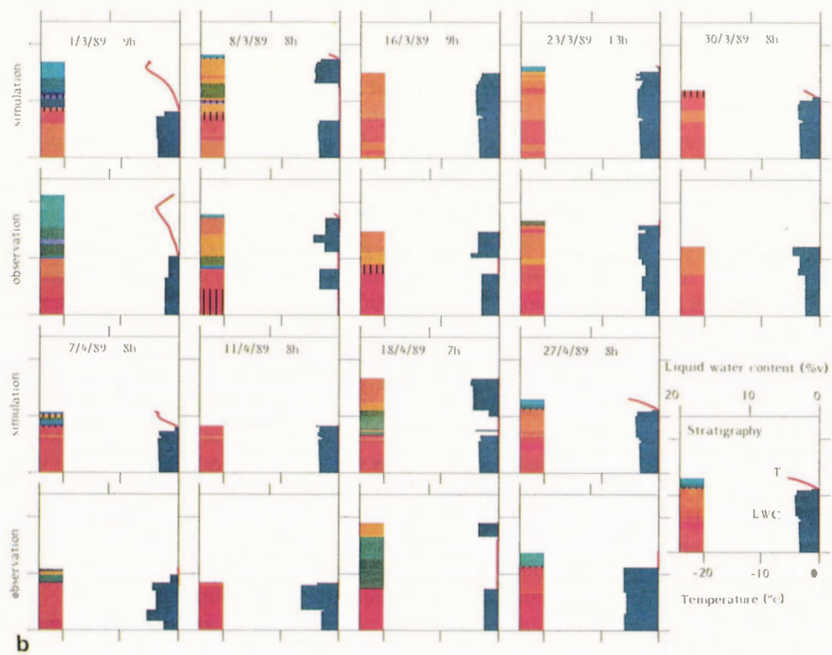
Fig. 7. Comparison between simulated and observed profiles and stratigraphy. Grain types are described by a colour coding. The correlation between these colours and the formalism used to describe snow is shown in Figure 8. Black vertical hachures show crusts.
