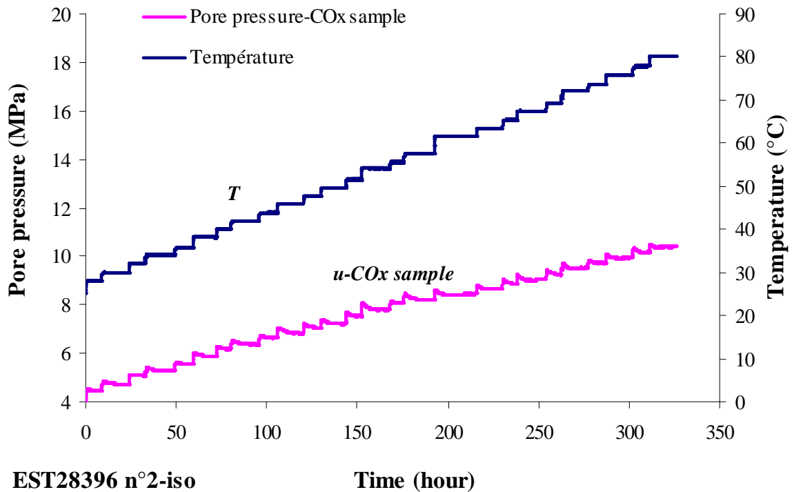
Figure 9: Thermally induced pore pressure in the second sample (EST27396 n°2-iso).
