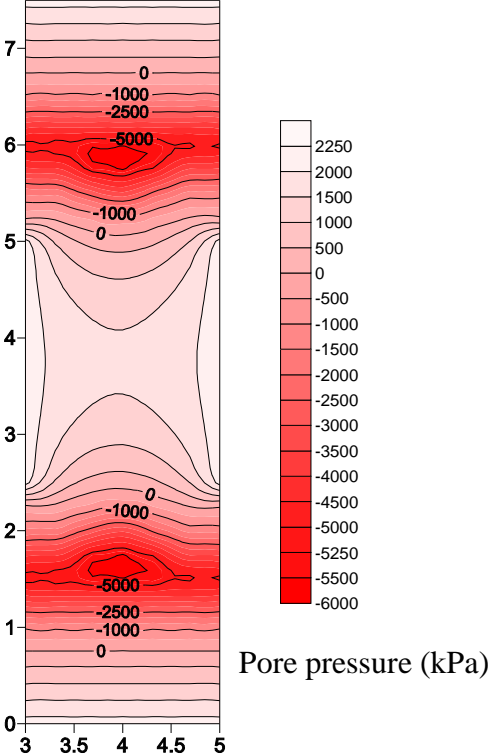
Fig. 16. Resaturation phase: computed pore pressure in the sample after 7 hours
