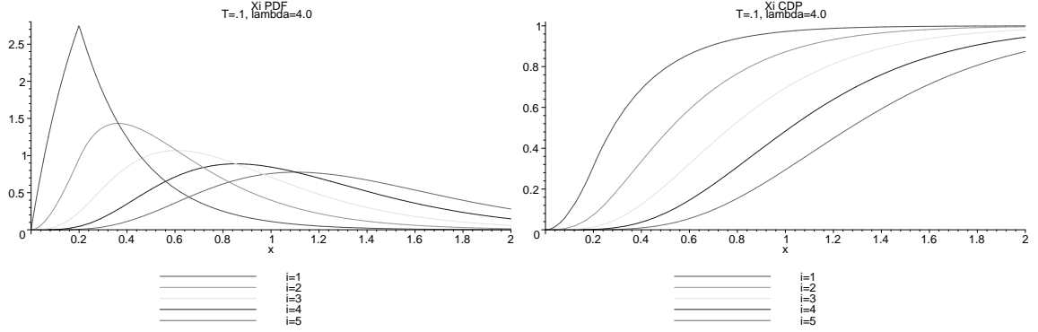
Figure 5.7: (a) Probability density function (PDF) for X(i) , for i = 1, 2, 3, 4, 5 , T = 0.1\text{sec} ; (b) Cumulative distribution function (CDF) for X(i) , for i = 1, 2, 3, 4, 5 , T = 0.1\text{sec} .
