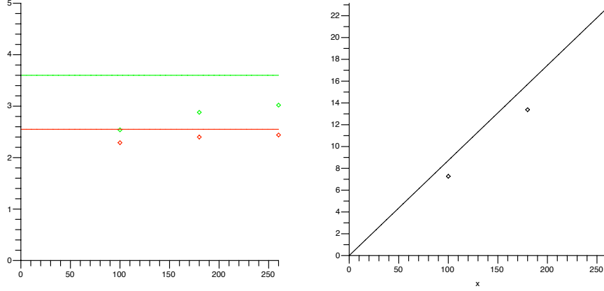
Figure 7.8: Average link density on a 6 \times 6 map, (a) SLO overlay: Maple simulations (dots), theory (plain), SLO with distance cost (red), uniform cost (green), (b) Full network: Maple simulations (dots), theory (plain).
