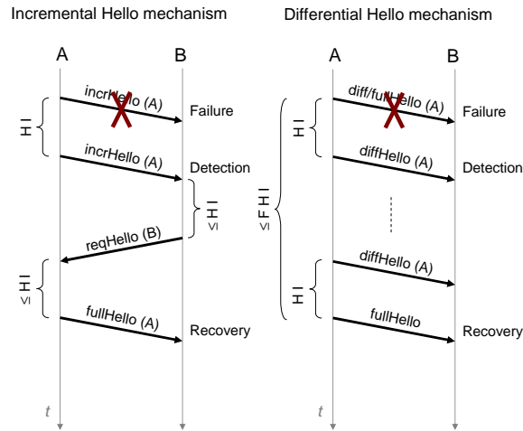
Figure 12.1: Differential and incremental behavior in case of a single Hello packet transmission failure. H_I denotes the time between two consecutive Hello packet transmissions, and F_H I denotes the time interval between two consecutive full Hello packet transmissions.
