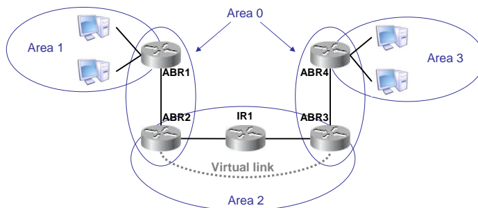
Figure 10.5: Virtual link between ABR_2 and ABR_3 through Area 2 provides connection of Area 0 ( backbone ).
