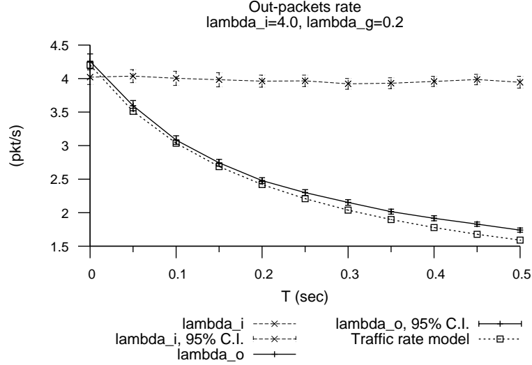
Figure 5.18: Out-packet ( \lambda_{out} ) and in-packet ( \lambda_{in} ) rates, for different values of T and a theoretical in-packet rate \lambda_{in} = 4 \frac{pkt}{s} (simulations).
