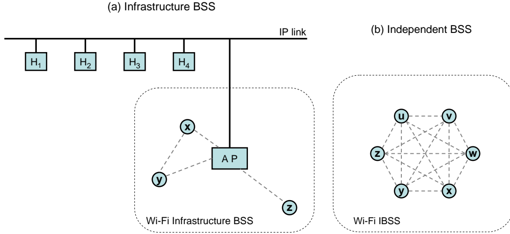
Figure 2.4: (a) Infrastructure BSS, (b) Independent BSS (IBSS).
