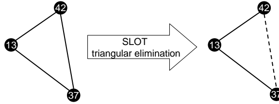
Figure 7.4: The SLOT triangular elimination under unit link cost. The link connecting routers with the highest ids, \overline{42, 37} in the picture, is excluded.
