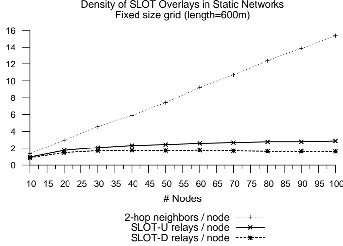
Figure 7.9: Density of SLOT overlays (SLOT-U and SLOT-D) in static networks. The SLOD-D simulations are computed with the quantized cost: \text{cost}(\overline{xy}) = \lceil K \frac{d(\overline{xy})}{r} \rceil , with K = 10 and d(\overline{xy}) being the Euclidean distance between x and y .
