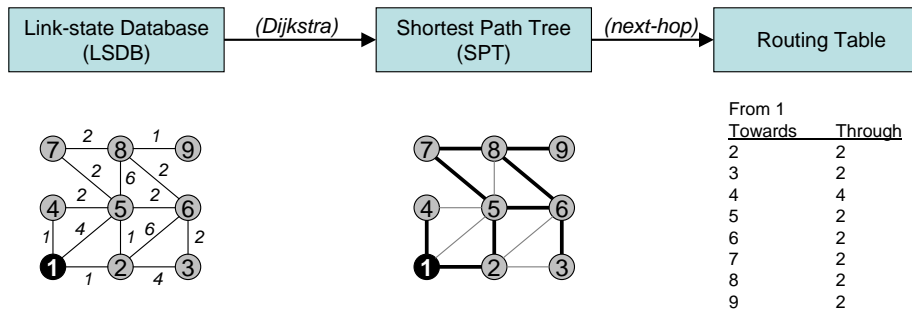
Figure 4.1: Construction of the routing table from the network graph indicated in the LSDB, with a network example.
