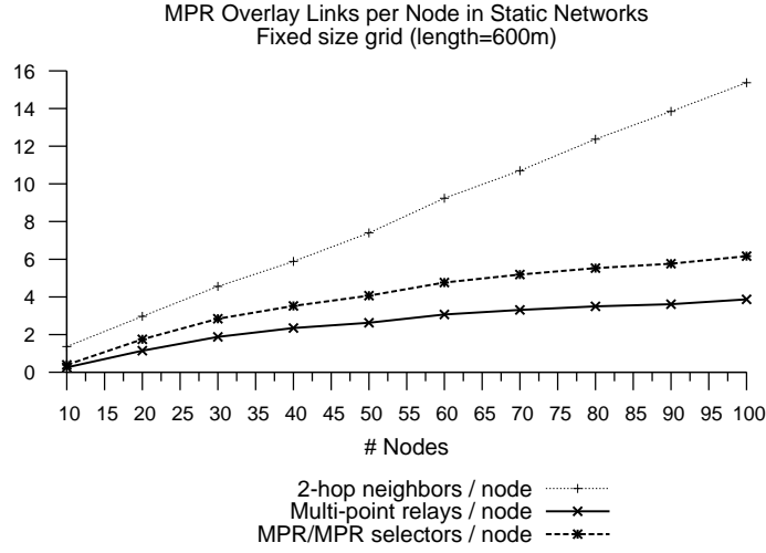
Figure 8.4: Density of MPR overlays for a static, error-free network. Results from simulations.
