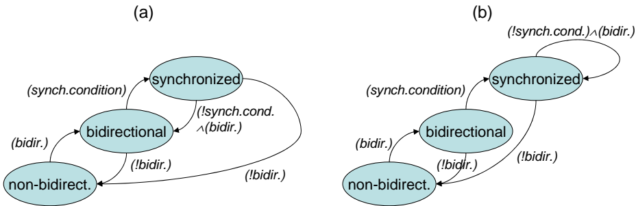
Figure 8.7: (a) Non-persistent and (b) persistent approaches for link synchronization.
