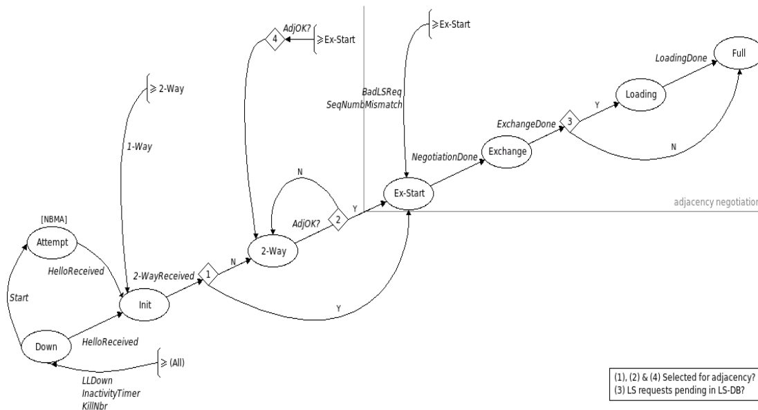
Figure 10.7: Finite States Machine for neighbors in OSPF.
