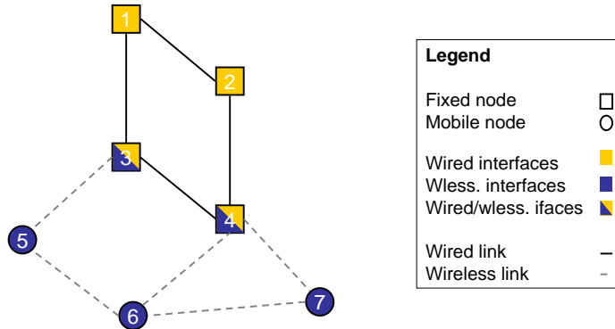
Figure 4.3: Example of compound (wired/wireless) network.
