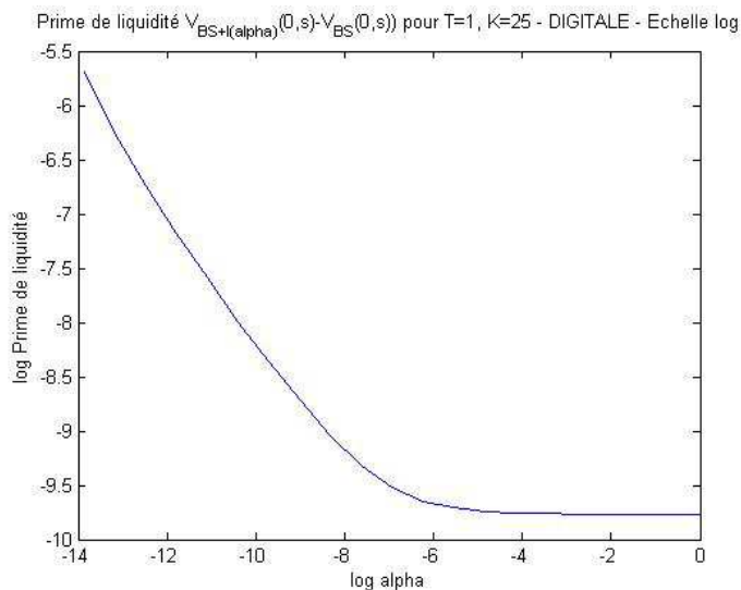
Figure 7.4: \log(V^\varepsilon - v^{BS}) - T = 1 , K = 25 , s = 15 , \sigma = 0.5 , \varepsilon = 0.1 , \ell = 1
