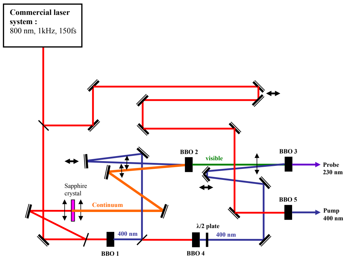
Figure 6.3 Schematic representation of the pump/probe source system.
