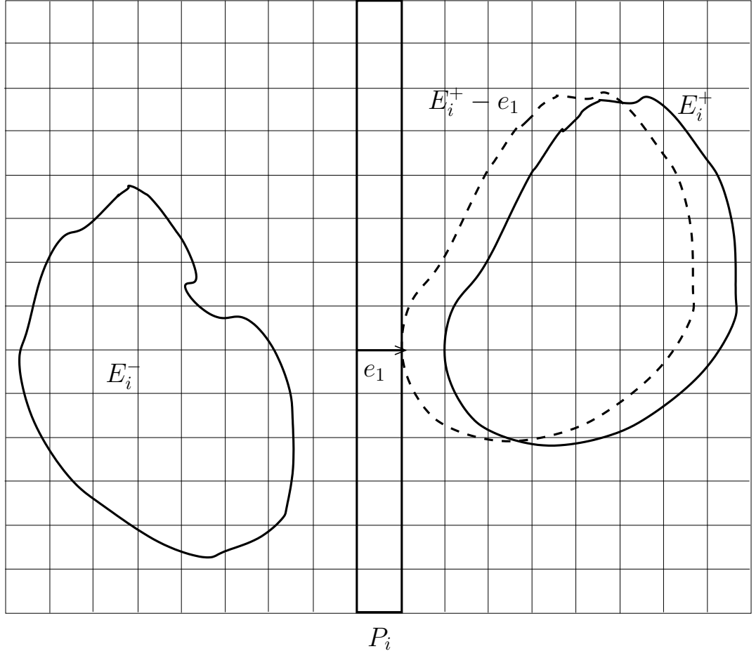
Figure 3.1: The construction in the proof of Proposition 3.2.3.
