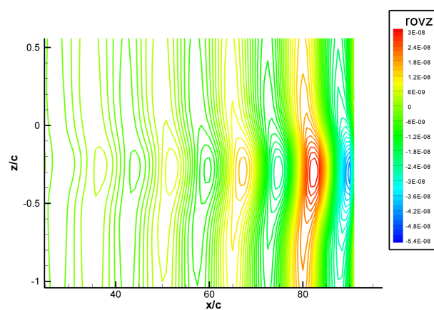
(a) \widehat{\rho w} : sillage
