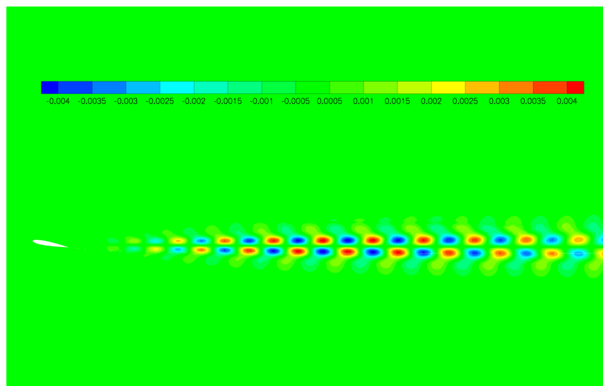
(b) Composante \widehat{u}
