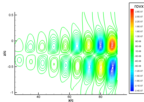
(a) \widehat{\rho u} : sillage
