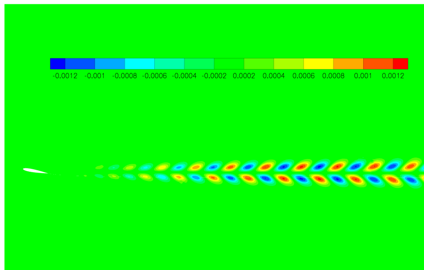
(a) Composante \widehat{\rho}
