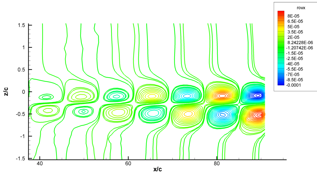
(a) \widehat{\rho u} : sillage
