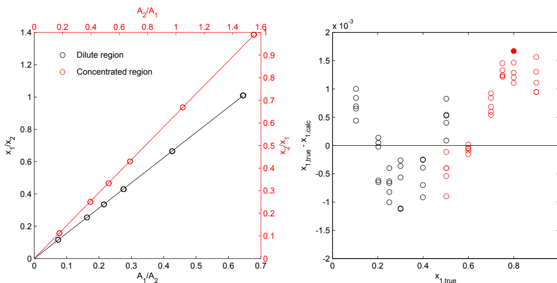
Figure 3.4: TCD Calibration for the ethanol (1) + cyclohexane (2) system using the method of Raal and Mühlbauer. left: Linear relation between the area and mole fraction ratios. The black line (and axes) depicts the dilute region calibration, the region defined as 0 < x_1 \leq 0.5 , while the red depicts the concentrated region calibration, used for 0.5 \leq x_1 < 1 . right: Error compared to the true composition, resulting from the use of Eqn. (3.3) and (3.4). The filled symbol denotes the maximum error, in mole fraction.
