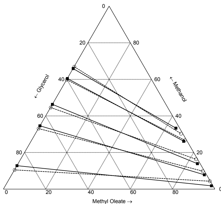
Figure 5.43: LLE modeling of the methyl oleate (1) + methanol (2) + glycerol (3) ternary system at 333.2 K and 101.3 kPa, using the non-polar PC-SAFT (—) and the following binary interaction parameters: k_{12} = 0 , k_{13} = 0.01 and k_{23} = -0.04 . Pure parameters for methanol were taken from [94], and the others from this work. Experimental data (○) and tie lines (---) were taken from Negi et al. [314].
