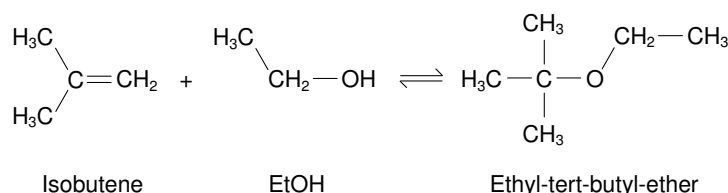
Figure 1.13: Synthesis reaction of ETBE from isobutene and ethanol
