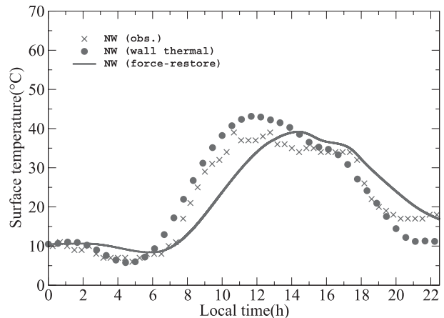
FIG. 8. The northwest wall temperature evolutions obtained with different surface temperature models (crosses: measurements; filled circles: wall thermal model; solid line: force–restore method).
