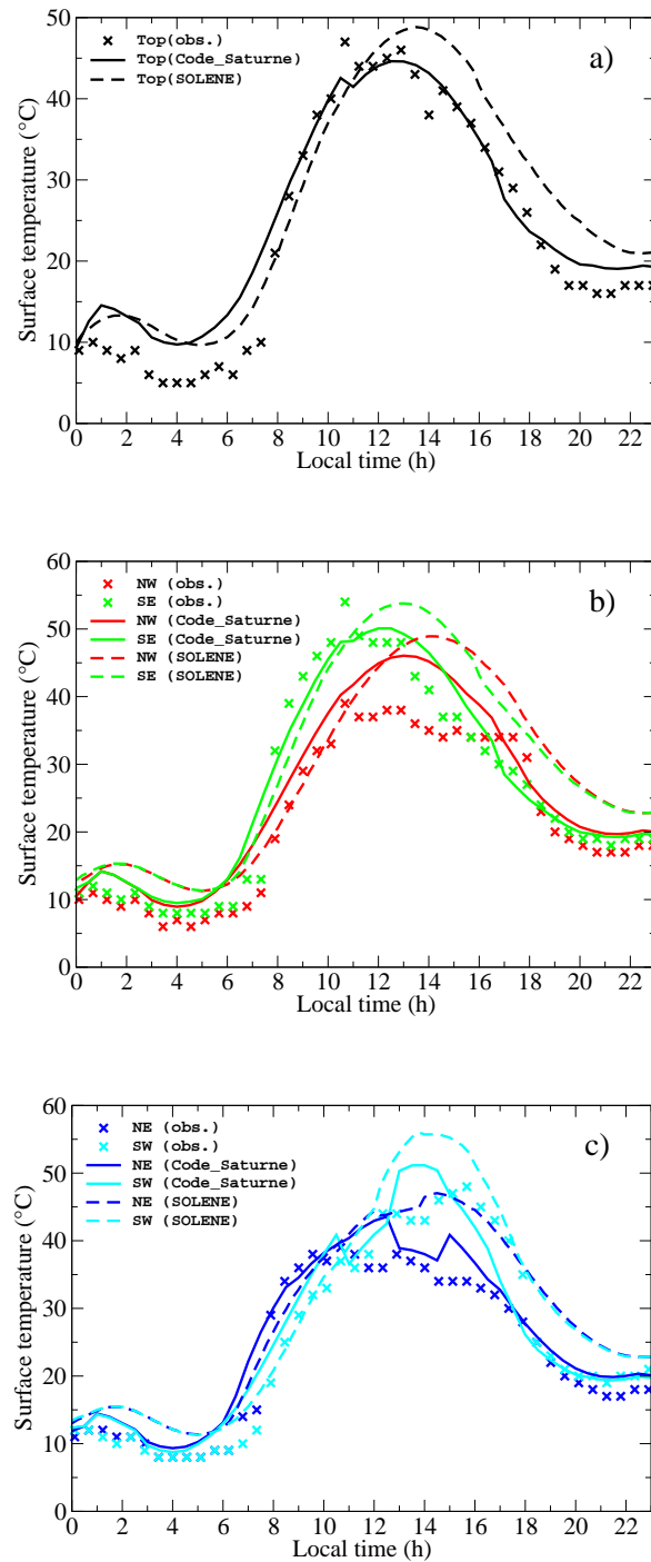
Figure 4.9: Evolution of surface temperature of different faces of the central container in MUST field experiment during a diurnal cycle (cross symbol: Measurements; Straight line: Simulation with Code_Saturne ; Dashed line: Simulation with SOLENE).
