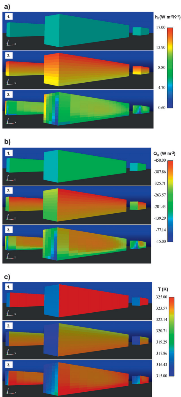
FIG. 9. Comparison of three convective models with visualization of the southeast and northeast walls at 1230 LT: (a) transfer coefficient h_f ( \text{W m}^{-2} \text{K}^{-1} ), (b) sensible heat flux Q_H ( \text{W m}^{-2} ), (c) surface temperature T ( \text{K} ). Label 1 indicates the constant h_f model, label 2 is for the 1D h_f model, and label 3 represents the 3D h_f model.
