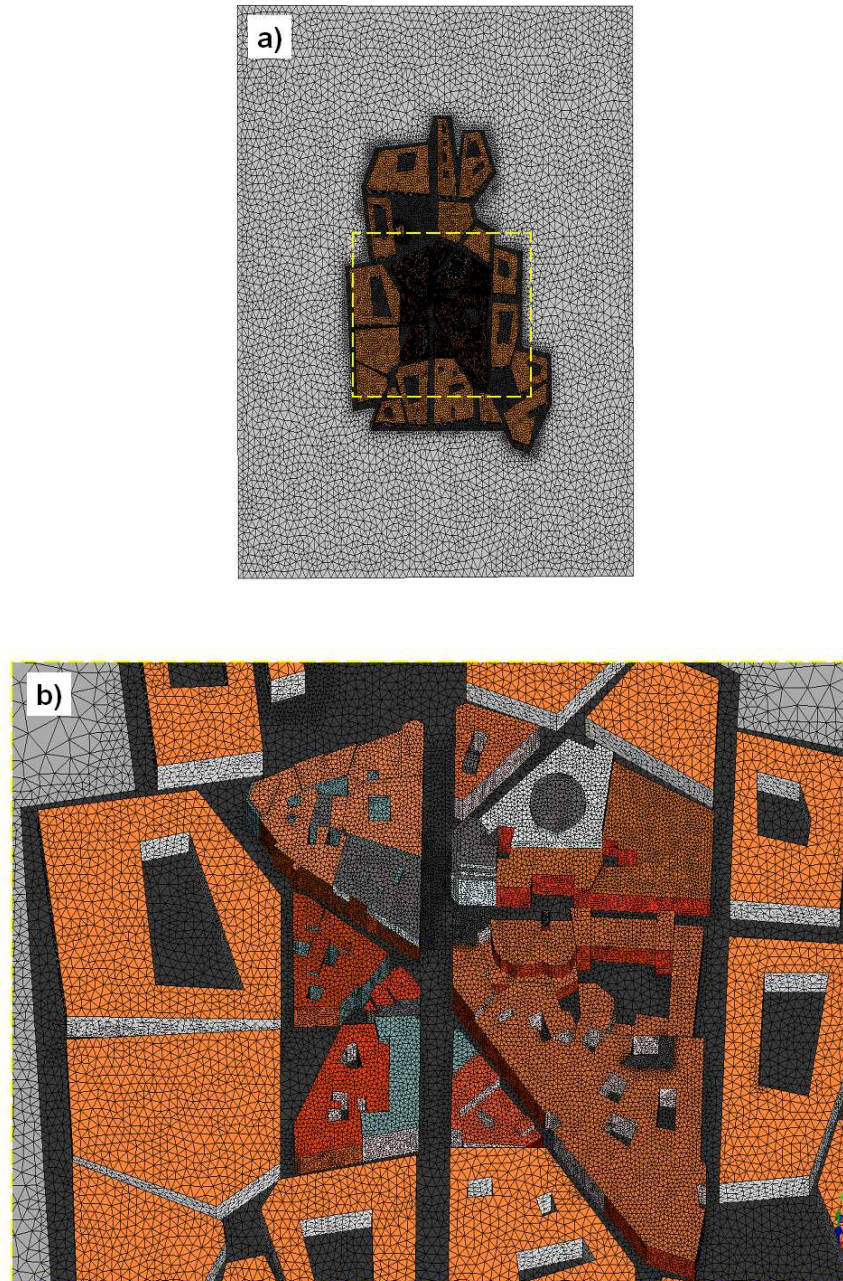
Figure 6.5: Tetrahedral mesh on the central area: a) whole area; b) zoom in the selected area a) (yellow contour).
