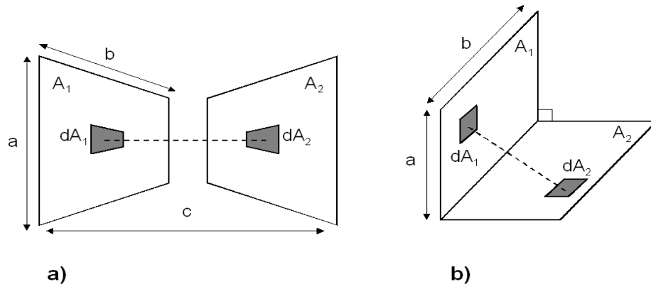
Figure 4.1: Schematics of the view factors or shape factors for the urban street canyon. (a) two parallel in-line planes; (b) two perpendicular planes.
