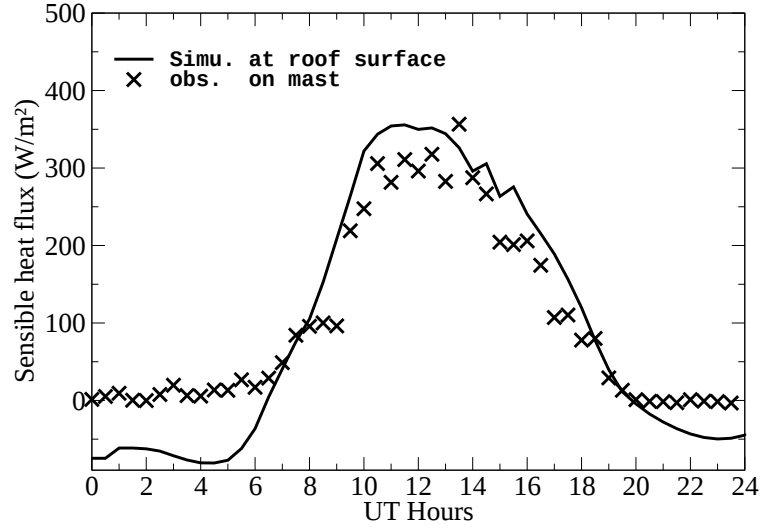
Figure 6.11: Diurnal variation of sensible heat flux calculated at roof surface (full line) and measured on the mast (cross symbol).
