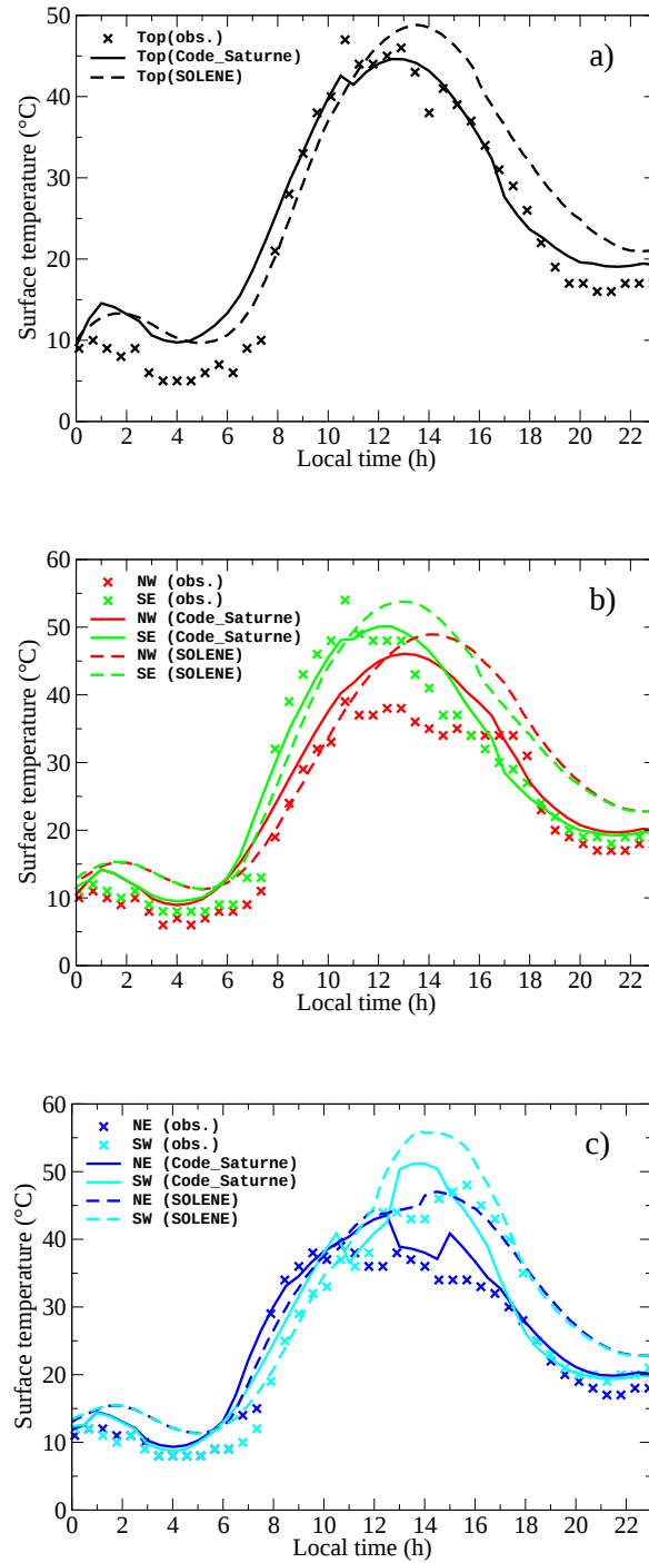
Figure 4.9: Evolution of surface temperature of different faces of the central container in MUST field experiment during a diurnal cycle (cross symbol: Measurements; Straight line: Simulation with Code_Saturne ; Dashed line: Simulation with SOLENE).
