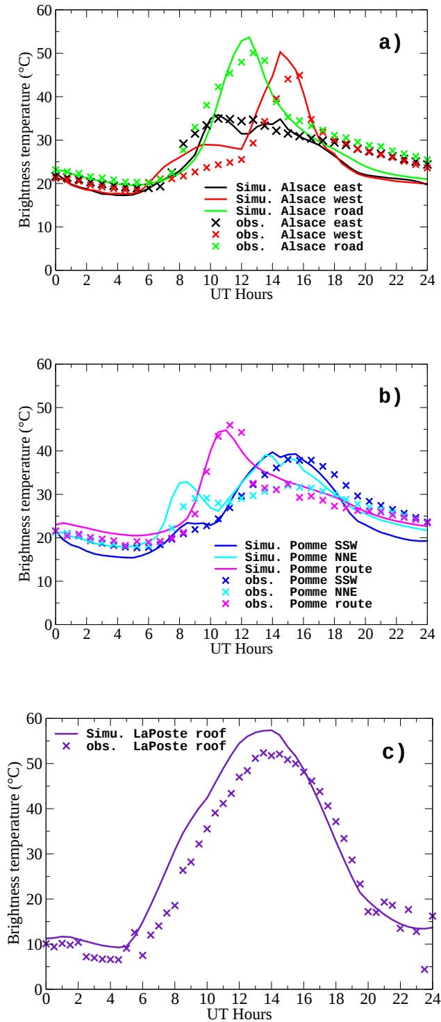
Figure 6.9: Evolution of brightness surface temperature of different positions of the infrared thermometers during a diurnal cycle (cross symbol: Measurements; full line: Simulation).
