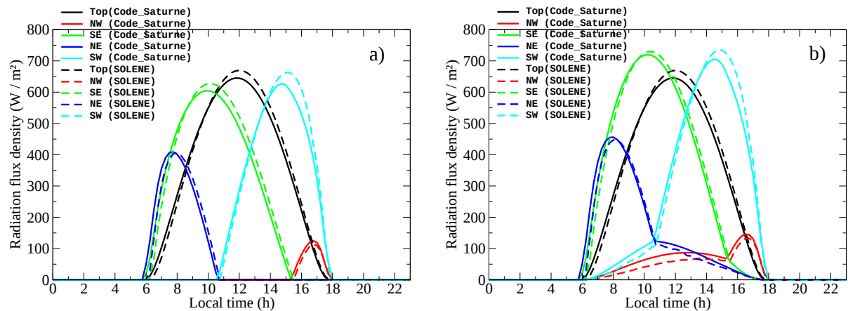
Figure 4.5: Comparison for the central container of the MUST field experiment of direct solar radiation flux on roof (top), N-W, S-E, N-E and S-W walls during a diurnal cycle between Code_Saturne (Straight line) and SOLENE (Dashed line): a) incident direct solar flux; b) direct solar flux after multi-reflections.
