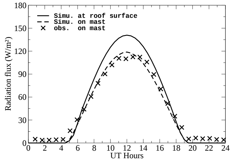
Figure 6.14: Same as Fig. 6.12 but for outgoing solar flux.
