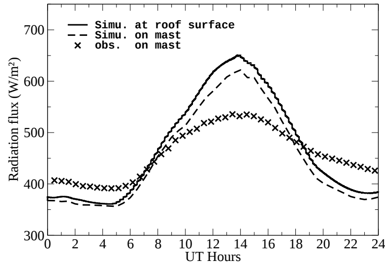
Figure 6.12: Diurnal variation of outgoing infrared flux calculated at roof surface (full line), at the mast level (dashed line) and measured on the mast (cross symbol).
