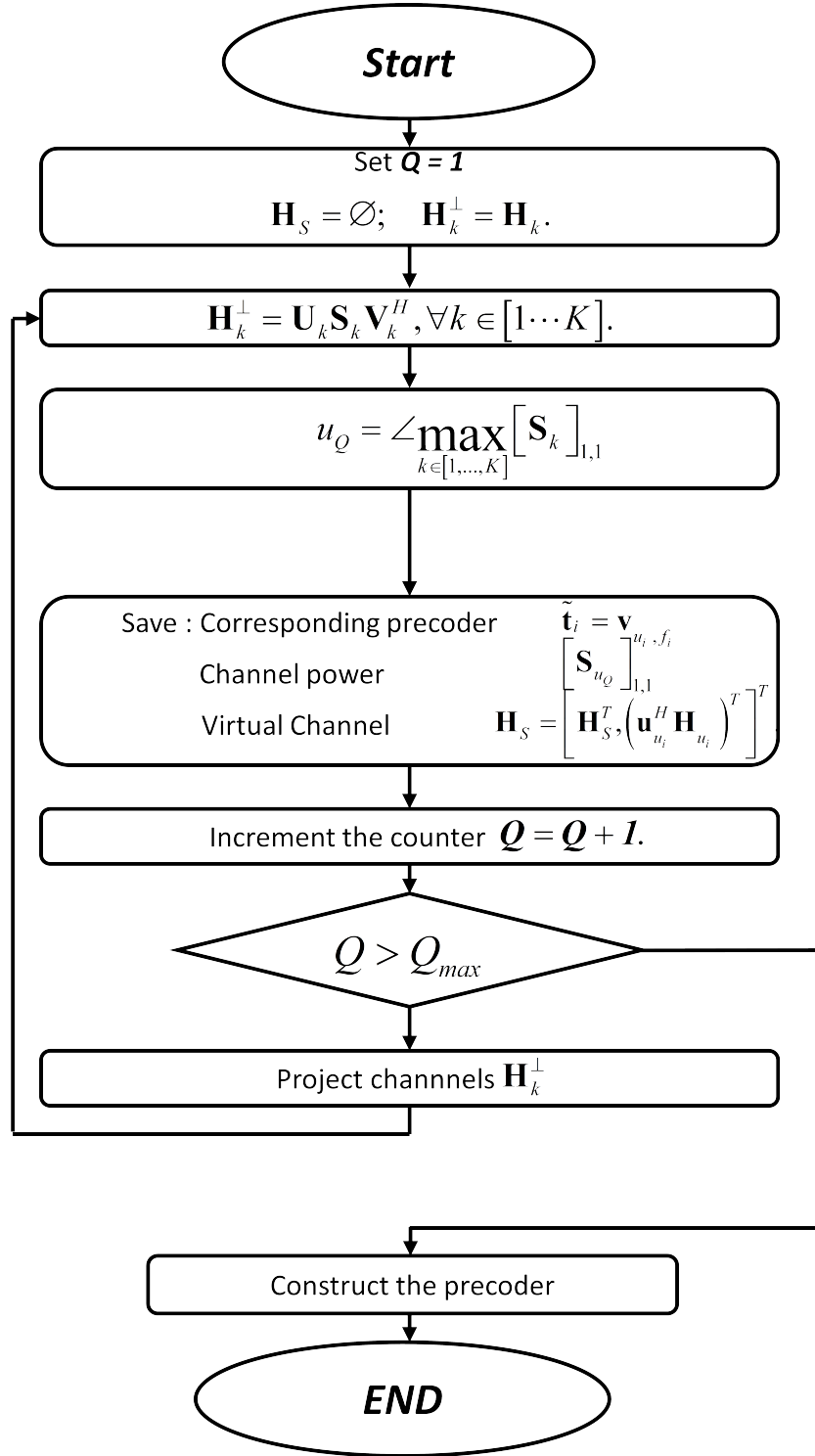
Figure 4.1: Réursive stream selection (main algorithm).
