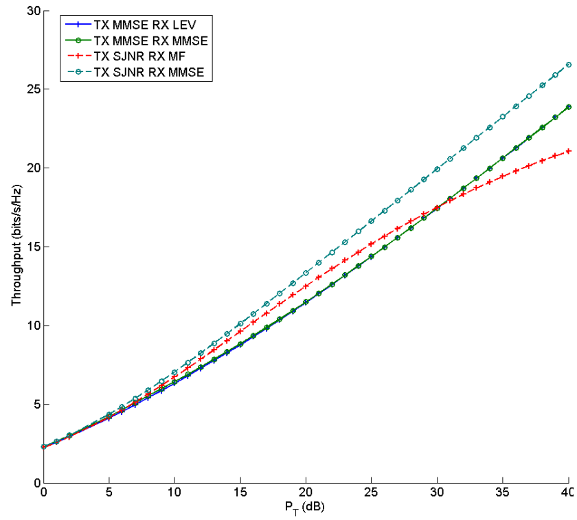
Figure 4.5: Throughput for N_T = 2 , N_R = 2 and K = 2 .
