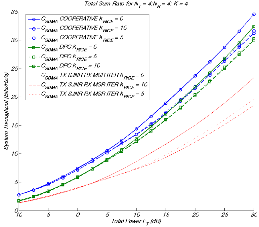
Figure 5.8: Throughput as a function of total transmit power P_T for N_T = 4, N_R = 4 and K = 4 with \theta channel.
