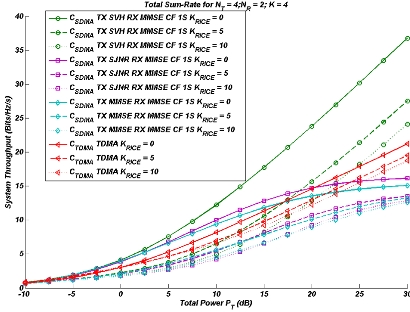
Figure 5.5: Throughput as a function of total transmit power P_T for N_T = 4 , N_R = 2 and K = 4 .
