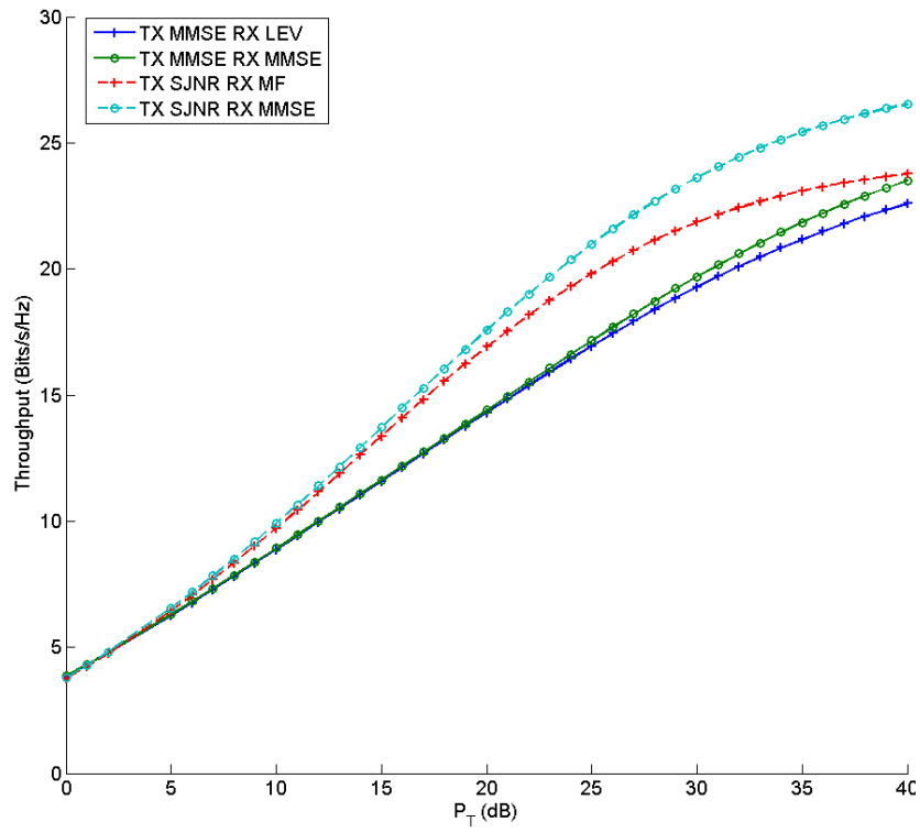
Figure 4.4: Throughput for N_T = 4 , N_R = 2 and K = 3 .
