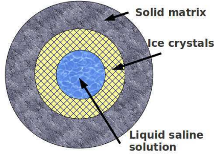
Figure 7.9: Schematic illustration of a partially frozen porous materials. It is assumed that liquid solution is embedded into ice crystals (this assumption actually can be observed in the freezing process of cylindrical capsule, see Figure 2.13 by Guzman and Braga (2005) [149]), then the solution-ice system is embedded into the solid matrix.
