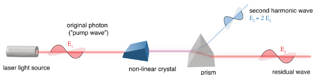
Figure 2.3.: Second-harmonic generation (SHG), also known as frequency-doubling, a non-linear optical process. Source: Jkwchui, Date: 8 th january 2011
