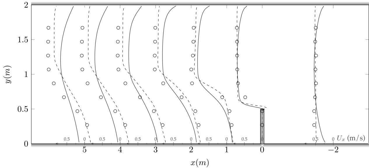
Figure 8.3: Profiles of the horizontal velocity plotted at different locations along the canal. The small axis mark on top of the x -axis represent the values of velocity magnitude. “ \circ ” are experimental results, “—” are results found using Telemac-2D and “---” are results found using OpenFoam.
