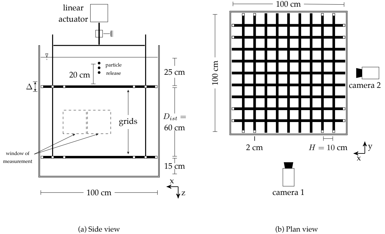
Figure 7.1: Scheme of the double-grid setup (the origin of the axis is located on the bottom right corner in the middle of the cross-section of the lower grid, and the x -axis is inverted). PIV measurements are recorded with camera 1, and particle trajectories using both cameras 1 and 2.
