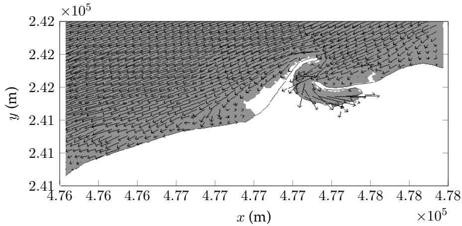
(a) Simulation without any radiation stresses
