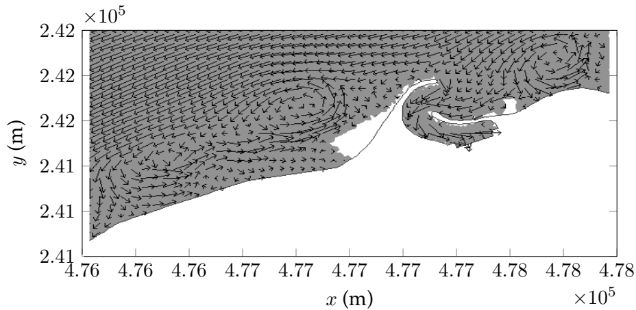
(b) Simulation with radiation stresses calculated from north west ( 125^\circ ) waves with a wave height of 1 m and a frequency 0.11 Hz
