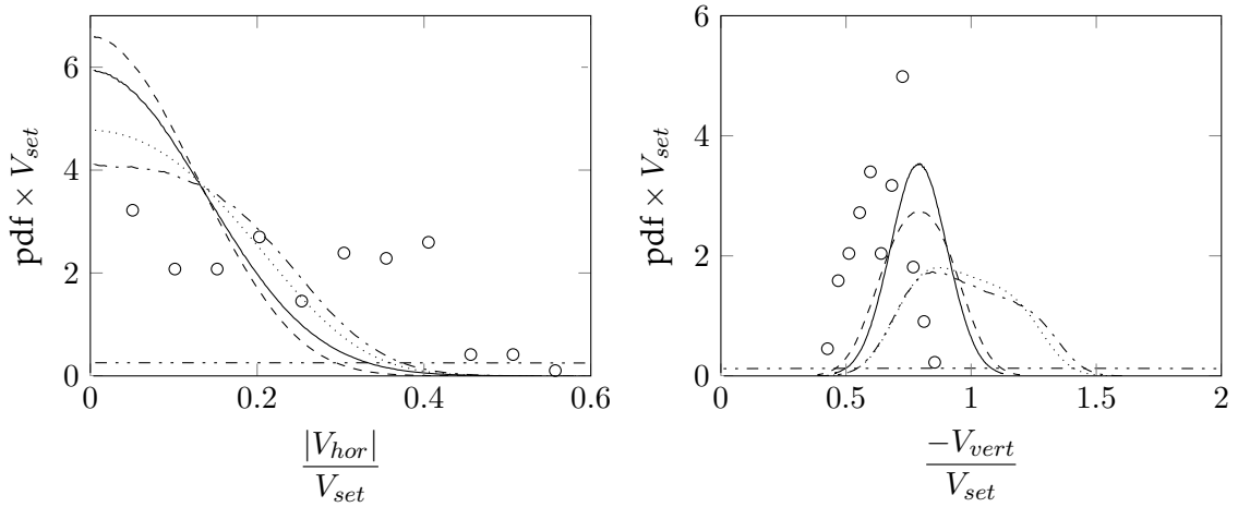
(c) \frac{D}{\lambda_l} = 0.424, \rho_{s/f} = 1.047, St_{set} = 4.58, N_r = 105, Re_{set} = 3450
