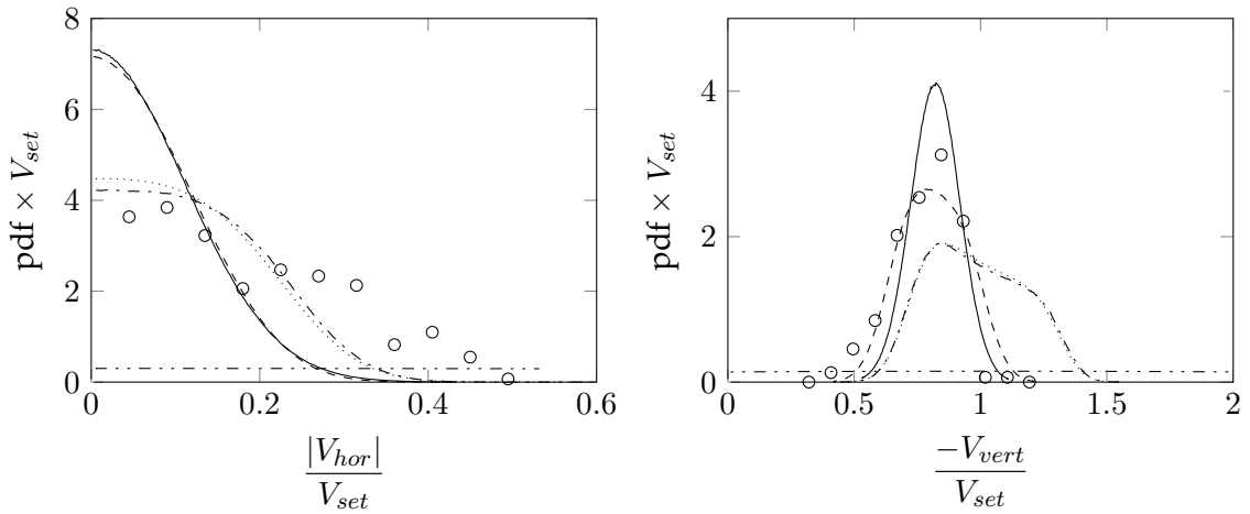
(b) \frac{D}{\lambda_l} = 0.212, \rho_{s/f} = 1.13, St_{set} = 2.06, N_r = 178, Re_{set} = 2020
