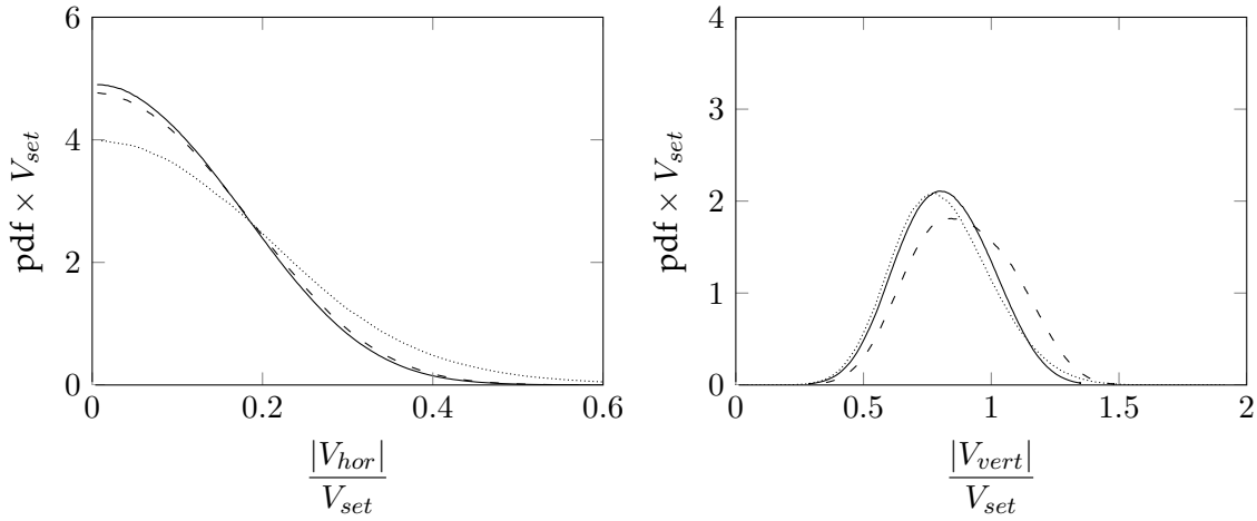
(a) \frac{D}{\lambda_l} = 0.106, \rho_{s/f} = 1.12, St_{set} = 1.52
