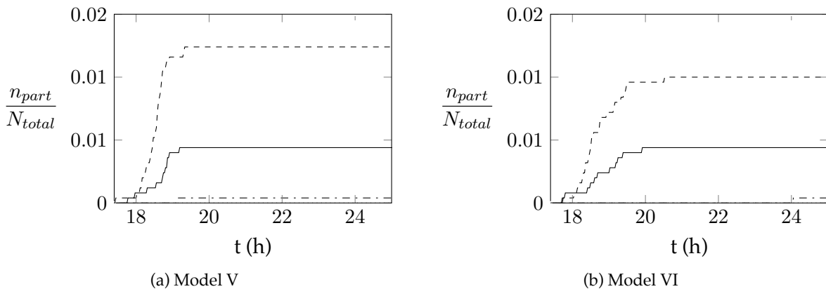
Figure 9.19: Cumulative number of particles entering each pumps for models considering different particles. “—” shows the number of particles entering pump 1, “- - -” shows the number of particles entering pump 2, “.....” shows the number of particles entering pump 3 (for both cases it is equal to zero) and “- - - -” shows the number of particles entering pump 4.
