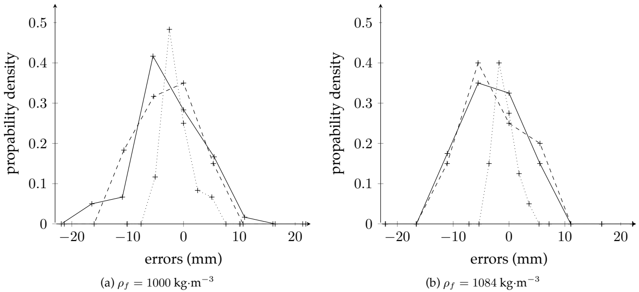
Figure C.2: Probability density functions of the errors on the positions of the fishing weights after the transform given by equations C.1. “+” errors along the x -axis, “-+-” errors along the y -axis and “...+...” errors along the z -axis.
