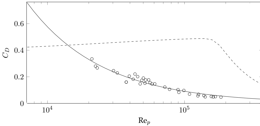
Figure 9.2: The drag coefficient for an Iridaea flaccida . “o” represents the experimental values given in Gaylord et al. (1994), “—” represents the best fit line of those values and “- - -” represents the empirical formula for a sphere given by Almedeij (2008).
