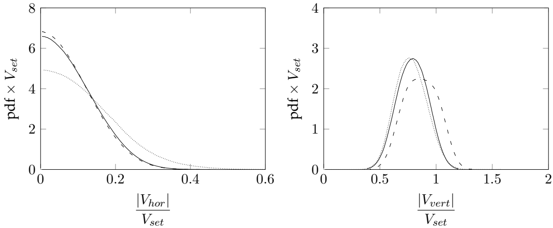
(b) \frac{D}{\lambda_l} = 0.424, \rho_{s/f} = 1.047, St_{set} = 4.58
