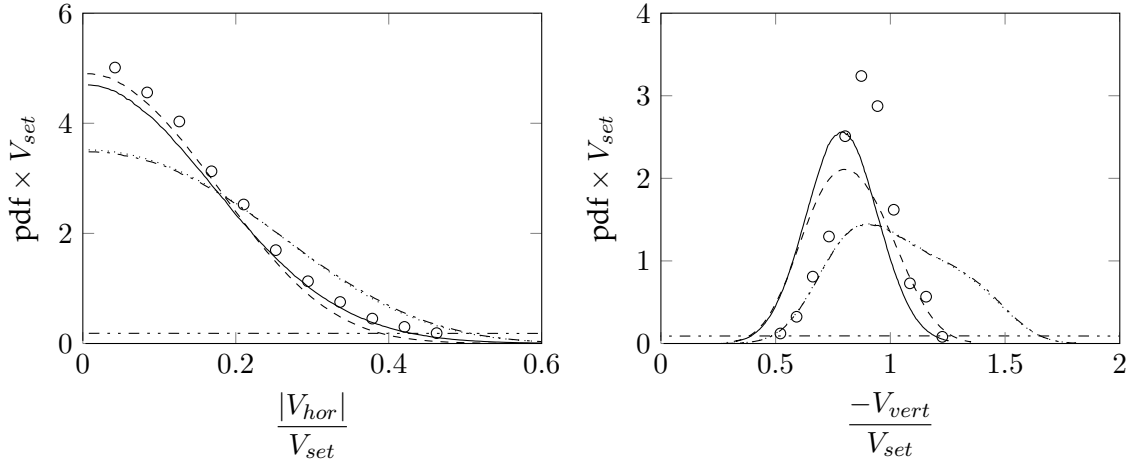
(a) \frac{D}{\lambda_l} = 0.106, \rho_{s/f} = 1.12, St_{set} = 1.52, N_r = 354, Re_{set} = 620
