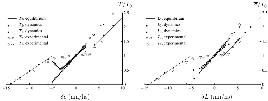
Fig. 8.28 – Comparison between thermal equilibrium and kinetic equilibrium in hard (A) and soft (B) devices. (A): Hard device. (B): soft device. Continuous line: thermal equilibrium computed using Eq.(8.3.22) (A) and (8.3.24)(B). (■): Tension and elongation attained at the end of the simulation (in hard device after 5 ms and in soft device after 10 ms). (●): Tension and elongation attained at the end of the step ( T_1 and L_1 ). Experimental points (open symbols) are taken from (Ford et al., 1977)( T_1 : ×, T_2 : ▽), (Brunello et al., 2007)( T_1 : ◇, T_2 : △) and (Linari et al., 2009)( T_1 : ⊙, T_2 : □).
