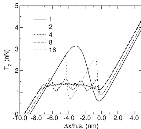
Fig. 8.13 – T_2 curves obtained by A.Vilfan and T.A.J Duke for P = 1 (solid line), P = 2 (dotted line), P = 4 (short-dashed line), P = 8 (long-dashed line) and P = 16 (dot-dashed line). From Vilfan and Duke (2003) Fig.8. The curves are obtained from numerical simulations based on a chemo-mechanical model by measuring the tension attained 2 ms after a stretch/release in hard device. The value of \beta used for their simulations is about 40.
