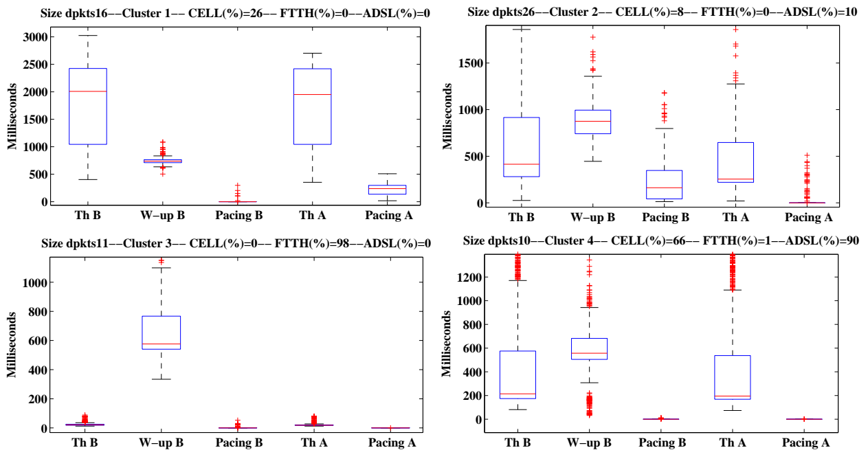
(a) K-means
