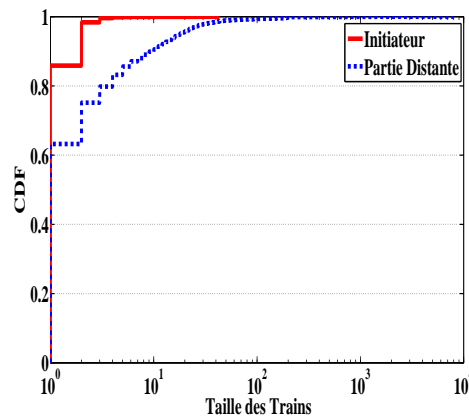
(b) Portland
