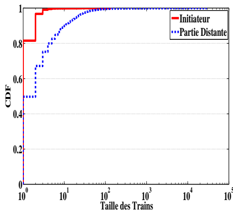
(a) Eurecom
