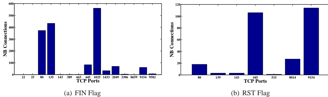
FIGURE 8.5 – Connection With Large Tear-Down : Destination Ports
