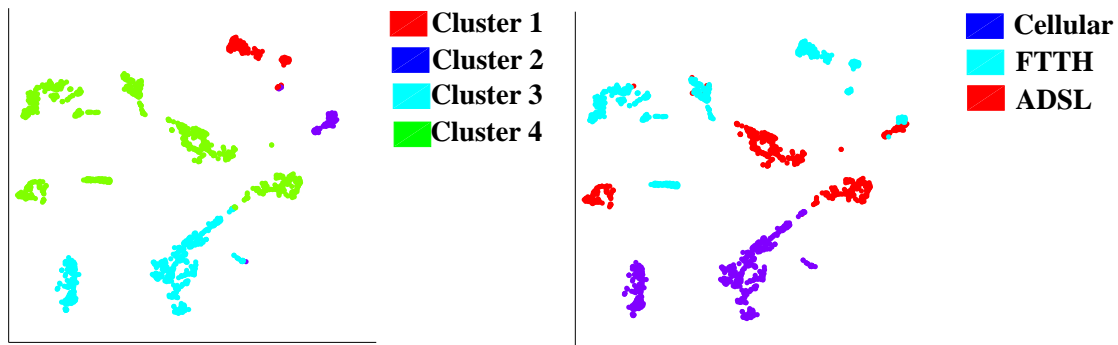
(a) K-means
