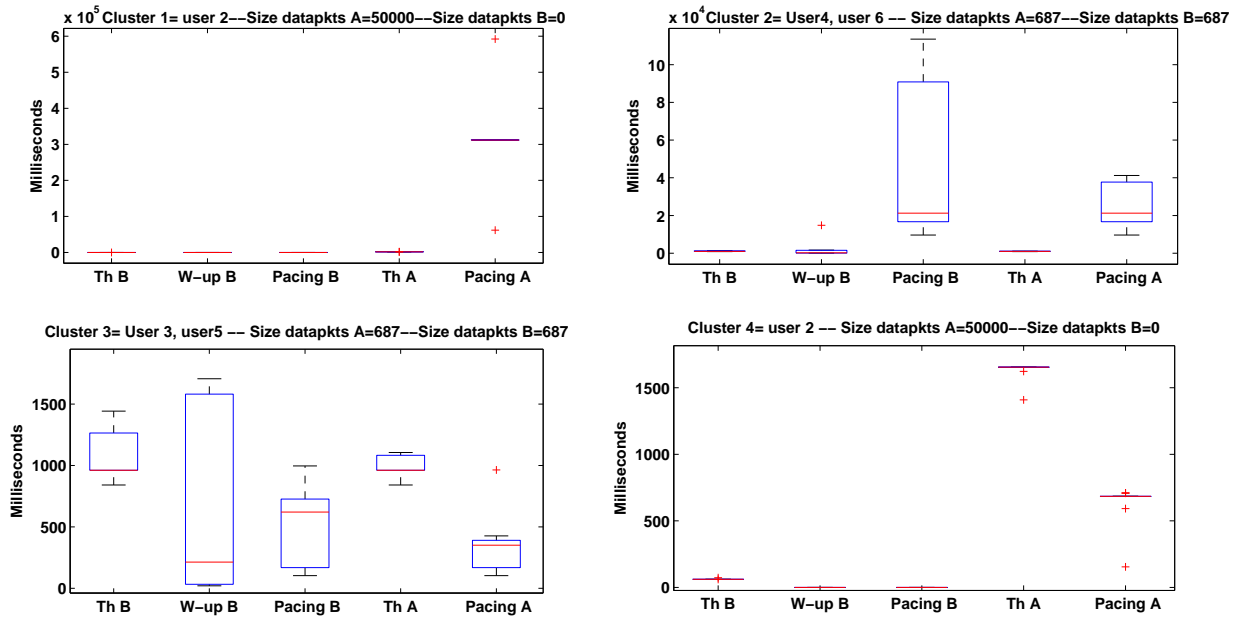
(a) K-means
