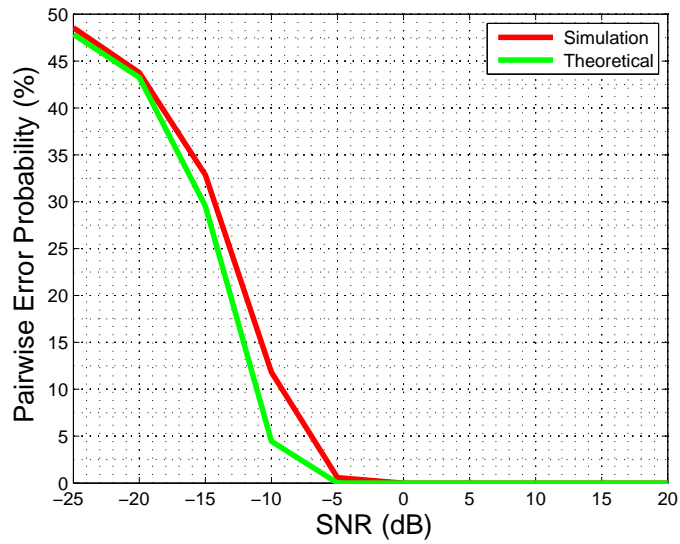
Figure C.16: PEP pour \alpha = 1.1 .
