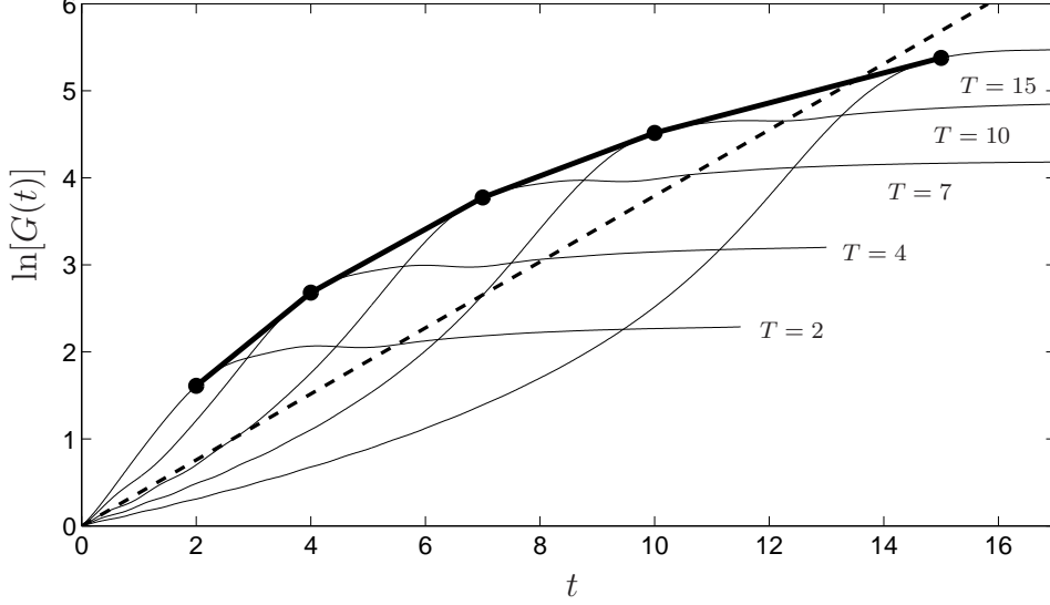
Figure 6.12: Evolution of the energy gain G(t) (thin lines) of the optimal perturbations for (k_x, k_y) = (4.887, 2.957) and T = 2, 4, 7, 10 and 15 . The optimal gain G_{max}(T) corresponding to each curve is indicated by a \bullet sign. The \bullet signs are connected by a thick black line that approximates the envelope of G(t) for (k_x, k_y) = (4.887, 2.957) . The dashed line indicates the gain of the most unstable eigenmode.
