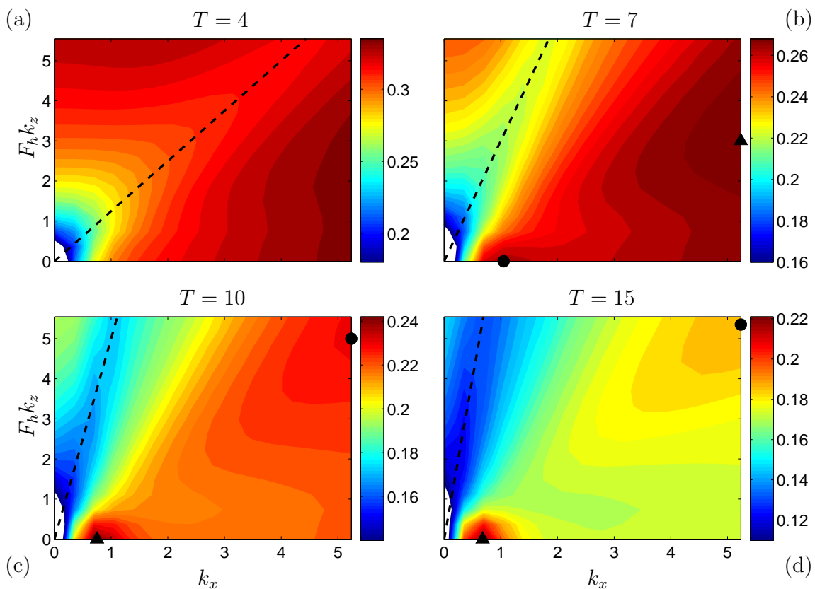
Figure 1: Optimal mean growthrate \sigma_m(k_x, F_h k_z) for optimization times T = 4 (a), T = 7 (b), T = 10 (c), and T = 15 (d). The colorbar is indicated next to each figure. The horizontal and vertical axis are the same on all figures, as shown in the lower left figure (c). The values of the ratio F_h k_z / k_x indicated by the dashed lines are r_{min} = 5/4, 3, 5 and 8 for T = 4, 7, 10 and 15 , respectively. In (b), (c) and (d), the \blacktriangle indicates the maximum of the computed \sigma_m (at the boundary in (c) and the \bullet indicates a secondary local maximum (at the boundary in (c) and (d)).
