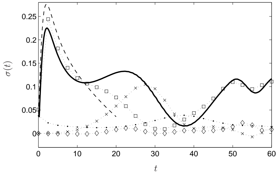
Figure 4.7: Instantaneous growth rate \sigma(t) (thick continuous line, as defined in (4.13)), for the optimal perturbations from t = 0 to t = 60 , k_z = 0.628 of the E-type mode in (a), and k_z = 3.142 of the H-type mode in (b). Dashed lines in (a) and (b) show respectively the growth rate of the OLE and OLH optimal perturbations of the frozen tanh profile for T = 20 . Also shown are the dissipation ( \cdot ) and the growth rate contributions from the mean shear ( \square ), the shear 2D ( \diamond ) and the strain 2D ( \times ).
