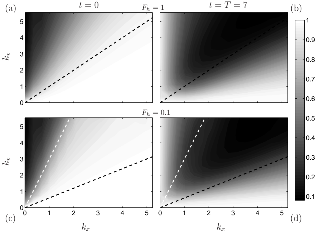
Figure 6.10: Energy fraction in the vortical part \frac{\int |\phi_1|^2 dk_y}{E} for the optimal perturbations at t = 0 (left column a,c) and optimal response at t = 7 (right column b,d). Froude numbers are F_h = 1 for the top row (a,b) and F_h = 0.1 for the bottom one (c,d), as indicated on the figure. Here, for k_x = 0 , the energy of the horizontal mean flow (which corresponds to \sqrt{k_x^2 + k_y^2} = 0 ) has been added to the energy of \phi_1 . The dashed lines correspond to those of figure 6.7.
