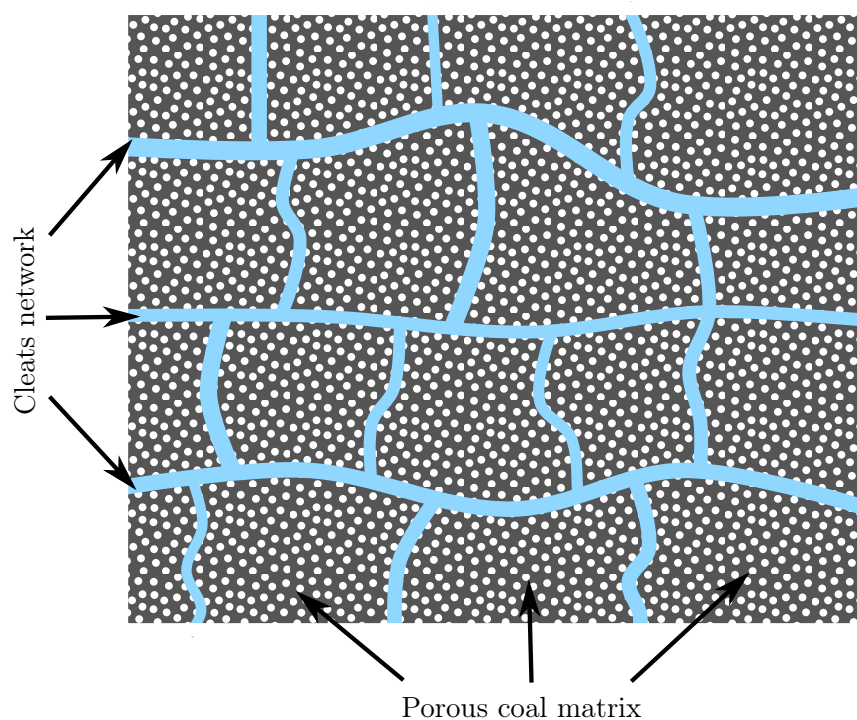
FIGURE 1.7. Schematic representation of a coal seam (Adapted from Harpalani and Schraufnagel (1990) ). Coal matrix is responsible for the differential swelling. The cleats network governs the transport properties of the seam.
