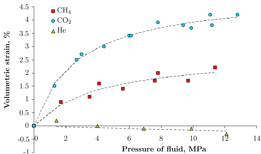
FIGURE 1.8. Volumetric strain of coal sample immersed in a pure fluid. The results are adapted from Ottiger et al. (2008) . The experiments are performed on dry coal samples from the Sulcis coal province (Italy).
