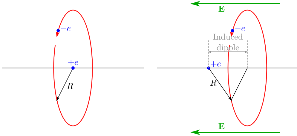
FIGURE 2.7. Sketch of an induced dipole in a one electron atom. Adapted from Israelachvili (1992) .
