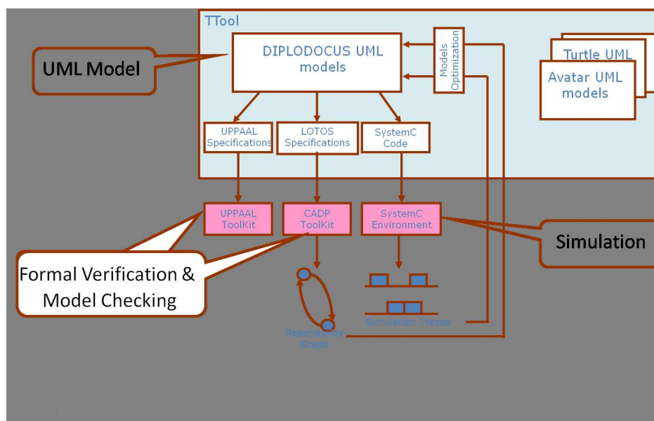
Figure 6.1: Simulation and formal verification with TTool
