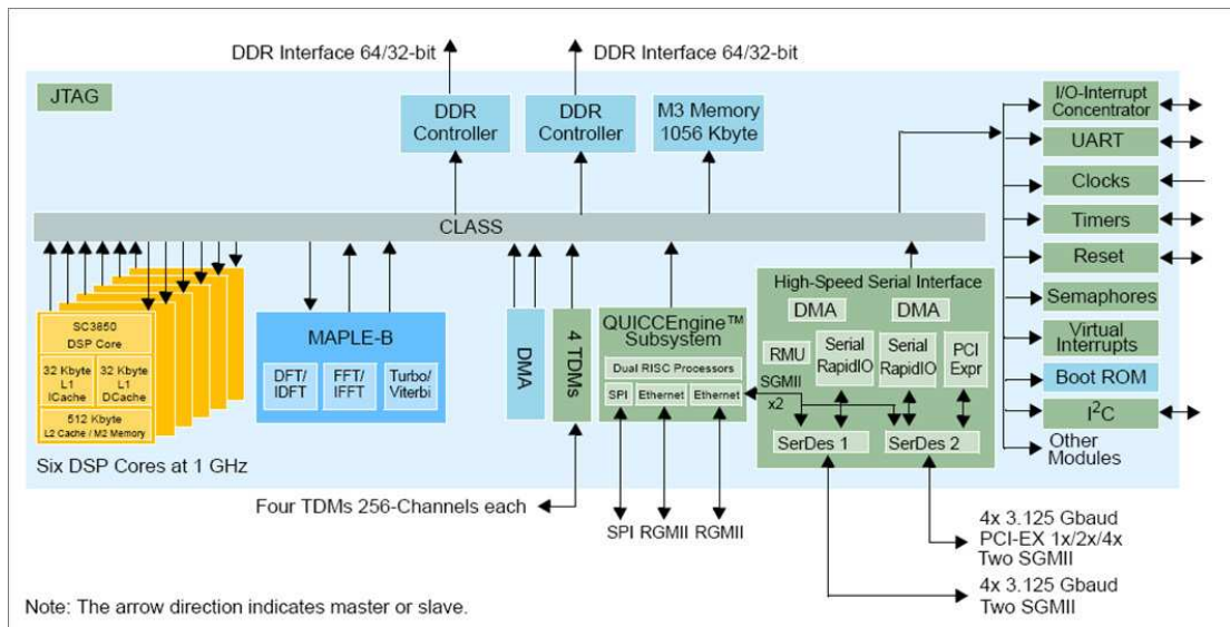
Figure 2.3: The Freescale DSP based SoC for LTE physical layer
