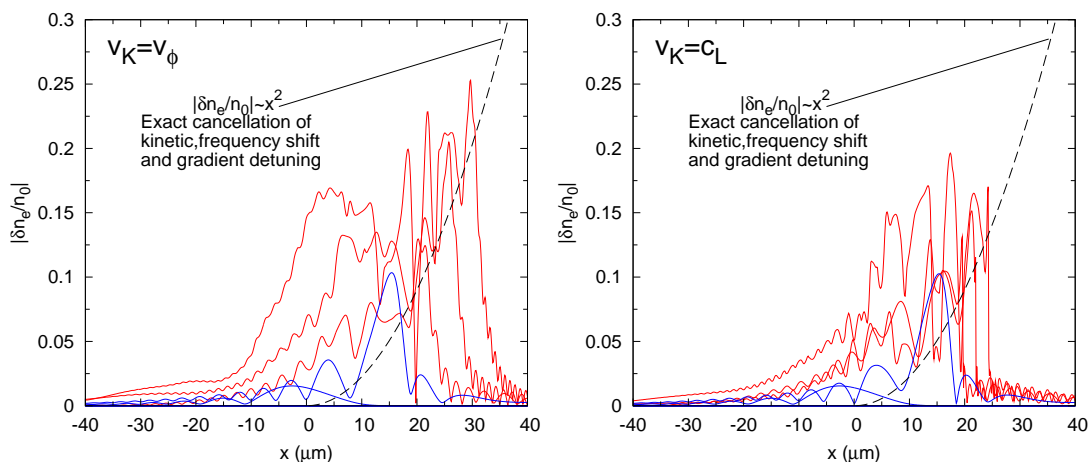
Figure 4.8: Langmuir wave envelope amplitude, obtained by solving the three wave equations. In both cases, the parameters are identical but for the velocity at which the kinetic nonlinear frequency shift propagates, v_K . (Left) Solution obtained for v_K = v_\phi . (Right) Solution obtained for v_K = c_L . In both cases, the blue lines indicate the initial response of the Langmuir wave to the passing of the pump wave. The red lines indicate the subsequent autoresonant evolution of the envelope amplitude. The interval between solutions is given by \Delta t = 0.2 ps, and both figures left and right show solutions in the range t = 0.3 - 1.1 ps.
