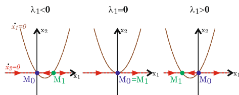
Fig. 2 Normal form reduction near \mu_c . The two nullclines \dot{x}_1 = 0 and \dot{x}_2 = 0 appear. Plain arrows indicate the direction of the trajectories for x_2 = 0
