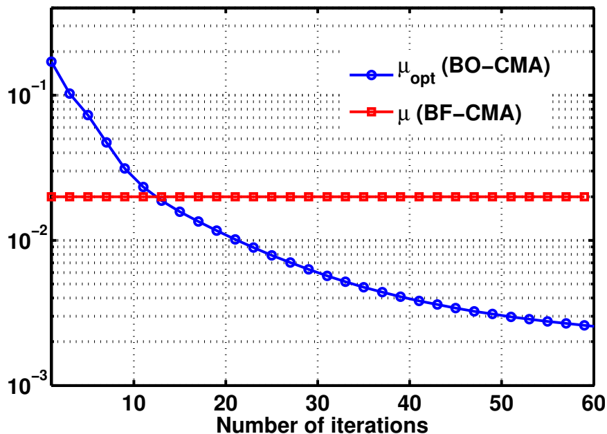
Figure 4.4: Optimal step size (BO-CMA) and fixed step-size (BF-CMA) versus the number of iterations ( N = 1000 , OSNR = 20dB, DL_f = 1000\text{ps/nm} , \tau_{\text{DGD}} = 50\text{ps} , \theta = \pi/4 ).
