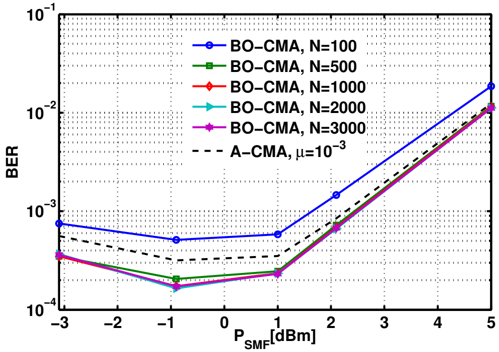
Figure 4.31: BER versus the power at the input of the SSMF for various N . (8PSK, residual CD of 1000ps/nm, transmission distance L_f = 800\text{km} .)
