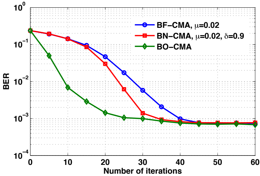
Figure 4.5: BER of the BO-CMA and the BF-CMA versus the number of iterations ( N = 1000 , \text{OSNR} = 20\text{dB} , DL_f = 1000\text{ps/nm} , \tau_{\text{DGD}} = 50\text{ps} , \theta = \pi/4 ).
