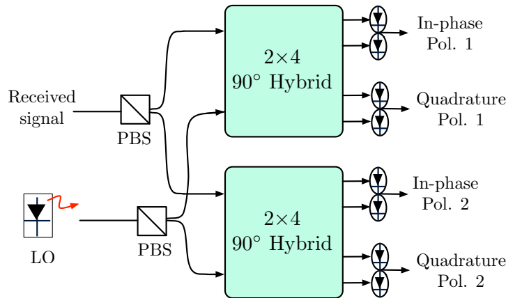
Figure 1.5: Block diagram of a phase and polarization diversity optical coherent receiver (POLMUX), LO and PSB stand for Local oscillator and Polarization Beam Splitter respectively
