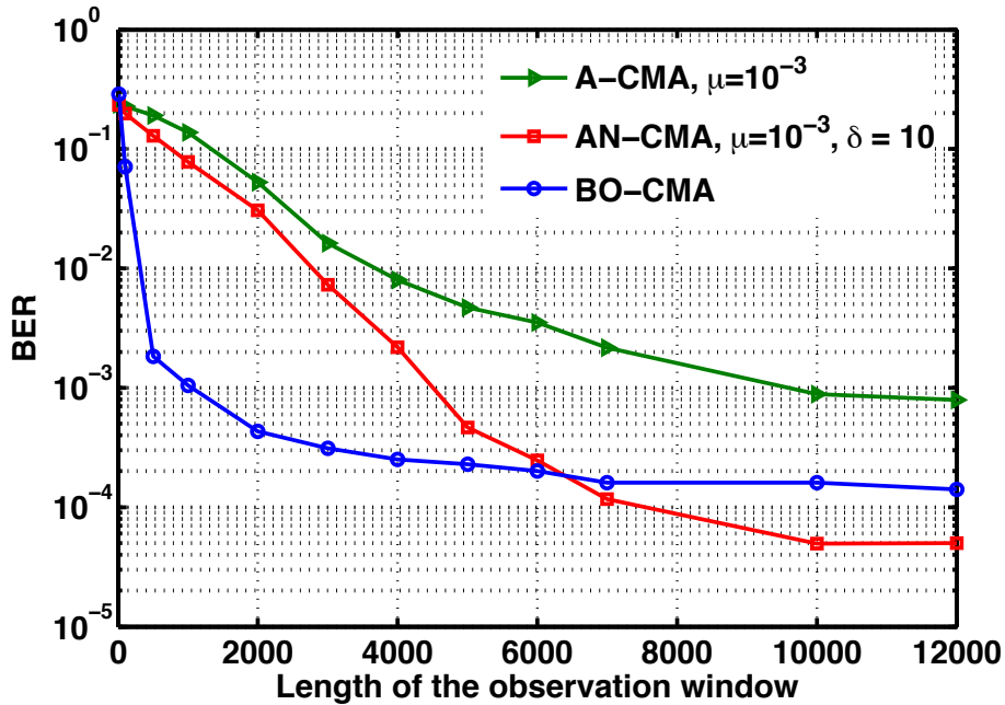
Figure 4.6: BER of the BO-CMA and the A-CMA versus the observation window length ( \text{OSNR} = 20\text{dB} , DL_f = 1000\text{ps/nm} , \tau_{\text{DGD}} = 50\text{ps} , \theta = \pi/4 ). For the BO-CMA, the observation window length is identical to the block size N . For the A-CMA, the observation window length is identical to the number of iterations.
