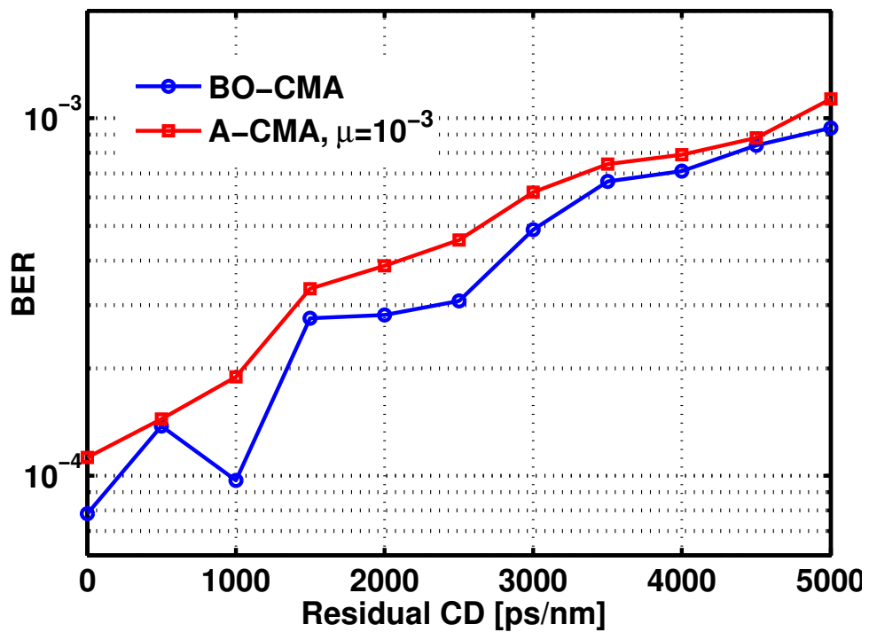
Figure 4.32: BER versus the residual CD (8PSK, OSNR=23.7dB, transmission distance L_f = 800\text{km} .)
