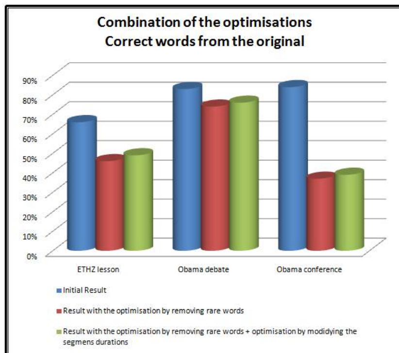
Figure 10.8: Speech-to-text algorithm - results of correct words from the original video after the optimization
