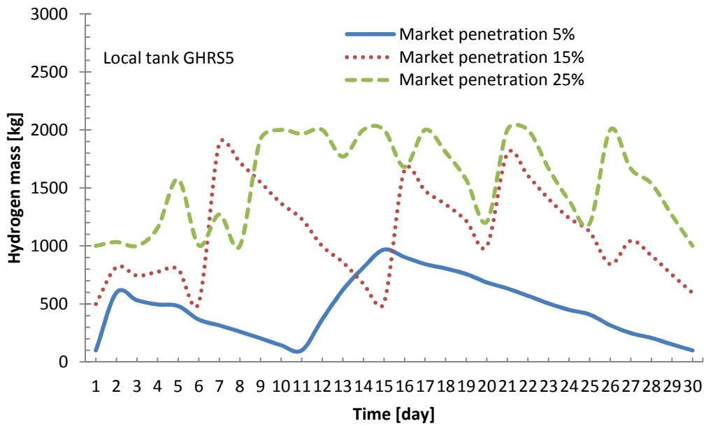
Figure 5.38 Hydrogen storage level of GHRS5
