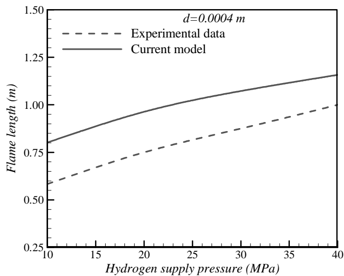
Figure 6.19 Comparison of the current model and experiments by T, Mogi and S, Horiguchi
