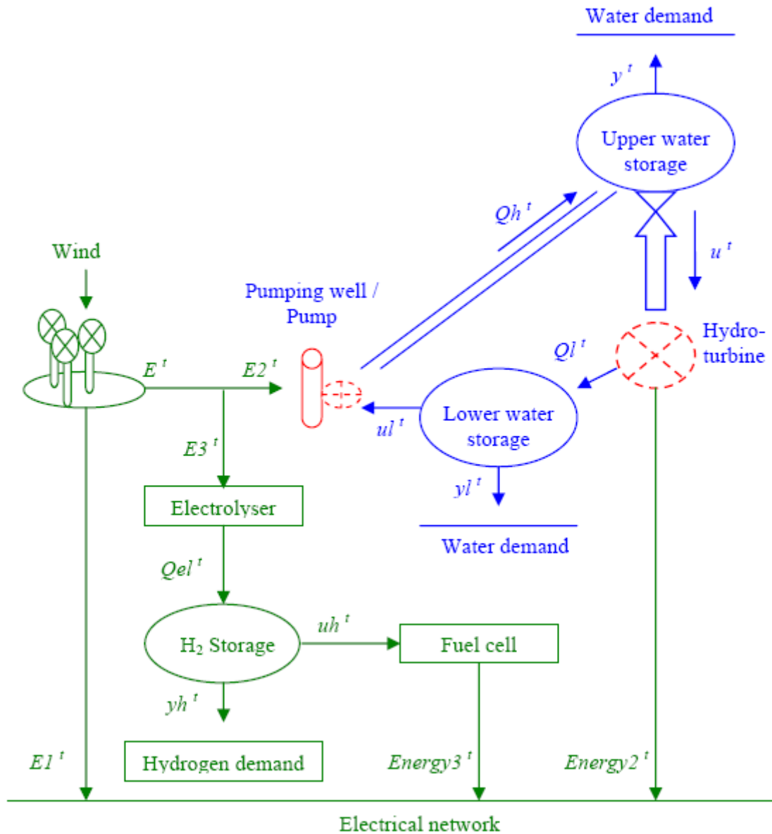
Figure 7.1 The integrated renewable energy system
