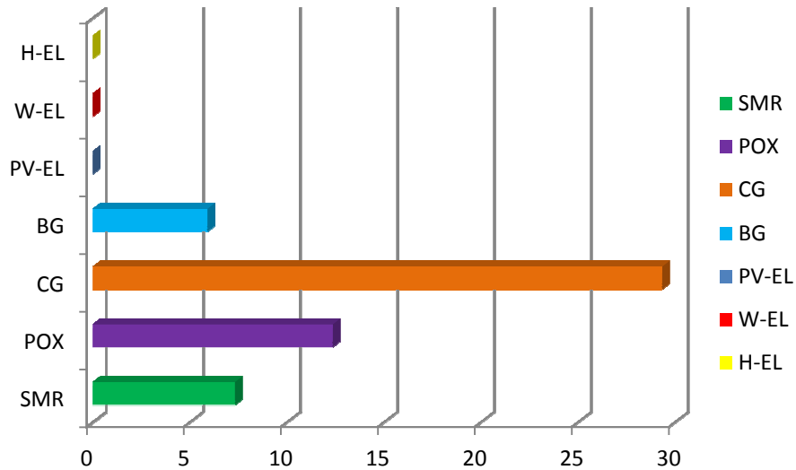
Figure 3.2 CO 2 emissions of various hydrogen production technologies (Pilavachi et al. , 2009)
