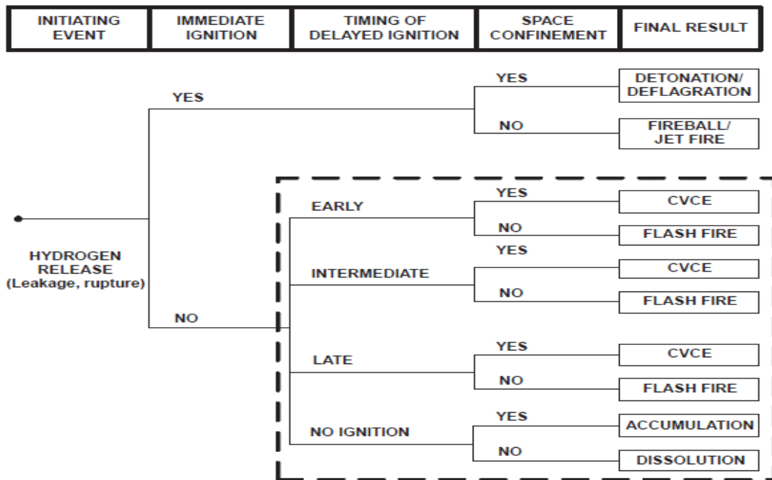
Figure 4.10 Event Tree Analysis adapted to accidental hydrogen releases (Rigas and Sklavounos,
