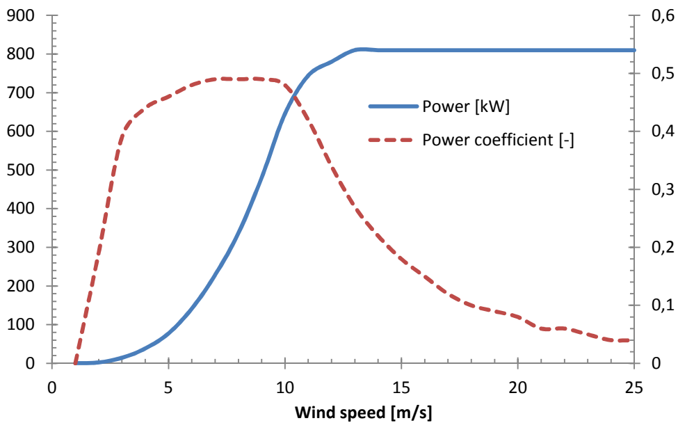
Figure 5.26 Manufacturer power curve of the considered wind turbine
