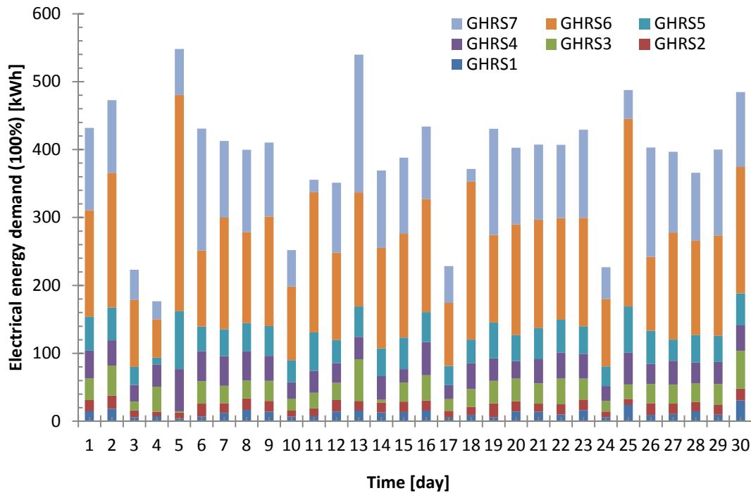
Figure 5.28 Electrical energy demand of the network of GHR5
