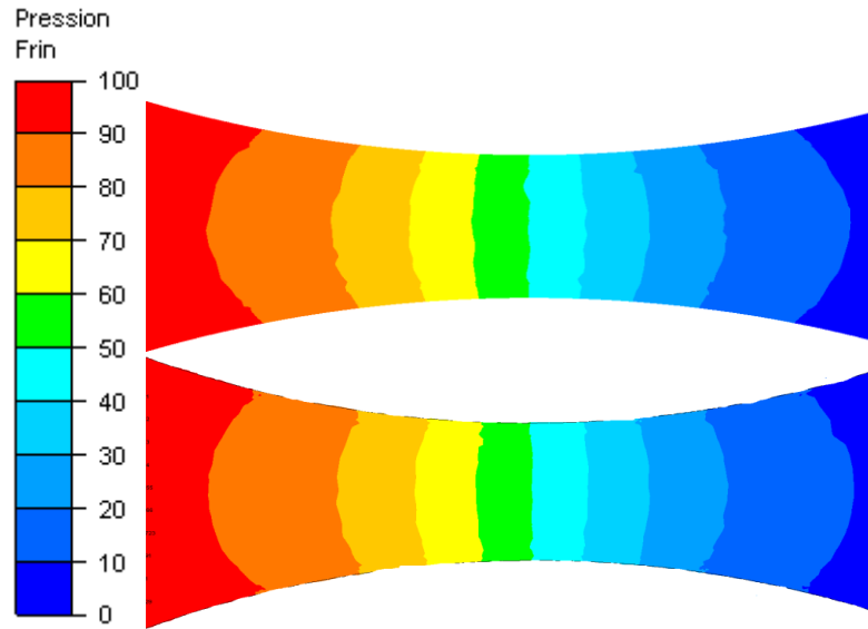
Figure 4-29: Pressure field comparison in the fluid between the monophasic (reference solution) and the multiphase approach after the modification of the bubble viscosity.
