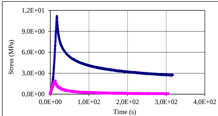
Figure 5-13: Relaxation tests. Comparison between 90°C (blue) and 110°C (pink).
