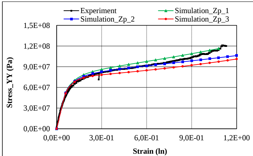
Figure 5-37: Stress evolution comparison between experiment and simulation with different values of Z_p .
