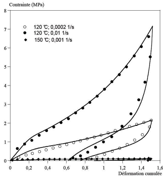
Figure 0-3 : Comparison model (plain line) – experience for PMMA [80].
