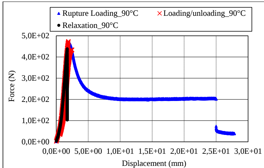
Figure 5-7: Experimental curve force/displacement at 90°C under different solicitations (loading up to rupture, loading/unloading and relaxation).
