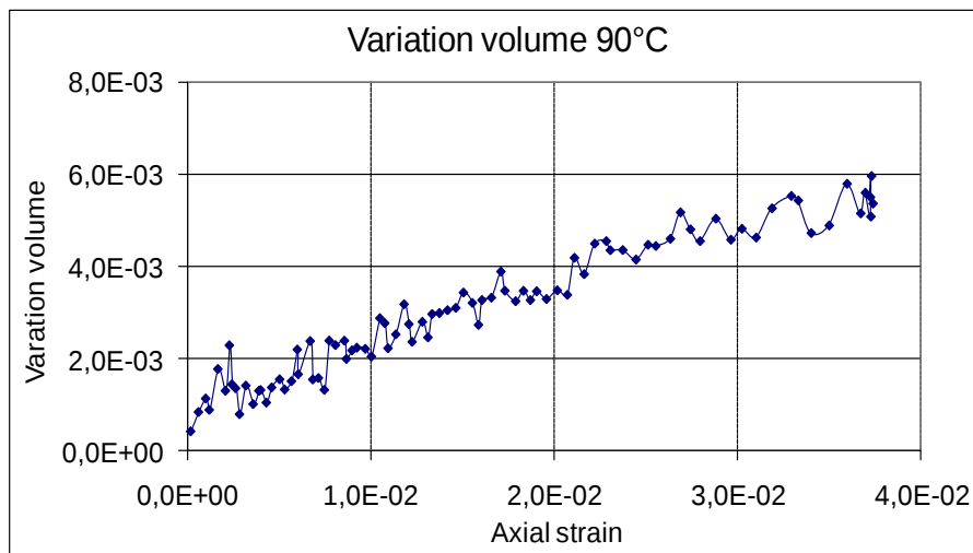
Figure 5-17: Volume variations at 90°C.
