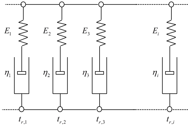
Figure 2-5: Generalized Maxwell model.
