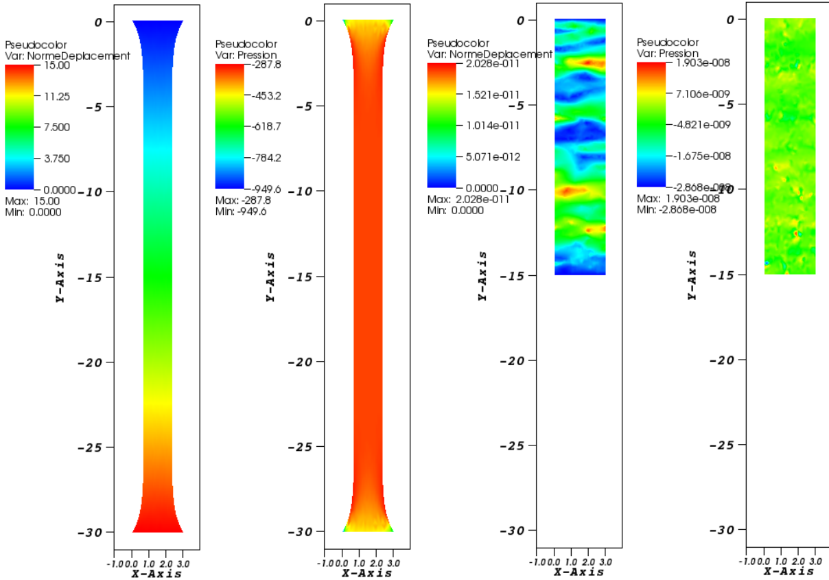
Figure 4-6: Displacement norm and pressure under loading-unloading with the new SMC solver. Errors in recovery are of the order of the asked precision for the iterative solver ( 1e^{-11} ) for the displacement norm and 1e^{-8} for pressure.
