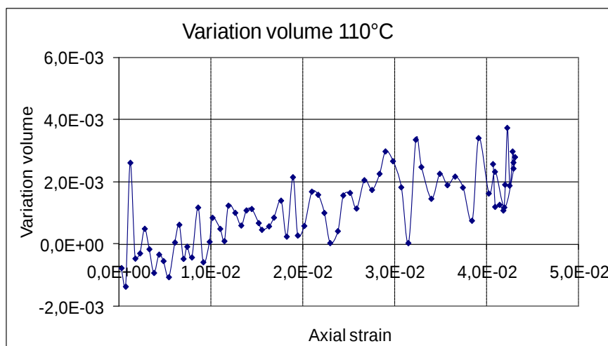
Figure 5-18: Volume variations at 110°C.
