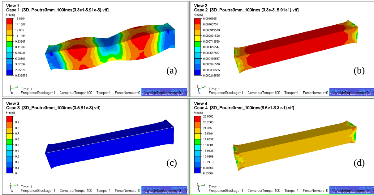
Figure 3-20: Elastic stress under uploading at 35% strain for 100 time steps in the viscoelastic case. (a, b, c, d) refer to the different cases of Table 3-1.
