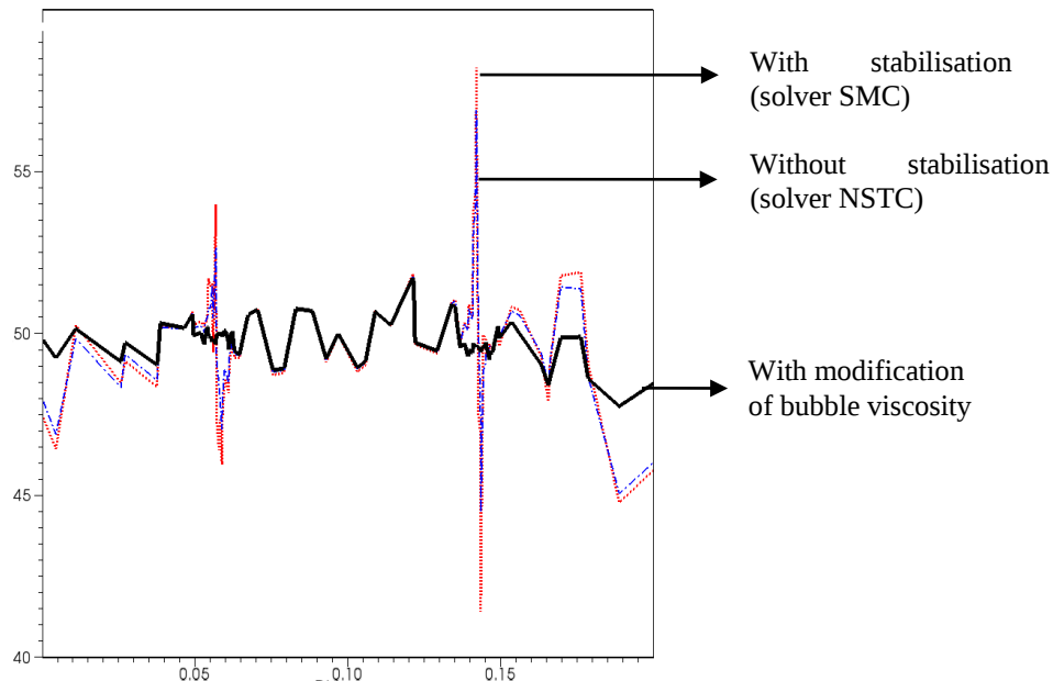
Figure 4-30: Pressure analysis through the thickness with different methods.
