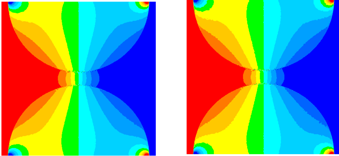
Figure 4-15: Pressure field resolution by the NSTC solver on the left and the SMC solver on the right.
