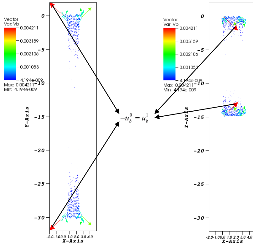
Figure 4-8: Bubble displacement under loading u_b^0 (left) and under unloading u_b^1 (right) with the full resolution by the new SMC solver. First, we can see the unstable pressure zone in the borders where the intensity of the bubble displacement is strong. Secondly, this shows a perfect recovery in which the obtained bubble displacements are perfectly opposite to traction and during spring back.
