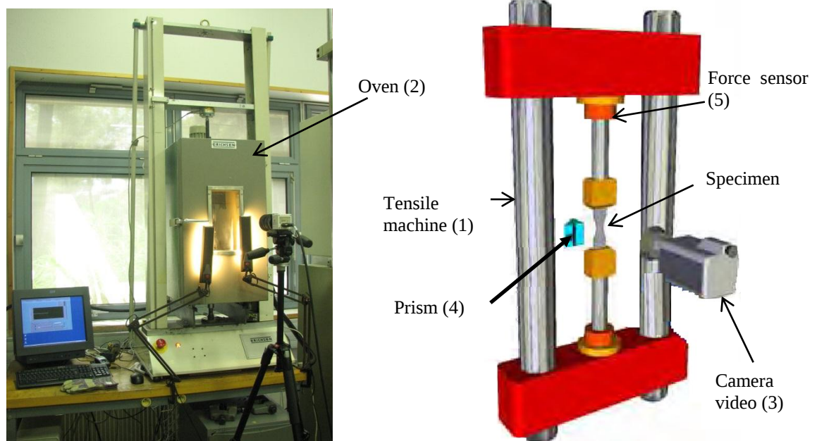
Figure 5-3: Test bench for 90°C and 110°C.
