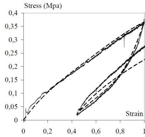
Figure 0-4: Comparison between experimental curve (plain line) and prediction of the model (dotted line) in the case of 10\text{e}^{-3}\text{ s}^{-1} tensile test at 115^{\circ}\text{C} [81].
