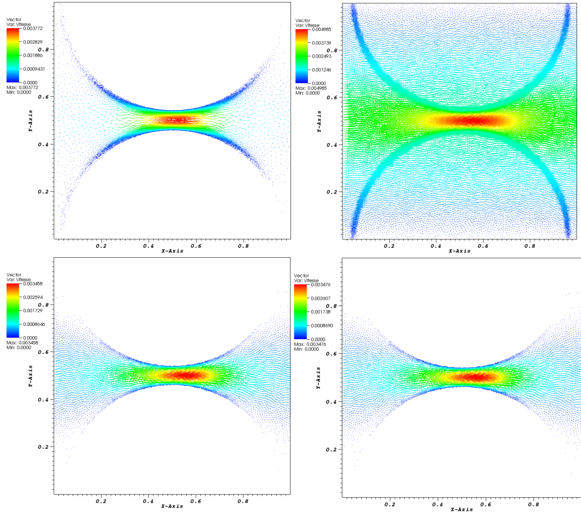
Figure 4-13: Velocity field (linear part) for the test case of flow around rigid particles. In the first row, on the left, velocity by the one phase modeling (reference results), on the right velocity by the penalization method; in the second row, on the left, velocity by the augmented Lagrangian method with Uzawa algorithm (the old solver NSTC) and on the right the new solver SMC (augmented Lagrangian method with Uzawa algorithm with a bubble's extra stress).
