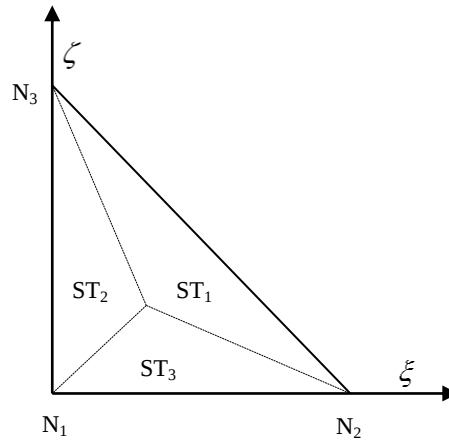
Figure 3-5: Schematic representation of a reference sub-element ( ST_i ) in two dimensions.
