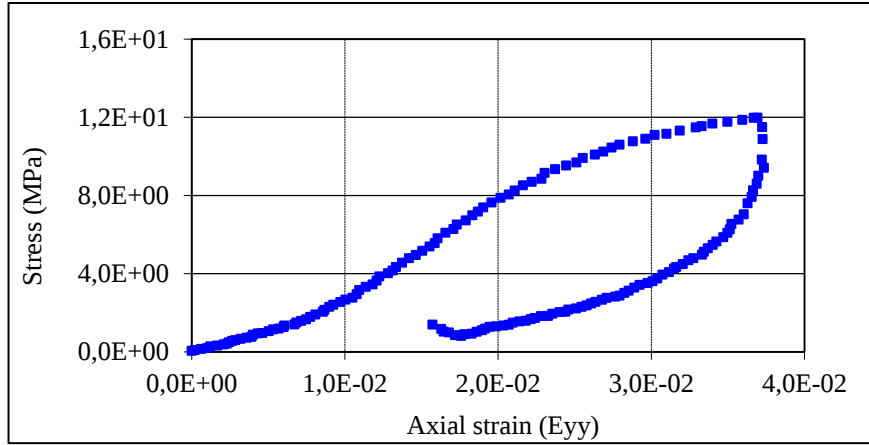
Figure 5-11: Non monotonic tensile tests (loading/unloading) at 90°C.
