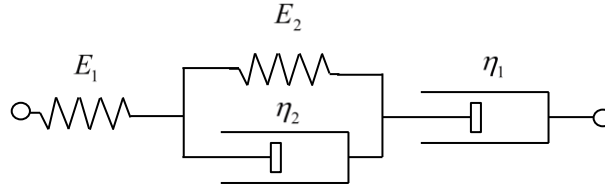
Figure 2-4: Schematic representation of the Burgers model.
