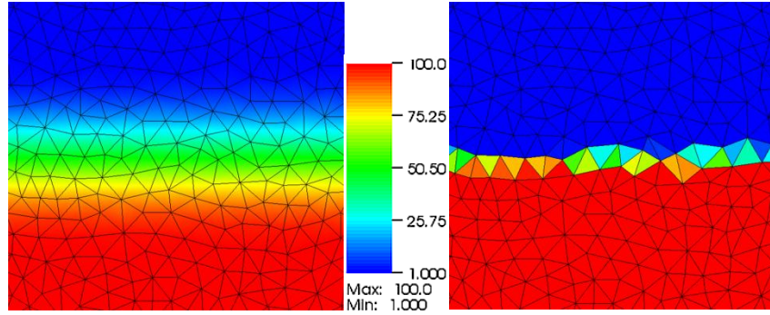
Figure 3-24: Illustration of the viscosity distribution on the mesh for the two mixture laws: P1 on the left and P0 on the right.
