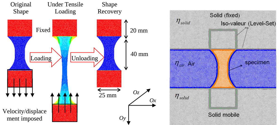
Figure 3-1: Simple uploading-unloading tensile test benchmark by the Lagrangian (left) and Eulerian (right) approach. In the left image, schematic of the original deformed and restored specimen. The image represents the initial, loaded and restored configurations. Remark that the specimen dimensions are in agreement with the real dimension of the specimen in the experimental test, which will be later presented in chapter 5. And the right image represents the schematic of the tensile test using an Eulerian method (detailed later in the section 3.4).
