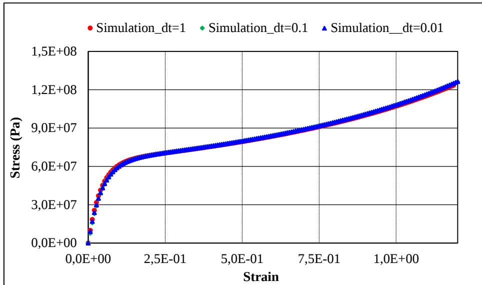
Figure 5-25: Stress vs. Strain curves for the tensile test at 21.6°C and for the strain rate of 1.83 \times 10^{-2} \text{ s}^{-1} . Curves illustrate the simulation with different time steps.
