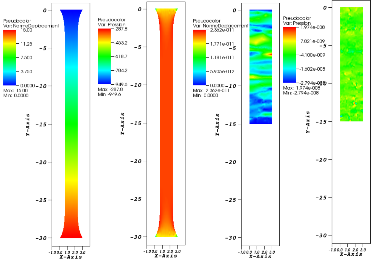
Figure 4-5: Displacement norm and pressure under loading-unloading with the old NSTC solver. Errors in recovery are of the order of the asked precision for the iterative solver ( 1e^{-11} ) for the displacement norm and 1e^{-8} for pressure.
