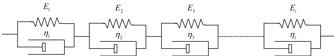
Figure 2-6: Generalized Kelvin-Voigt model.
