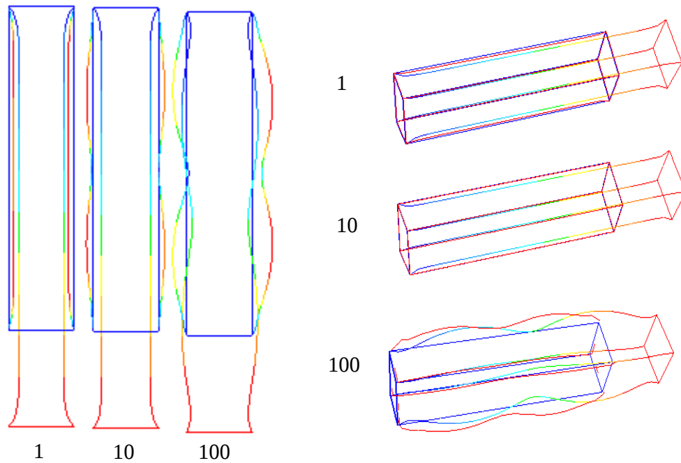
Figure 3-22: Specimen shape (2D-left image and 3D-right image) under tensile test at 35% strain for 1, 10 and 100 time steps in the elastic case.
