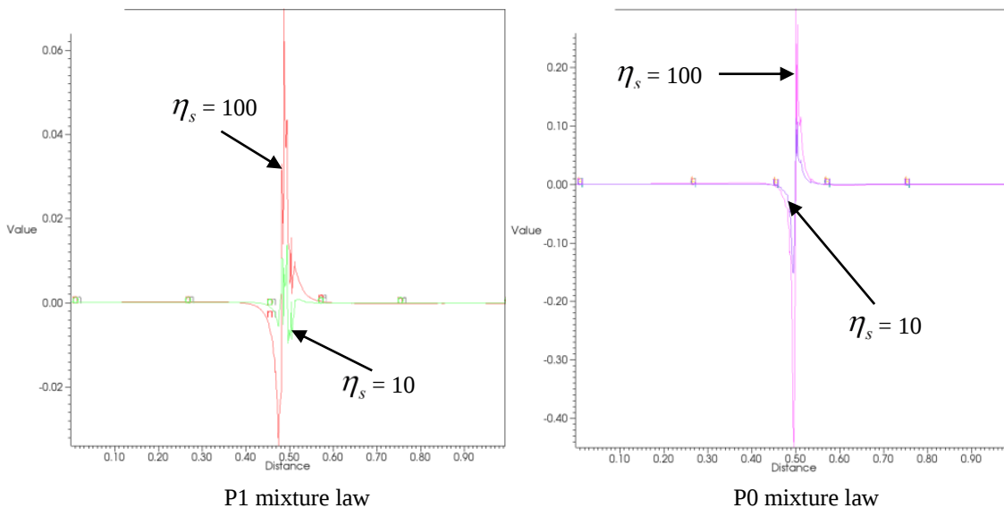
Figure 4-20: Pressure values through a vertical line crossing both domains for different solid viscosities using two different mixture laws. Please note that we did not synchronize the scales of the two curves due to the strong difference between them.
