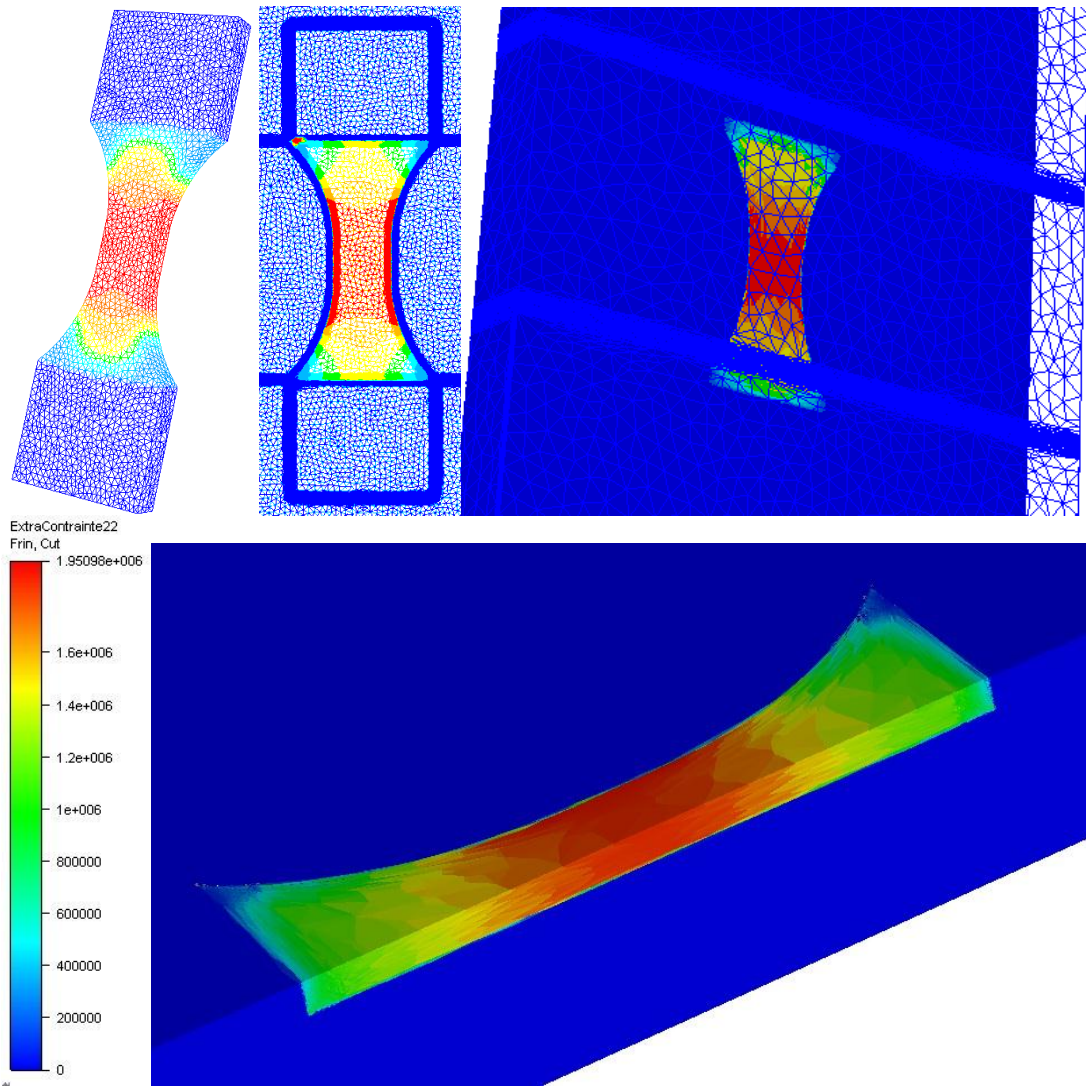
Figure 5-19: \sigma_{yy} stress at 110°C and loading by the incremental Lagrangian and Eulerian methods in 2D and 3D. In the first row, from left to right, the first image represents the specimen under loading by the incremental Lagrangian approach in 3D, the second describes the 2D Eulerian approach and the last one the 3D Eulerian approach. The image in the second row displays the stress inside of the specimen on two cutting planes, for the 3D Eulerian approach.
