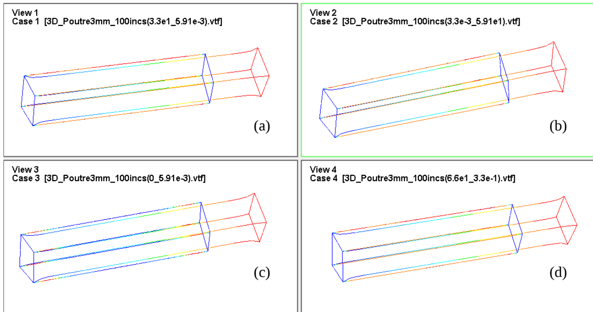
Figure 3-19: Specimen shape under uploading-unloading tensile at 30% strain for 100 time steps with different viscous and elastic factors. (a, b, c, d) correspond to the different cases of Table 3-1.
