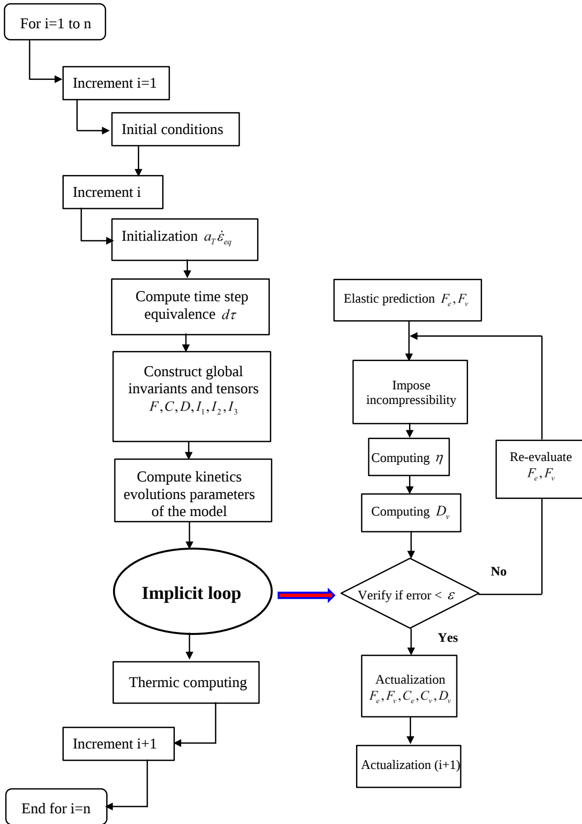
Figure 0-1: Algorithm of resolution
