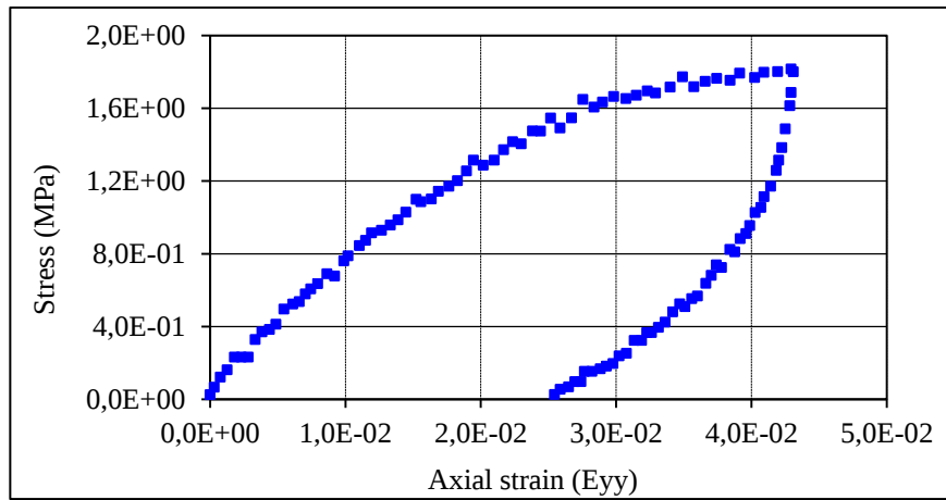
Figure 5-12: Non monotonic tensile tests (loading/unloading) at 110°C.
