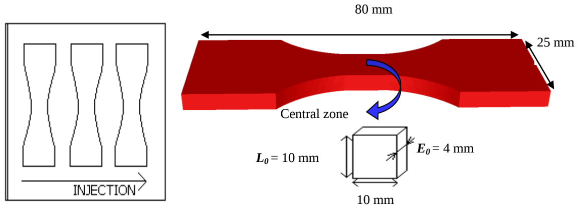
Figure 5-1: Samples tooled from the PMMA plate and its initial form.
