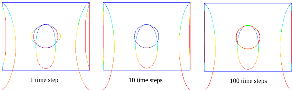
Figure 3-15: Specimen shape (2D with a circular hole) under uploading-unloading tensile at 30% strain for different time steps.
