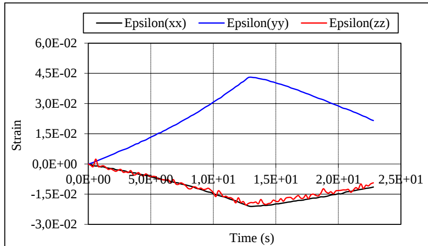
Figure 5-16: Comparison between the strain in the three directions at 110°C.
