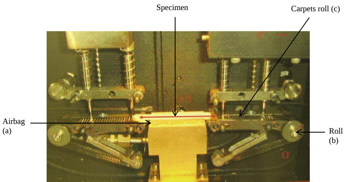
Figure 5-6: Test bench for 163°C.
