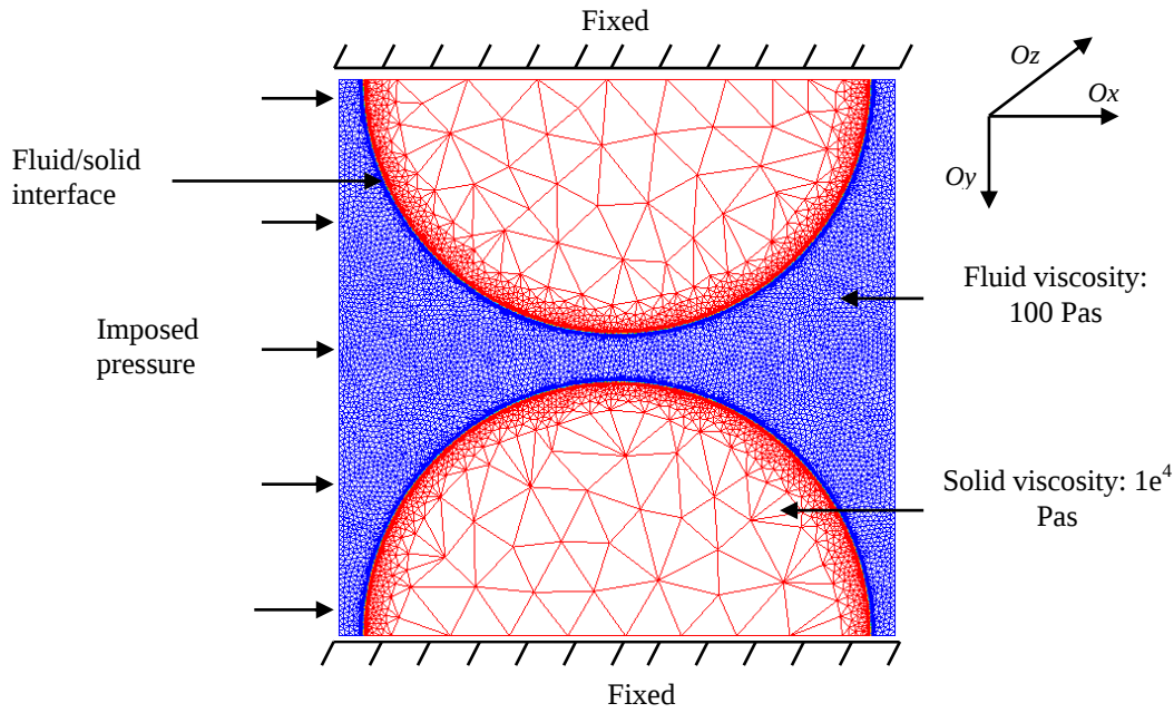
Figure 3-2: Geometry, boundary conditions and mesh representation for the flow between two rigid particles test case.
