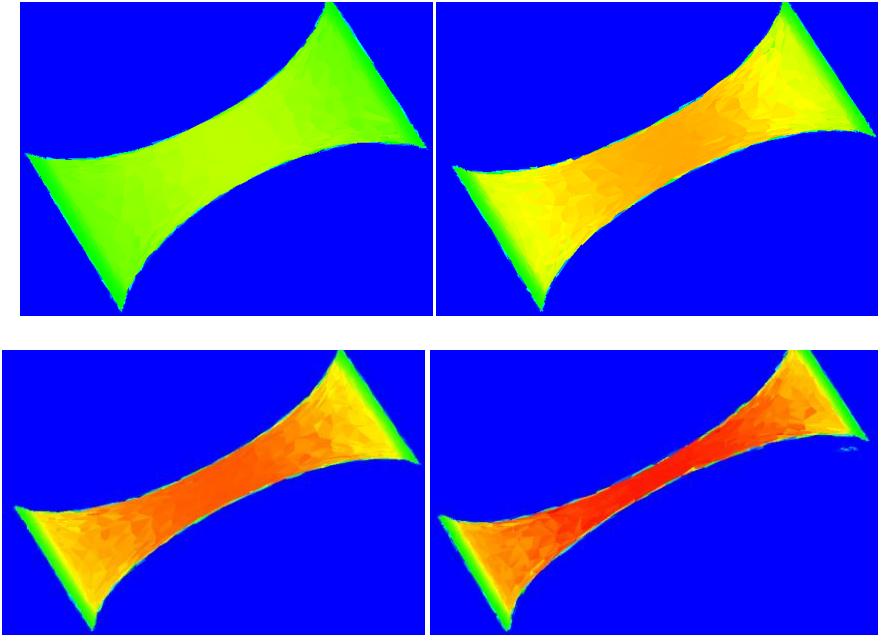
Figure 5-30: Longitudinal stress distribution at 5% (upper left), 15% (upper right), 25% (lower left) and 50% (lower right) of deformation.
