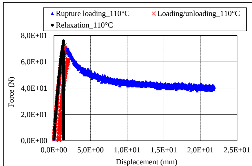
Figure 5-8: Experimental curves force/displacement at 110°C under different solicitations (loading up to rupture, loading/unloading and relaxation).
