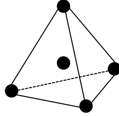
Figure 4-3: Displacement interpolation.
