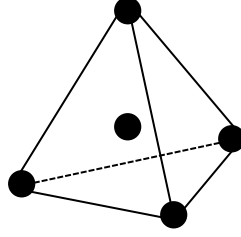
Figure 3-4: Displacement interpolation.
