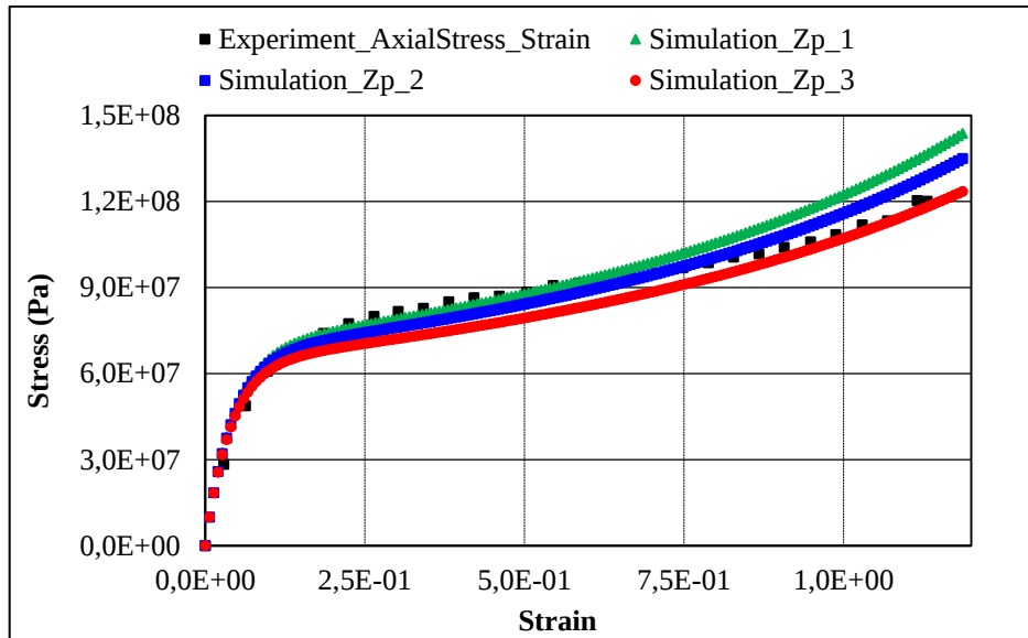
Figure 5-23: Stress vs. Strain curves for the tensile test at 21.6^{\circ}\text{C} and for a strain rate of 1.83\text{e}^{-2} \text{ s}^{-1} . The chosen material is a Polyamide 6.6 produced by Rhodia. Curves illustrate the comparison between experimental and simulation by calculation on the material point with different values of Z_p , the parameter that controls the change rate of \eta .
