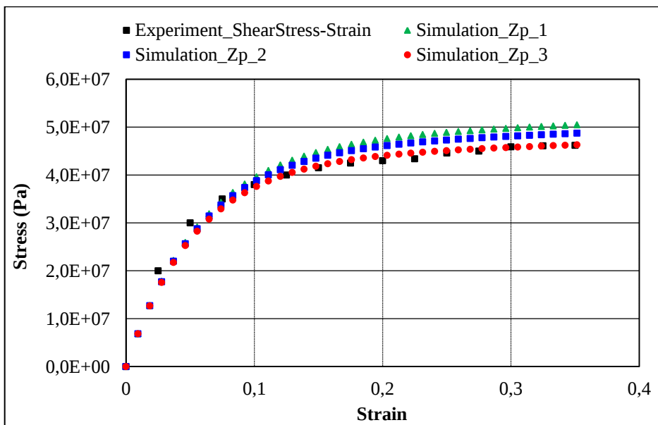
Figure 5-24: Stress vs. Strain curves for the shear test. Curves illustrate the comparison between experimental and simulation by calculation on the material point with different value of Z_p . The value of strain rate is 3.7\text{e}^{-2} \text{ s}^{-1} .
