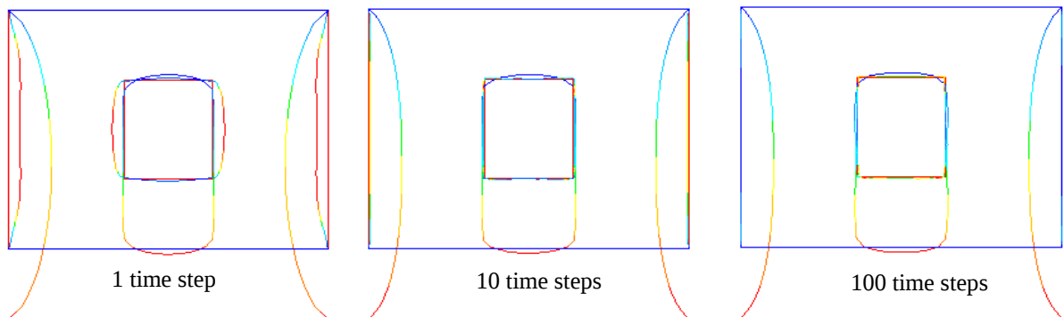
Figure 3-14: Specimen shape (2D with a rectangular hole) under uploading-unloading tensile at 30% strain for different time steps.
