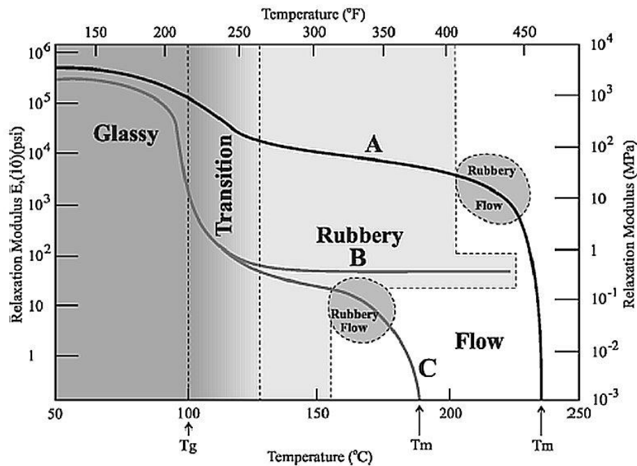
Figure 2-1: E_r(10 \text{ Sec.}) for a crystalline polystyrene (A), a lightly cross-linked polystyrene (B), and amorphous polystyrene (C) [15].
