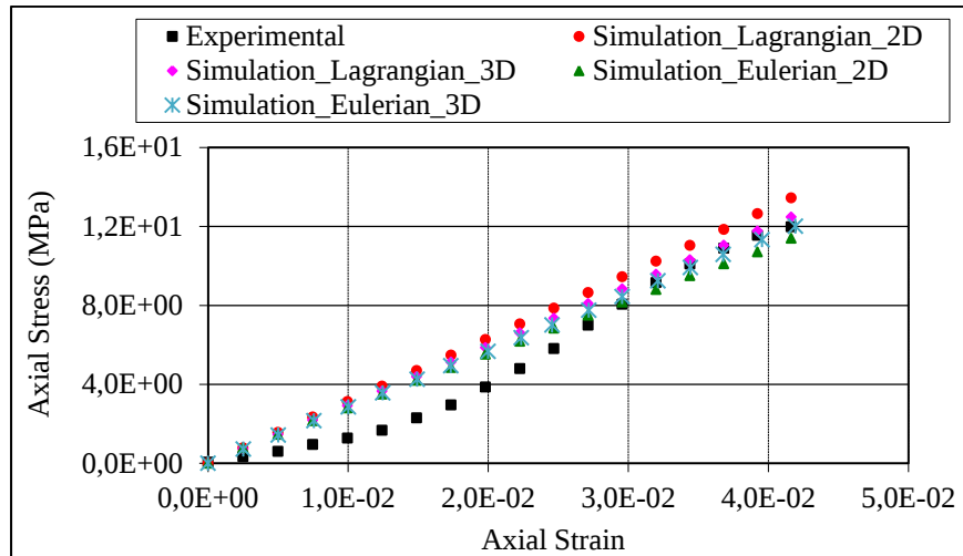
Figure 5-20: Stress vs. Strain curves for loading at 90°C. Curves illustrate the comparison between experimental and simulation by the incremental Lagrangian and Eulerian methods, in 2D and 3D.
