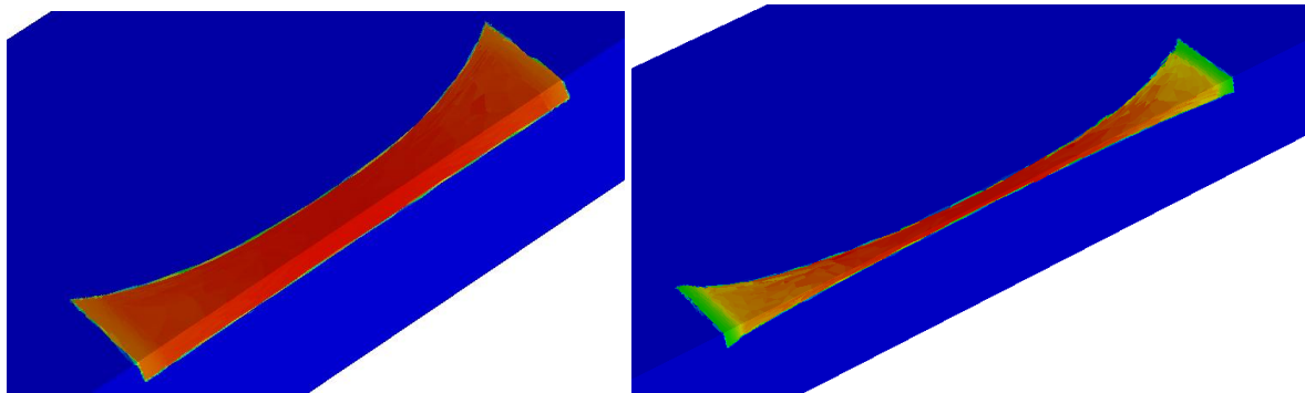
Figure 5-31: Longitudinal stress distribution inside the specimen at 5% (left) and 60% (right) of deformation. Schematic representation is obtained by two symmetric cutting planes following the longitudinal and the thickness direction.
