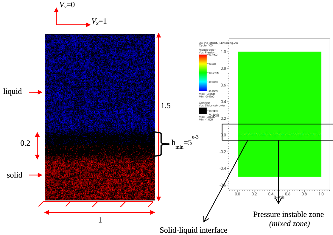
Figure 4-18: Two phase test case.
