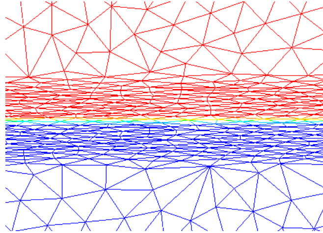
Figure 3-26: Interface refinement using anisotropic mesh adaptation: a zoom at the interface region.
