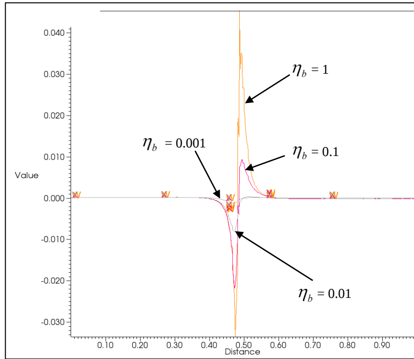
Figure 4-21: Pressure for different bubble viscosities, from 0.001 to 1 Pas by P1 mixture law.
