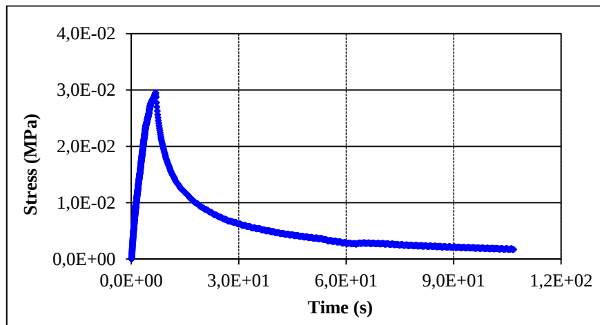
Figure 5-14: Relaxation tests at 163°C.
