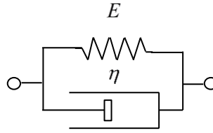
Figure 2-3: Schematic representation of the Kelvin–Voigt model.
