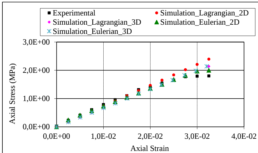
Figure 5-21: Stress vs. Strain curves for loading at 110°C. Curves illustrate the comparison between experimental and simulation by the incremental Lagrangian and Eulerian methods, in 2D and 3D.
