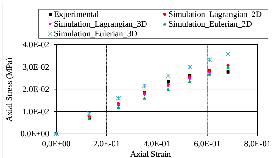
Figure 5-22: Stress vs. Strain curves for loading at 163°C. Curves illustrate the comparison between experimental and simulation by the incremental Lagrangian and Eulerian methods, in 2D and 3D.
