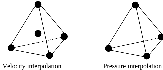
Figure 3-3: Element P1+/P1 (MINI-element) for velocity-pressure interpolation.
