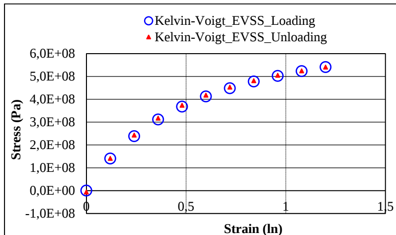
Figure 5-27: Axial stress in the central zone under loading and unloading.
