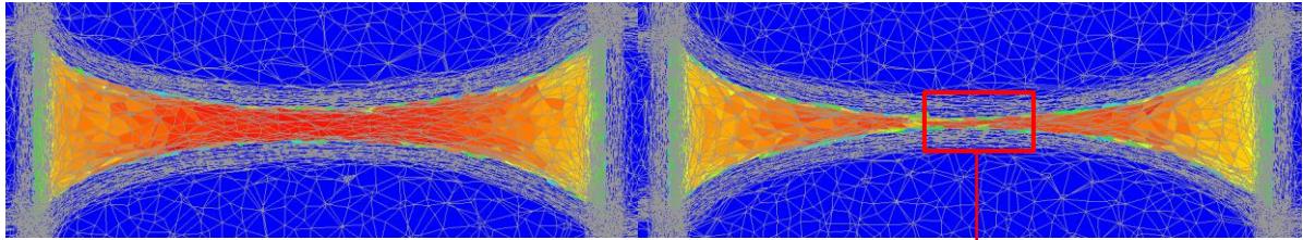
Figure 5-33: Anisotropic mesh and stress distribution on the cutting plan at 60% (left) and 70% (right).
