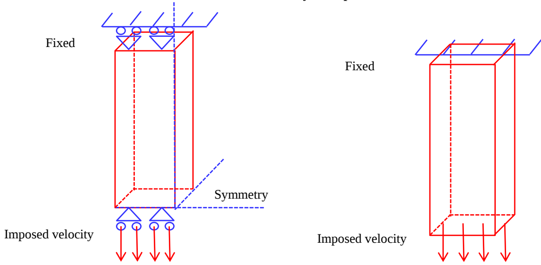
Figure 5-36: A perfect tensile test bench (left) and a normal tensile test bench (right).
