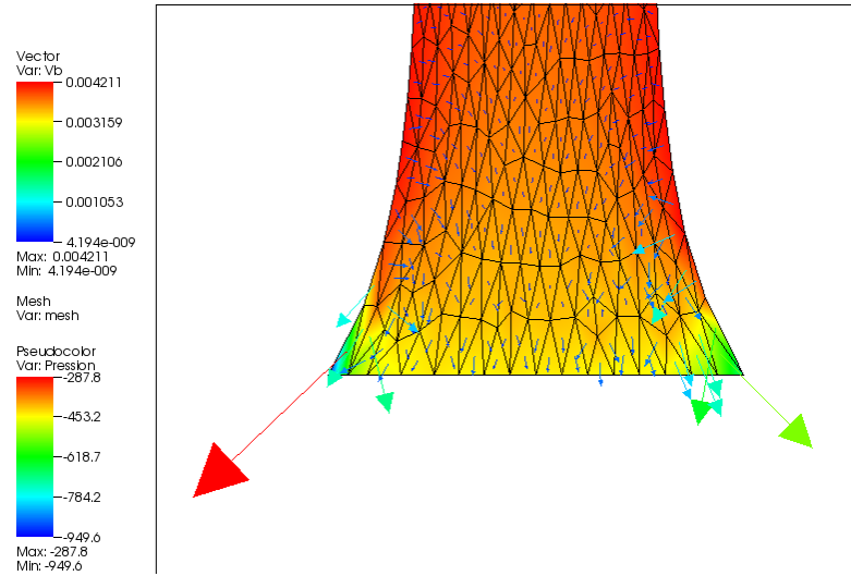
Figure 4-7: Schematic representation of the bubble velocity field in the specimen under loading with the mesh geometry and the pressure field. Since the bubble velocity is computed on elements, these vectors are illustrated on elements. Note that the pressure field is colored as its displayed scale.
