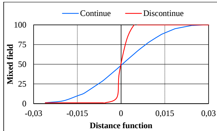
Figure 3-25: Vertical section of Figure 3-24. A good intermediate value of the mixed field for the discontinuous law is corresponding to that in the element crossed by the interface. The two variations of slope for the continue law P1 are due to the mesh.
