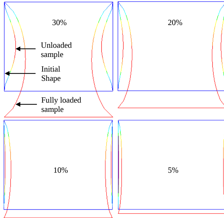
Figure 3-7: Specimen shape under uploading and unloading tensile tests with different levels of strain, for an elastic behavior and resolution on one single step.
