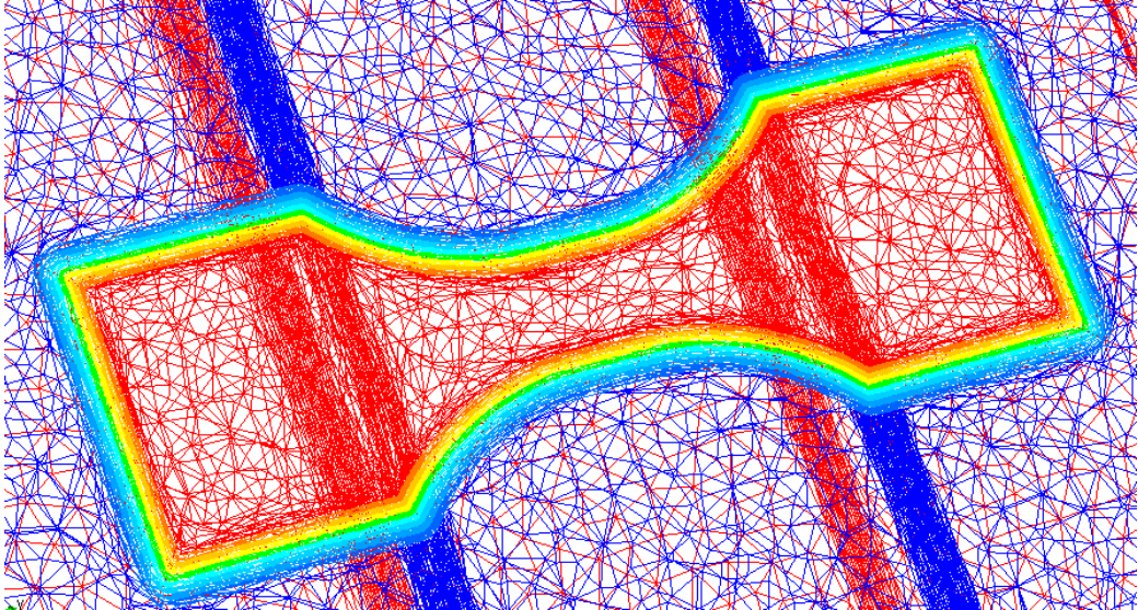
Figure 5-29: Original geometry and mesh of the tensile test by an Eulerian approach. Schematic representation of the mesh in a cutting plane on the thickness of the computational domain.
