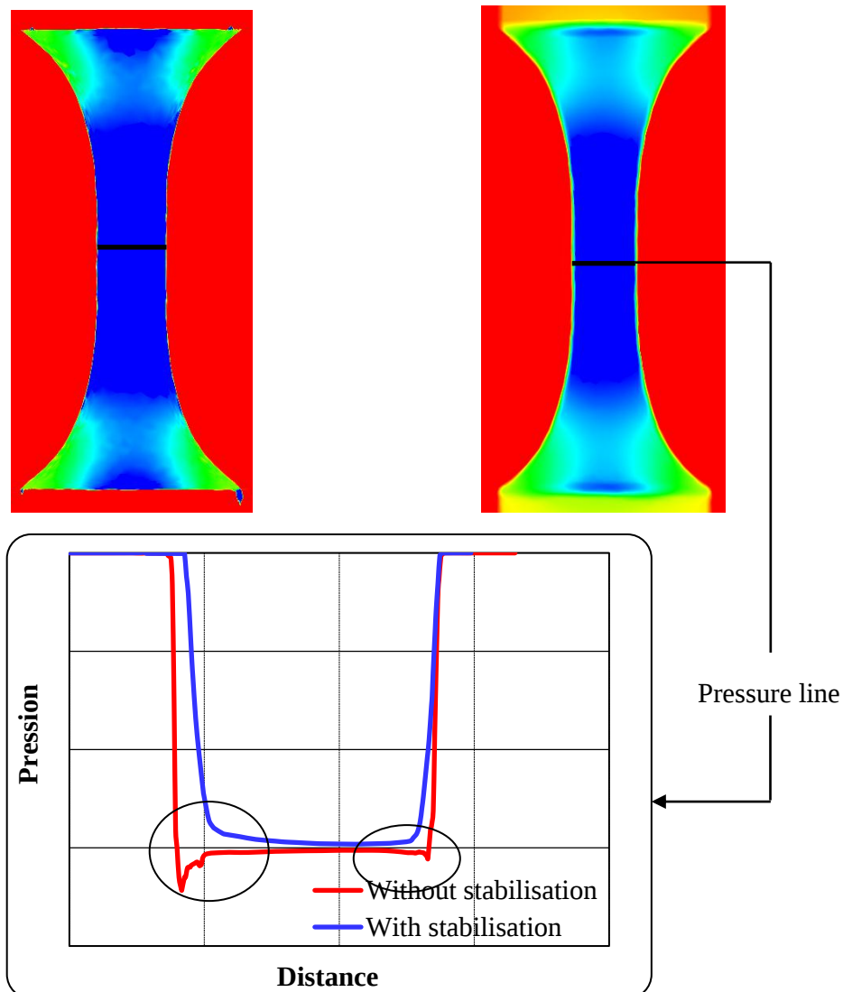
Figure 4-34: Pressure curve without stabilization (red - without modification of the bubble viscosity – left image) and with stabilization (blue - with modification of the bubble viscosity – right image).
