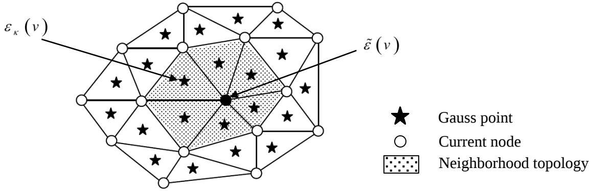
Figure 4-17: Stress projection on node [127].
