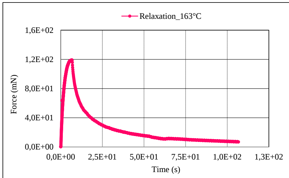
Figure 5-9: Experimental curve force/displacement at 163°C under a relaxation test.
