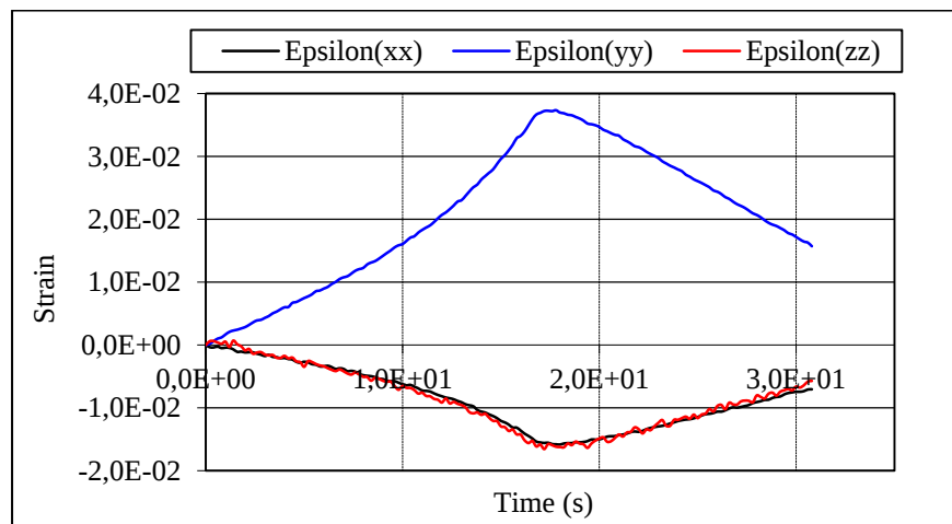
Figure 5-15: Comparison between the strain in the three directions at 90°C.
